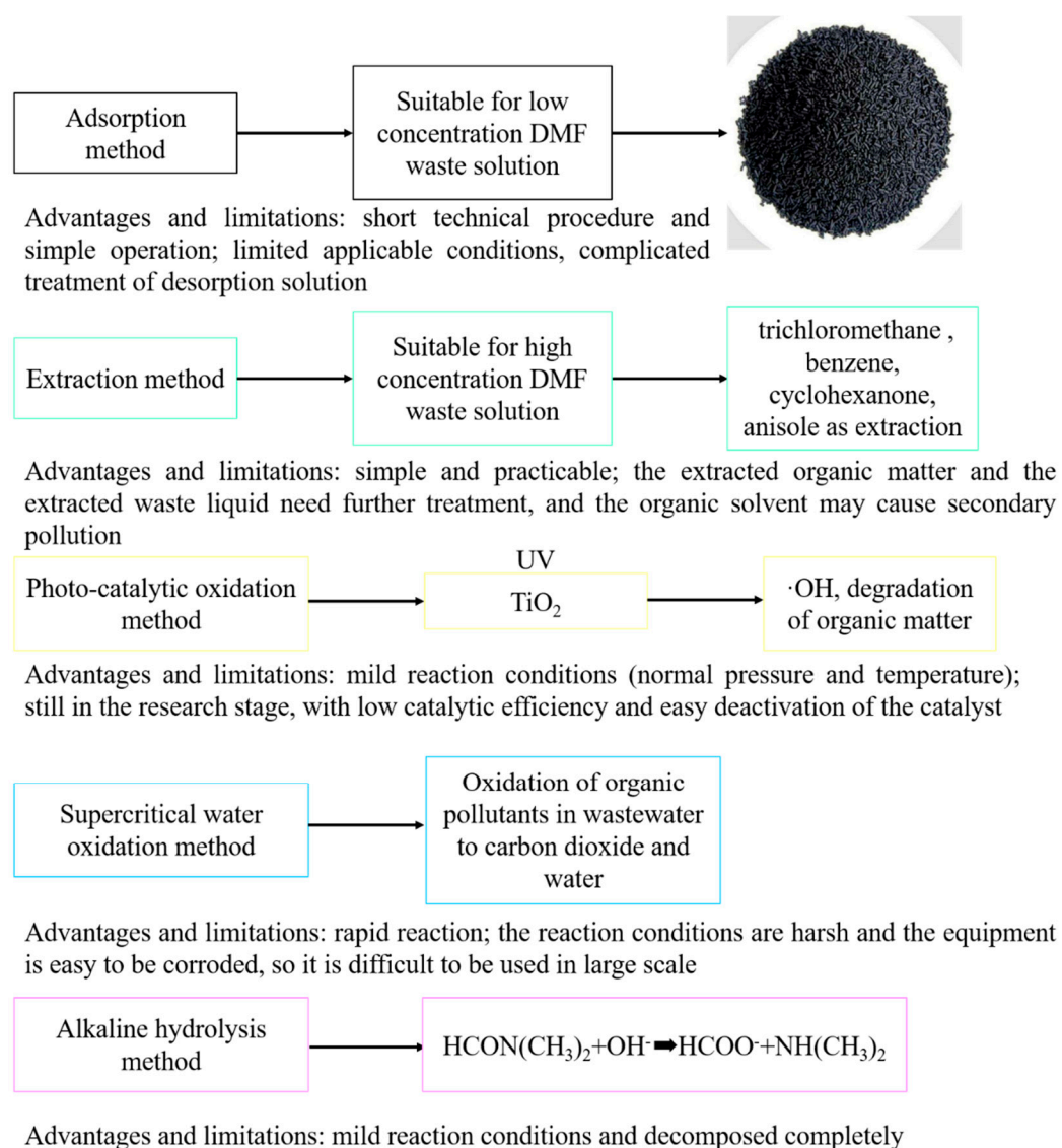
Figure 1. Some existing technologies used for DMF separation and their relative advantages and drawbacks.
