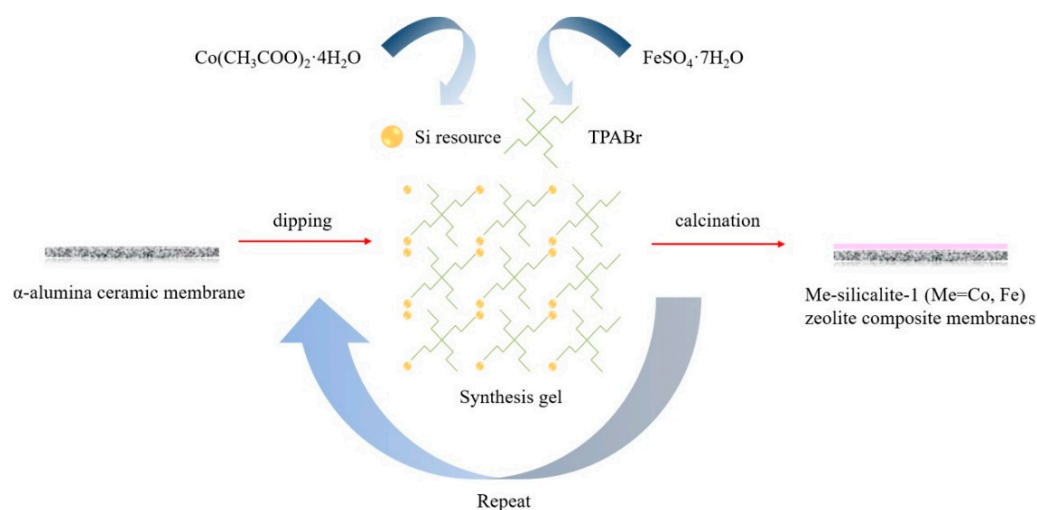
Figure 8. Fabrication procedures of the Me-silicalite-1 (Me = Co and Fe) zeolite composite membranes.
