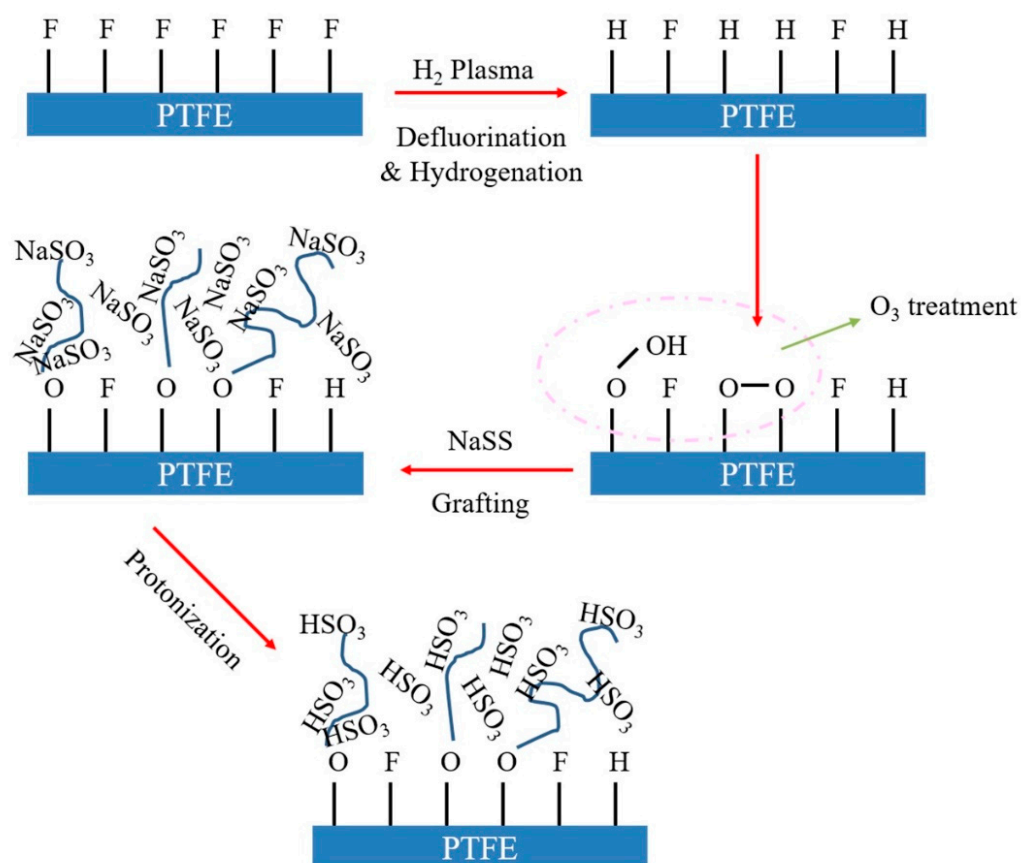
Figure 6. Fabrication procedures of the PTFE-g-PSSA membranes.
