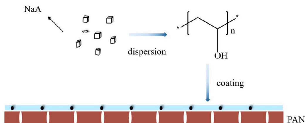
Figure 7. Fabrication procedures of the NaA/PAN membranes.
