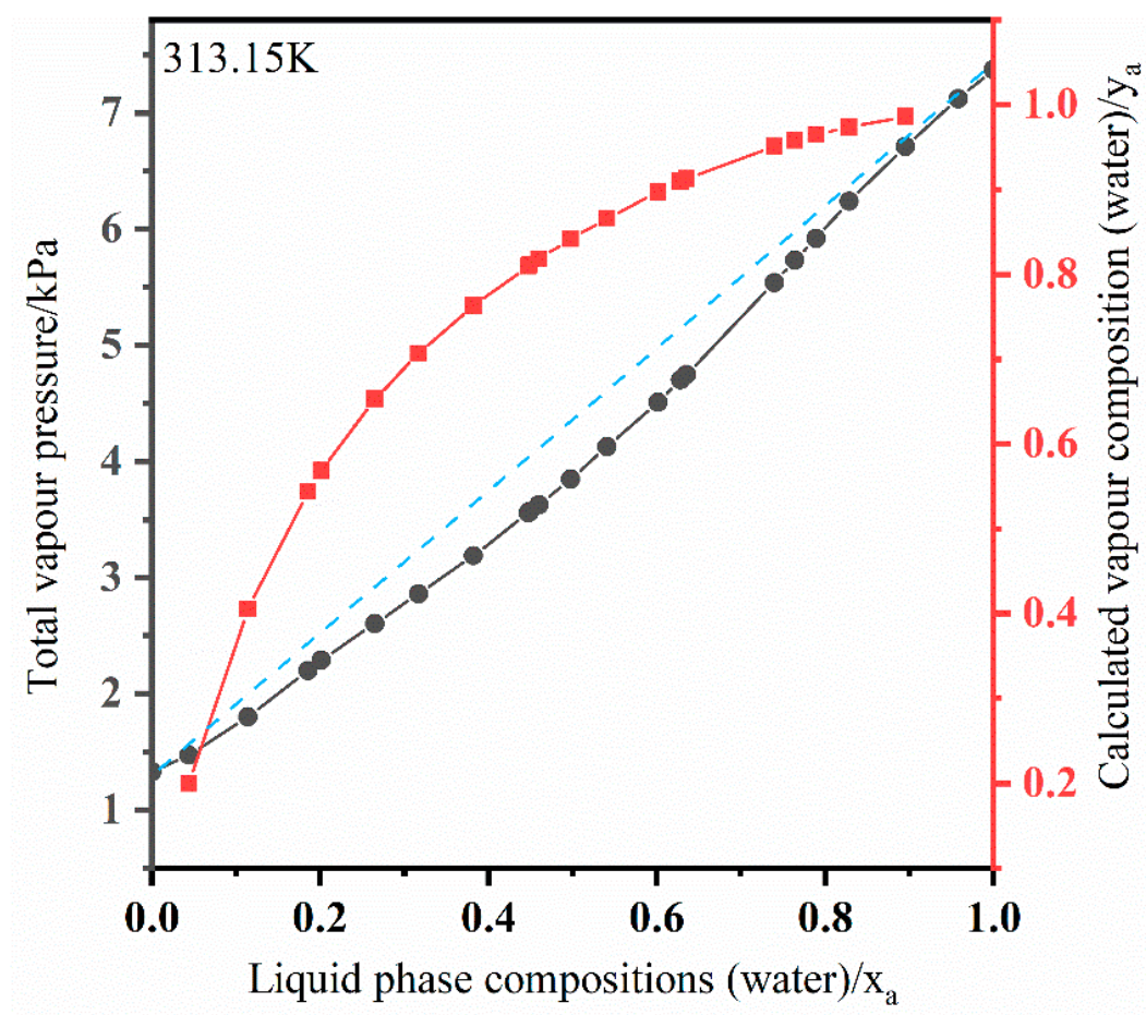
Figure 5. Vapor–liquid equilibria of DMF + water as a function of mole fraction of water.
