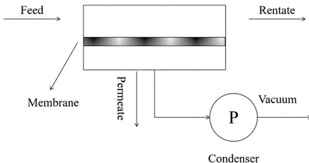
Figure 2. Graphical presentation of typical vacuum pervaporation process.
