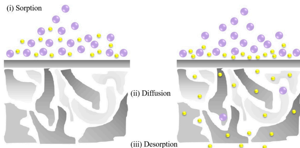
Figure 3. Graphical presentation of the solution–diffusion model.
