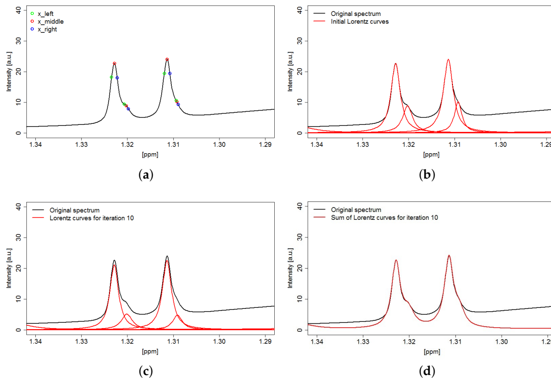
Figure 8. Deconvolution of the frequency region of the overlapping methyl groups of lactate and threonine in a 1D ^1\text{H} spectrum of human blood plasma. (a) Peak selection procedure to find the metabolite positions, (b) determination of initial Lorentz curves for parameter approximation, (c) iterative approximation of Lorentz curves, showing results after 10 iterations and (d) superposition of final Lorentz curves to match experimental spectrum.
