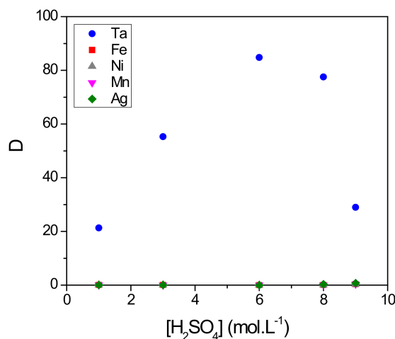
Figure 6. Effect of \text{H}_2\text{SO}_4 concentration on the distribution coefficient D of Ta, Fe, Ni, Mn and Ag. Extraction conditions: A/O = 1; T = 22^\circ\text{C} . Extraction time: 30 min. Organic phase (O): 4-MAcPh; Aqueous phase (A): [\text{Ta}] = [\text{Fe}] = [\text{Ni}] = [\text{Mn}] = [\text{Ag}] = 0.1 \text{ g}\cdot\text{L}^{-1} , [\text{H}_2\text{SO}_4] = 1\text{--}9 \text{ M} , [\text{HF}] = 0.06 \text{ M} .
