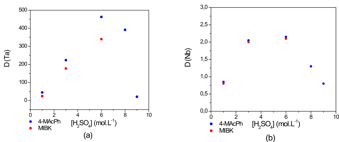
Figure 3. Effect of H 2 SO 4 concentration on the distribution coefficient D of (a) Ta and (b) Nb. Extraction conditions: O/A = 1; T = 22 °C. Extraction time: 30 min. Organic phase (O): 4-MAcPh (●) or methyl isobutyl ketone (MIBK) (●); Aqueous phase (A): [Ta] = [Nb] = 1 g·L −1 , [H 2 SO 4 ] = 1–9 M, [HF] = 0.06 M.
