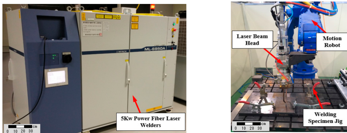
(b) Optical system and jig shape assembled in a six-axis robot.
