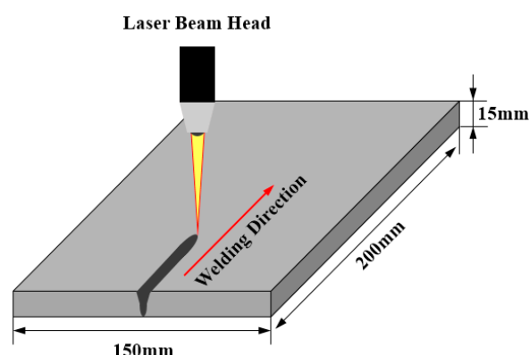
Figure 2. The fiber laser welding process.
