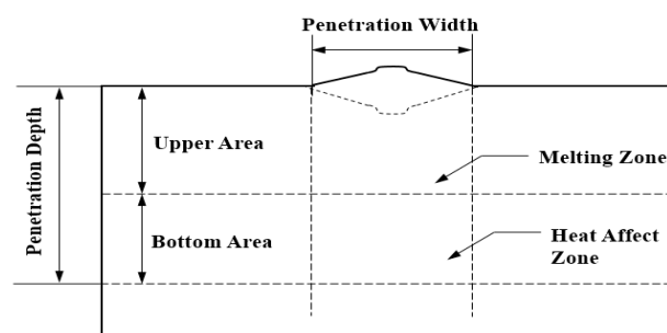
Figure 3. Schematic diagram of penetration geometry.
