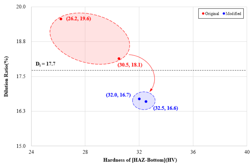
Figure 11. Weld joint hardening distributions using modified input parameters.
