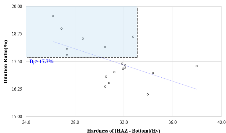
Figure 7. Weld joint hardening according to dilution ratio in fiber laser welding.
