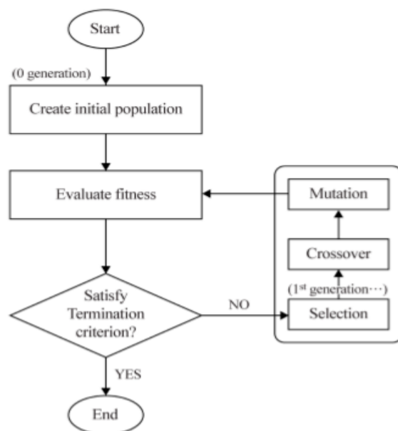
Figure 10. Flow chart of the multi-objective optimization (MOO) method to predict the welding parameters.
