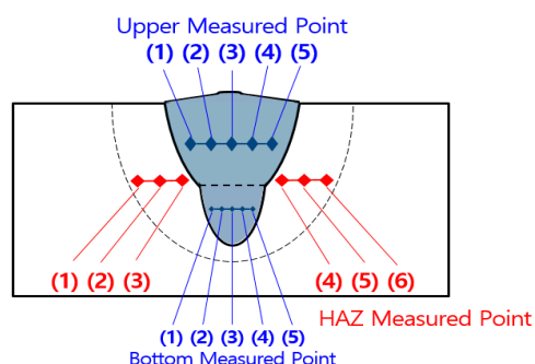
Figure 4. Schematic diagram of the hardness test.
