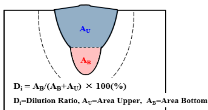
Figure 5. Schematic diagram of dilution ratio.
