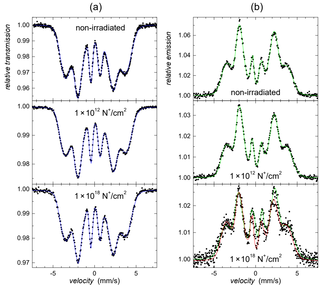
Figure 6. Mössbauer spectra of Fe_{74}Cu_{11}Nb_3Si_{16}B_6 amorphous metallic alloy irradiated by 110 keV N^+ ions with the indicated fluences: (a) transmission geometry (blue); (b) CEMS (green). Mössbauer spectrum taken from the wheel side of the ribbons is shown for comparison in (b) (red).
