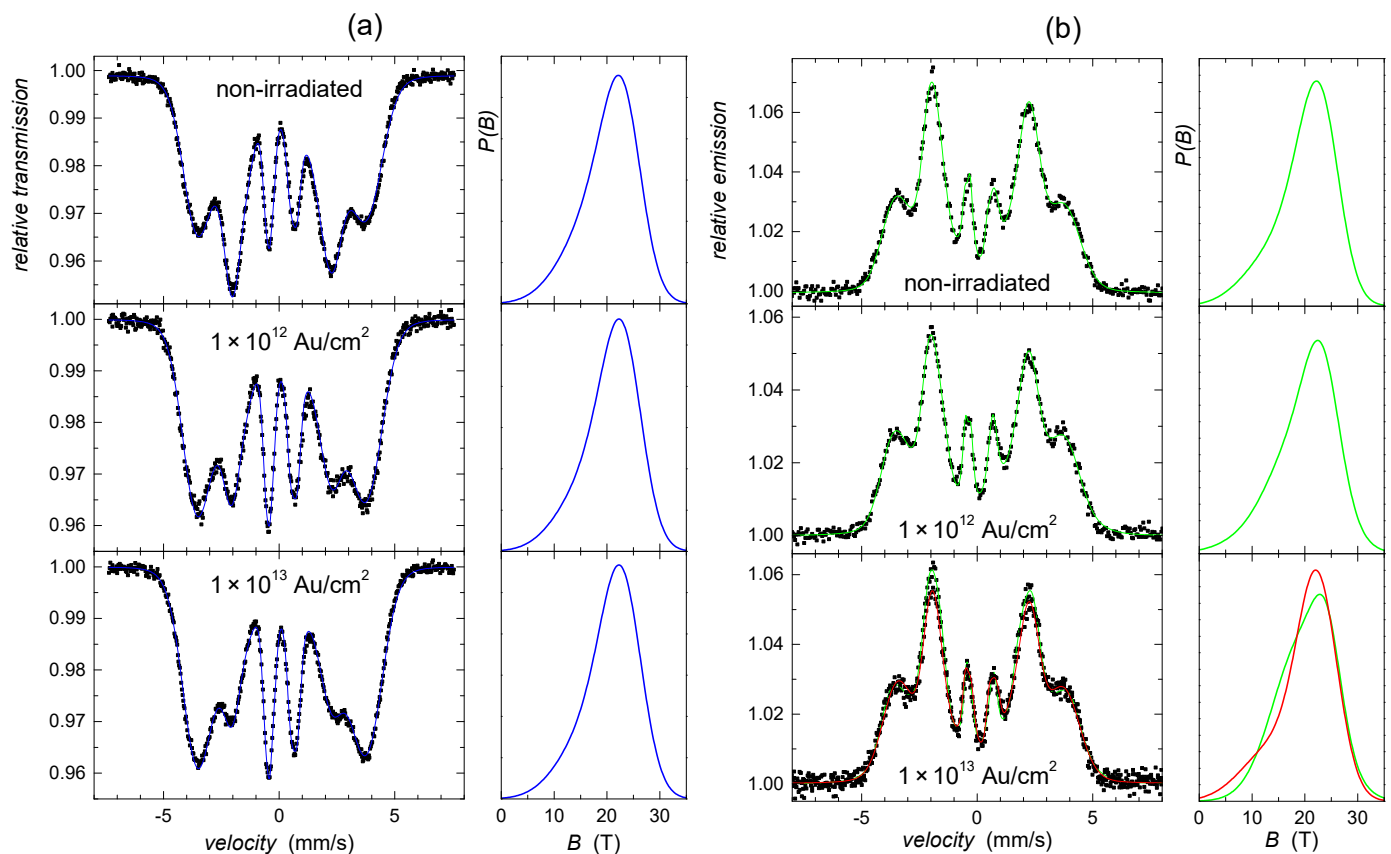
Figure 21. Mössbauer spectra (left-hand panels) and corresponding P(B) distributions (right-hand panels) of \text{Fe}_{74}\text{Cu}_{11}\text{Nb}_3\text{Si}_{16}\text{B}_6 amorphous metallic alloy irradiated by 593 MeV Au ions with the indicated fluences: (a) transmission geometry (blue); (b) CEMS (green). Mössbauer spectrum taken from the wheel side of the ribbons is shown for comparison in (b) together with the corresponding P(B) (red).
