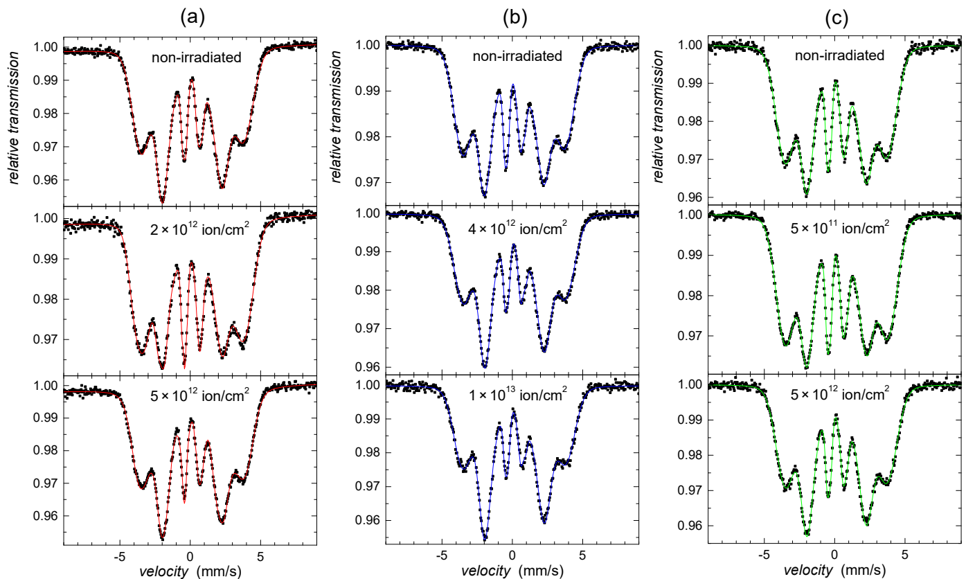
Figure 19. Mössbauer spectra of \text{Fe}_{73}\text{Cu}_1\text{Nb}_3\text{Si}_{16}\text{B}_7 amorphous metallic alloy recorded in transmission geometry after irradiation by: (a) 5.9 MeV/u ^{238}\text{U} ions (red); (b) 11.1 MeV/u ^{131}\text{Xe} ions (blue); (c) 11.1 MeV/u ^{197}\text{Au} ions (green) with the indicated fluences.
