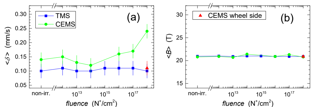
Figure 7. Parameters derived from transmission (TMS, blue) and CEMS (green) Mössbauer spectra of Fe_{74}Cu_{11}Nb_3Si_{16}B_6 irradiated by 110 keV N^+ ions plotted against the ion fluence: (a) average isomer shift, \langle \delta \rangle ; (b) average hyperfine magnetic field, \langle B \rangle . Red triangles correspond to CEMS spectrum taken from the wheel side of the ribbons. Solid lines are only guides for the eye.
