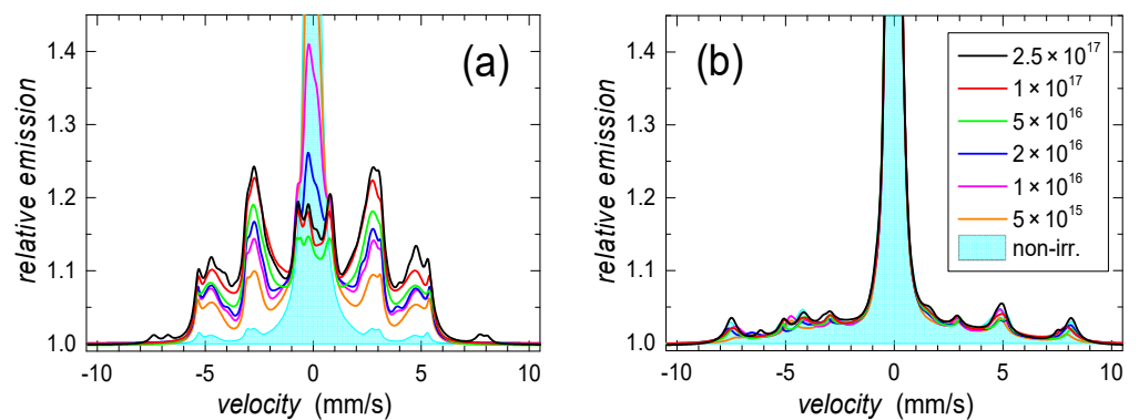
Figure 13. CEMS spectra of ^{57}\text{Fe}_{81}\text{Mo}_8\text{Cu}_1\text{B}_{10} amorphous metallic ribbons recorded from its: (a) air side; (b) wheel side after irradiation by 130 keV \text{N}^+ ions with the indicated fluences.
