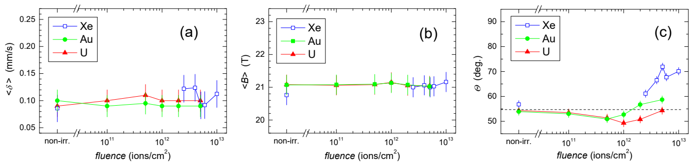
Figure 20. Parameters derived from transmission Mössbauer spectra of \text{Fe}_{73}\text{Cu}_1\text{Nb}_3\text{Si}_{16}\text{B}_7 amorphous metallic alloy irradiated by the indicated heavy ions: (a) average isomer shift, \langle\delta\rangle ; (b) average hyperfine magnetic field, \langle B \rangle ; (c) angle \Theta as a function of ion fluence. Dashed line in (c) represents \Theta -values that correspond to random orientations of spins. Solid lines are only guides for the eye.
