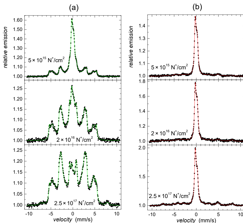
Figure 12. CEMS spectra of ^{57}Fe_{81}Mo_8Cu_1B_{10} amorphous metallic ribbons recorded from its: (a) Air side (green); (b) wheel side (red) after irradiation by 130 keV N^+ ions with the indicated fluences.
