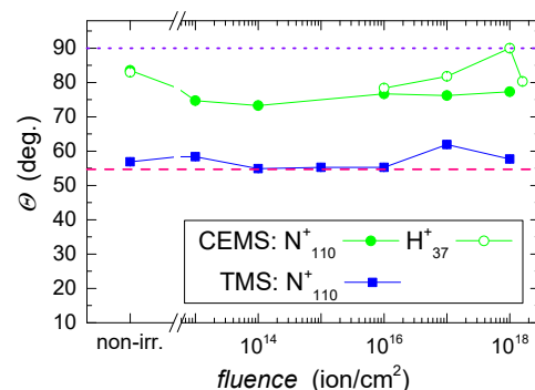
Figure 9. Orientations of net magnetic moments characterized by the angle \Theta of the \text{Fe}_{74}\text{Cu}_1\text{Nb}_3\text{Si}_{16}\text{B}_6 amorphous metallic alloy exposed to 37 keV \text{H}^+ and 110 keV \text{N}^+ ions plotted against the ion fluence. Pink dashed and violet dotted lines represent \Theta -values that correspond to random and in-plane orientations of spins, respectively. Solid lines are only guides to an eye.
