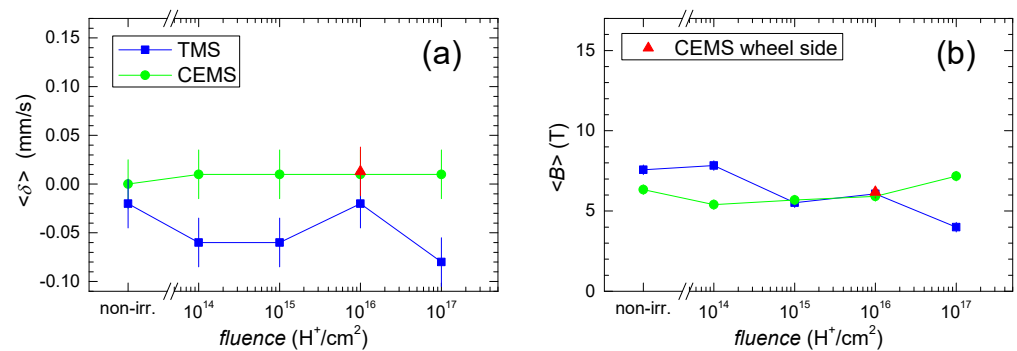
Figure 2. Parameters derived from transmission (TMS, blue) and CEMS (green) Mössbauer spectra of Fe 76 Mo 8 Cu 1 B 15 irradiated by 80 keV H + ions plotted against the ion fluence: (a) Average isomer shift, \langle\delta\rangle ; (b) average hyperfine magnetic field, \langle B\rangle . Red triangles correspond to CEMS spectrum taken from the wheel side of the ribbons. Solid lines are only guides for the eye.
