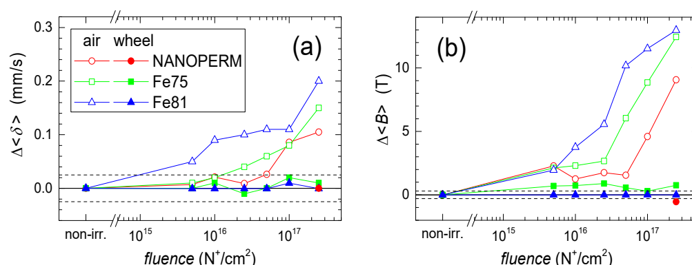
Figure 18. Differences of parameters derived from CEMS spectra of Fe_{76}Mo_8Cu_1B_{15} (NANOPERM-type, red circles), ^{57}Fe_{75}Mo_8Cu_1B_{16} (Fe75, green squares), and ^{57}Fe_{81}Mo_8Cu_1B_{10} (Fe81, blue triangles) amorphous metallic alloys irradiated by 130 keV N^+ ions plotted against the ion fluence: (a) Average isomer shift, \Delta\langle\delta\rangle ; (b) average hyperfine magnetic field, \Delta\langle B\rangle . Open and solid symbols correspond to CEMS spectra taken from air and wheel sides of the ribbons, respectively. Solid lines are only guides for the eye, dashed lines represent the error margins.
