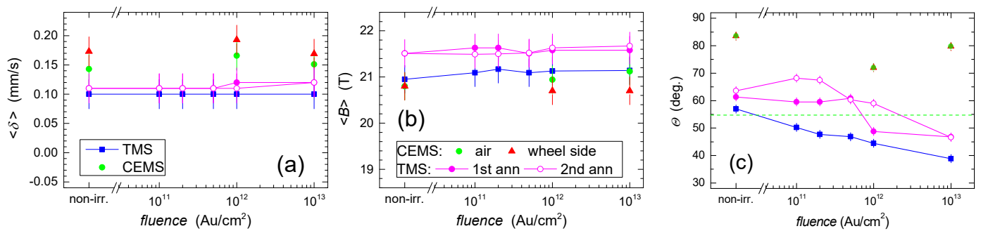
Figure 22. Parameters derived from transmission (TMS, blue) and CEMS (green) Mössbauer spectra of \text{Fe}_{74}\text{Cu}_1\text{Nb}_3\text{Si}_{16}\text{B}_6 irradiated by 593 keV Au ions plotted against the ion fluence: (a) average isomer shift, \langle\delta> ; (b) average hyperfine magnetic field, \langle B \rangle ; (c) angle \Theta . Red triangles correspond to CEMS spectra taken from the wheel side of the ribbons. Parameters corresponding to the annealed samples are plotted in magenta. Dashed line in (c) represents \Theta -values that correspond to random orientations of spins. Solid lines are only guides for the eye.
