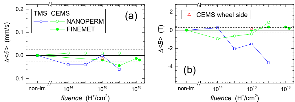
Figure 10. Differences of parameters derived from transmission (TMS, blue) and CEMS (green) Mössbauer spectra of Fe_{74}Cu_1Nb_3Si_{16}B_6 (FINEMET-type, solid symbols) and Fe_{76}Mo_8Cu_1B_{15} (NANOPERM-type, open symbols) metallic alloys irradiated by 37 keV and 80 keV H^+ ions, respectively, plotted against the ion fluence: (a) average isomer shift, \Delta\langle\delta\rangle ; (b) average hyperfine magnetic field, \Delta\langle B \rangle . Red triangles correspond to CEMS spectra taken from the wheel side of the ribbons. Solid lines are only guides for the eye, dashed lines represent the error margins.
