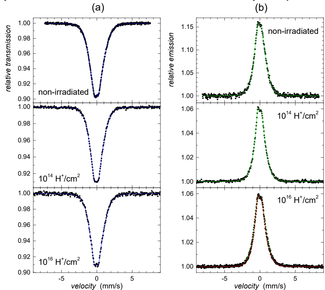
Figure 1. Mössbauer spectra of \text{Fe}_{76}\text{Mo}_8\text{Cu}_1\text{B}_{15} amorphous metallic alloy irradiated by 80 keV \text{H}^+ ions with the indicated fluences: (a) Transmission geometry (blue); (b) conversion electron Mössbauer spectroscopy (CEMS, green). Mössbauer spectrum taken from the wheel side of the ribbons is shown for comparison in (b) (red).
