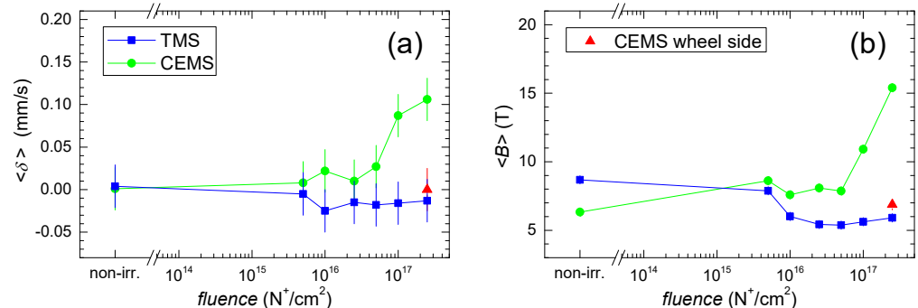
Figure 4. Parameters derived from transmission (TMS, blue) and CEMS (green) Mössbauer spectra of \text{Fe}_{76}\text{Mo}_8\text{Cu}_1\text{B}_{15} irradiated by 130 keV N^+ ions plotted against the ion fluence: (a) Average isomer shift, \langle\delta\rangle ; (b) average hyperfine magnetic field, \langle B\rangle . Red triangles correspond to the CEMS spectrum taken from the wheel side of the ribbons. Solid lines are only guides for the eye.
