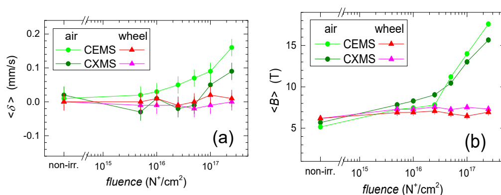
Figure 17. Parameters derived from CEMS and CXMS spectra recorded from the air (circles) and wheel (triangles) sides of ^{57}\text{Fe}_{75}\text{Mo}_8\text{Cu}_1\text{B}_{16} irradiated by 130 keV \text{N}^+ ions plotted against the ion fluence: (a) Average isomer shift, \langle\delta\rangle ; (b) average hyperfine magnetic field, \langle B\rangle . Solid lines are only guides for the eye.
