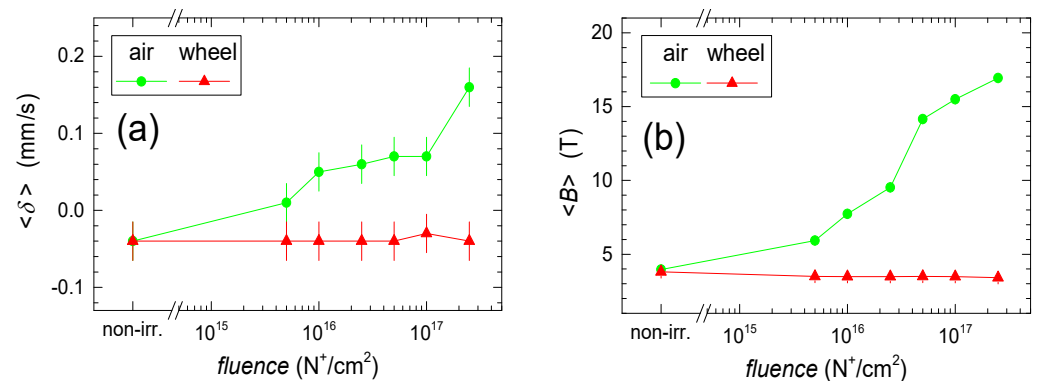
Figure 14. Parameters derived from CEMS spectra recorded from the air (green circles) and wheel (red triangles) sides of the ribbons of ^{57}\text{Fe}_{81}\text{Mo}_8\text{Cu}_1\text{B}_{10} irradiated by 130 keV \text{N}^+ ions plotted against the ion fluence: (a) average isomer shift, \langle\delta\rangle ; (b) average hyperfine magnetic field, \langle B\rangle . Solid lines are only guides for the eye.
