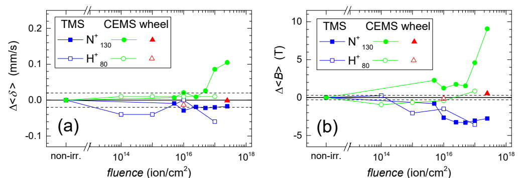
Figure 5. Differences of parameters derived from transmission (TMS, blue) and CEMS (green) Mössbauer spectra of irradiated and non-irradiated \text{Fe}_{76}\text{Mo}_8\text{Cu}_1\text{B}_{15} amorphous metallic alloy exposed to 80 keV H^+ and 130 keV N^+ ions as plotted against the ion fluence: (a) average isomer shift, \Delta\langle\delta\rangle ; (b) average hyperfine magnetic field, \Delta\langle B\rangle . Red triangles correspond to CEMS spectra taken from the wheel side of the ribbons. Solid lines are only guides for the eye, dashed lines represent the error margins.
