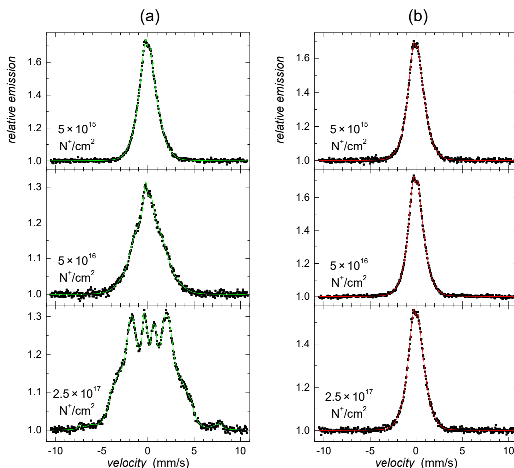
Figure 15. CEMS spectra of ^{57}\text{Fe}_{75}\text{Mo}_8\text{Cu}_1\text{B}_{16} amorphous metallic ribbons recorded from its: (a) air side (green); (b) wheel side (red) of the ribbons after irradiation by 130 keV \text{N}^+ ions with the indicated fluences.
