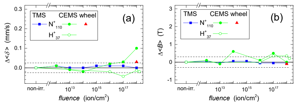
Figure 8. Differences of parameters derived from transmission (TMS, blue) and CEMS (green) Mössbauer spectra of irradiated and non-irradiated \text{Fe}_{74}\text{Cu}_1\text{Nb}_3\text{Si}_{16}\text{B}_6 amorphous metallic alloy exposed to 37 keV \text{H}^+ and 110 keV \text{N}^+ ions as plotted against the ion fluence: (a) average isomer shift, \Delta\langle\delta\rangle ; (b) average hyperfine magnetic field, \Delta\langle B\rangle . Red triangles correspond to CEMS spectra taken from the wheel side of the ribbons. Solid lines are only guides for the eye, dashed lines represent the error margins.
