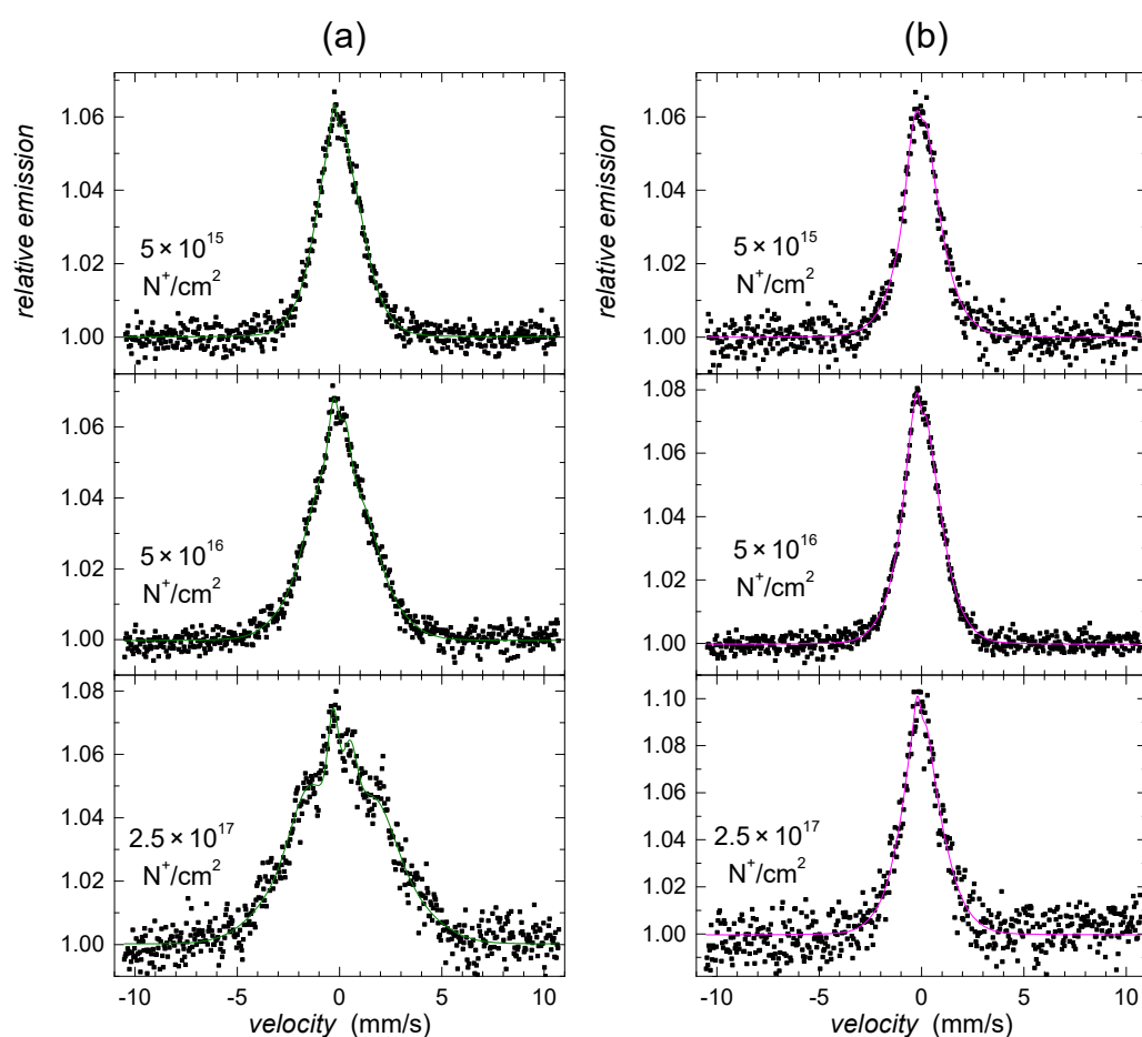
Figure 16. CXMS spectra of ^{57}\text{Fe}_{75}\text{Mo}_8\text{Cu}_1\text{B}_{16} amorphous metallic ribbons recorded from its: (a) air side (dark green); (b) wheel side (magenta) of the ribbons after irradiation by 130 keV \text{N}^+ ions with the indicated fluences.
