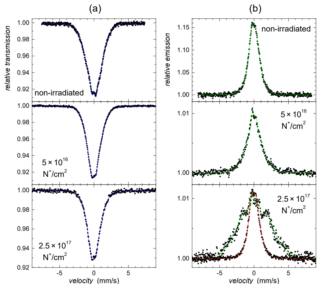
Figure 3. Mössbauer spectra of Fe 76 Mo 8 Cu 1 B 15 amorphous metallic alloy irradiated by 130 keV N + ions with the indicated fluences: (a) Transmission geometry (blue); (b) CEMS (green). The Mössbauer spectrum taken from the wheel side of the ribbons is shown for comparison in (b) (red).
