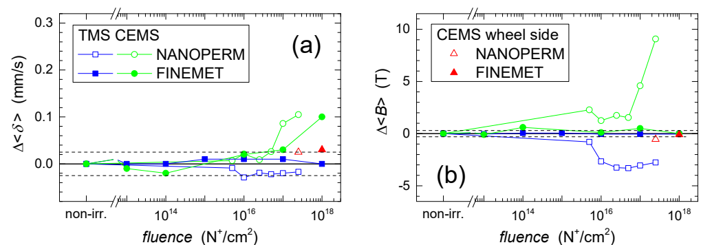
Figure 11. Differences of parameters derived from transmission (TMS, blue) and CEMS (green) Mössbauer spectra of Fe_{74}Cu_1Nb_3Si_{16}B_6 (FINEMET-type, solid symbols) and Fe_{76}Mo_8Cu_1B_{15} (NANOPERM-type, open symbols) metallic alloys irradiated by 110 keV and 130 keV N^+ ions, respectively, plotted against the ion fluence: (a) average isomer shift, \Delta\langle\delta\rangle ; (b) average hyperfine magnetic field, \Delta\langle B \rangle . Red triangles correspond to CEMS spectra taken from the wheel side of the ribbons. Solid lines are only guides for the eye, dashed lines represent the error margins.
