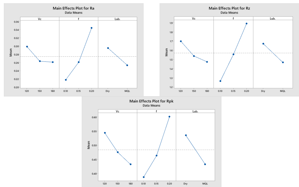
Figure 2. Main effect plots for Ra, Rz, and Rpk.
