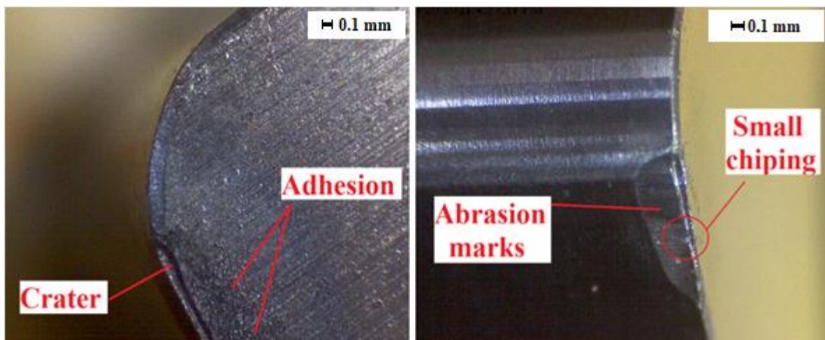
Figure 8. Tool wear after 28 min cutting time in MQL.
