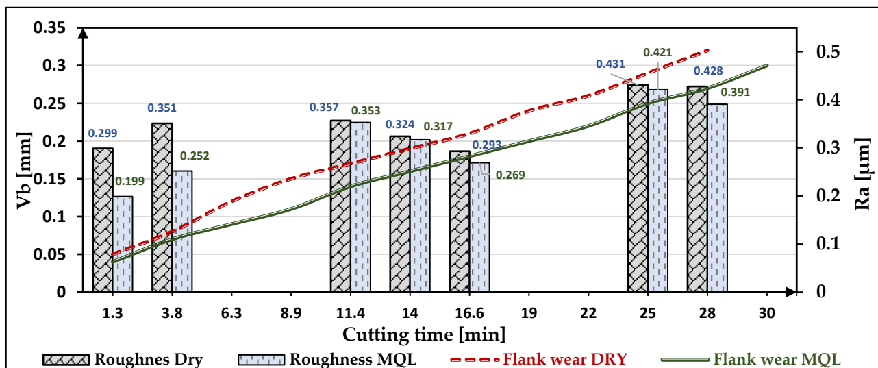
Figure 6. Tool wear progression and related Ra.
