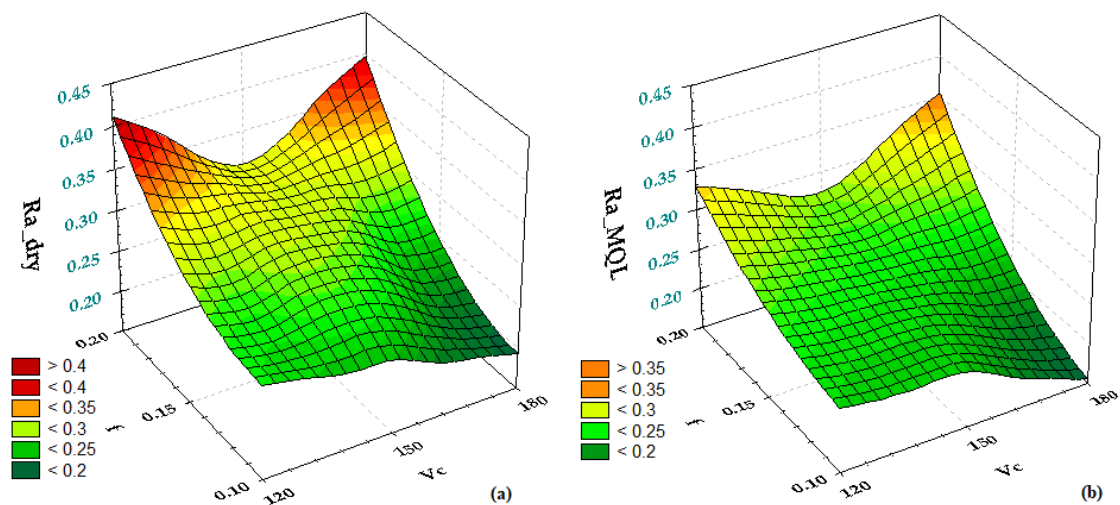
Figure 3. Mean Ra vs. feed and cutting speed in dry (a) and MQL (b).
