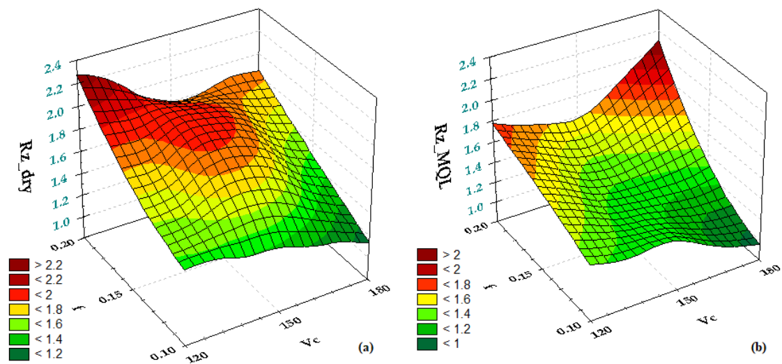
Figure 4. Mean Rz vs. feed and cutting speed in dry (a) and MQL (b).
