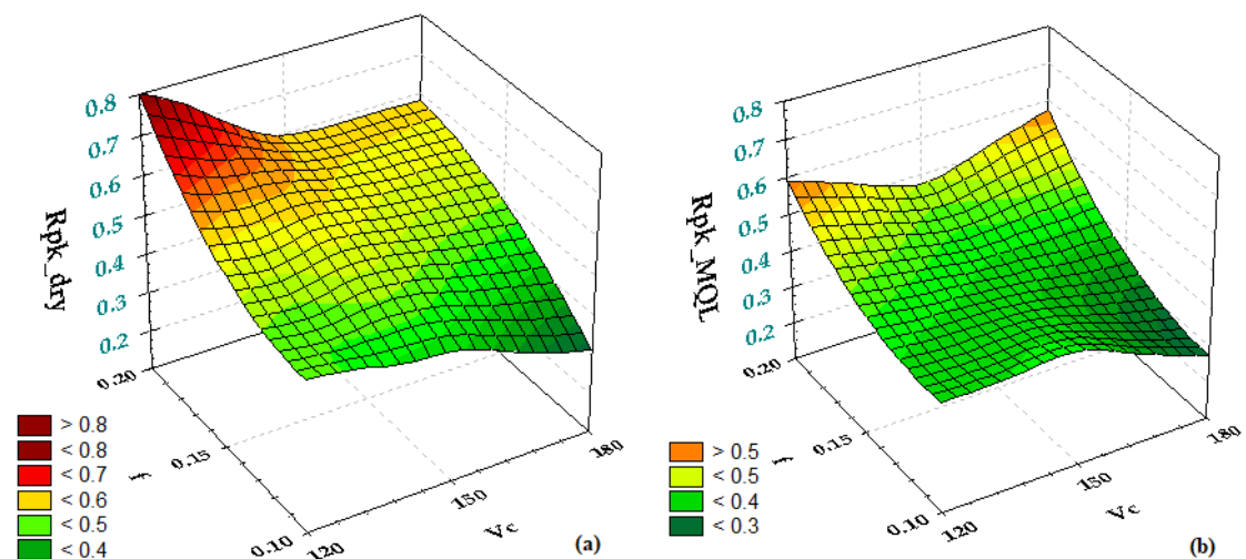
Figure 5. Mean Rpk vs. feed and cutting speed in dry (a) and MQL (b).
