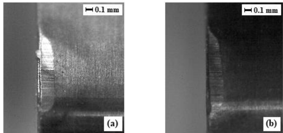
Figure 7. Flank wear in dry (a) and MQL (b) after 14 min cutting time.
