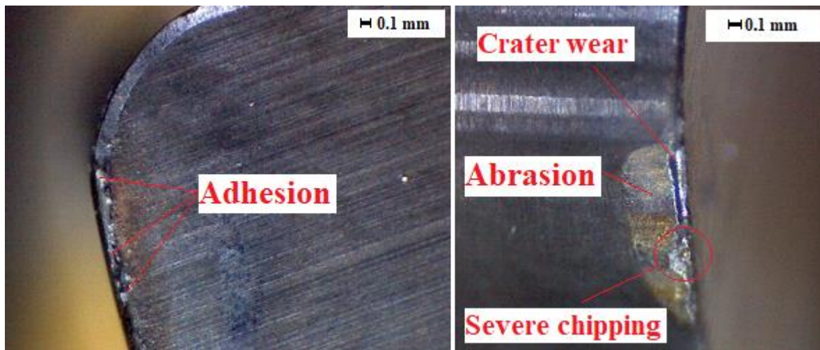
Figure 9. Tool wear after 28 min cutting time in dry.
