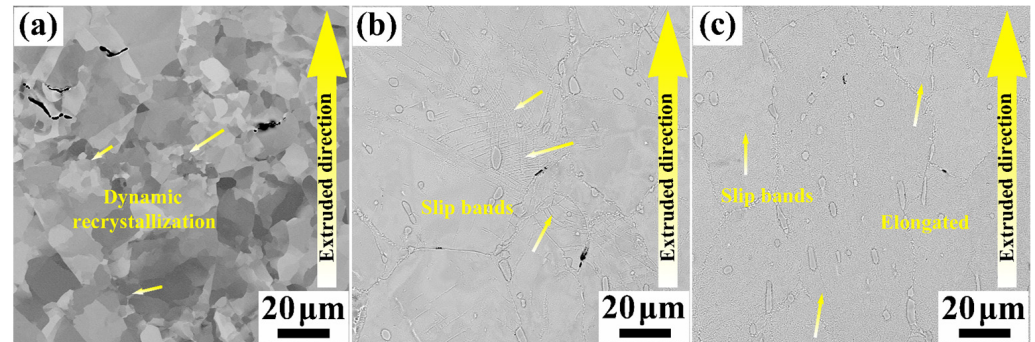
Figure 7. The post-fracture cross-sectional morphologies of the three samples were observed at 1073 K: (a) Al10 1273 K 1 h, (b) Al10 1473 K 10 min, and (c) Al10 1473 K 10 min + 973 K 10 h. The arrow indicates the extruded direction.
