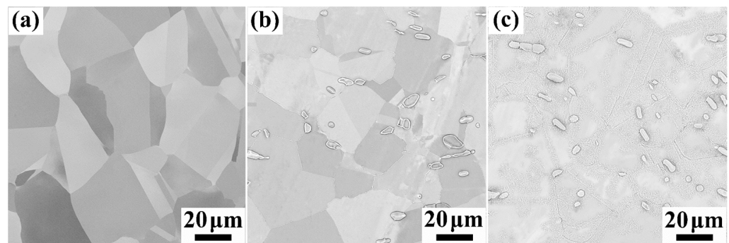
Figure 1. SEM morphologies of R1273, R1473, and A973 samples at (a) Al10 1273 K 1 h, (b) Al10 1473 K 10 min, and (c) Al10 1473 K 10 min + 973 K 10 h, respectively.
