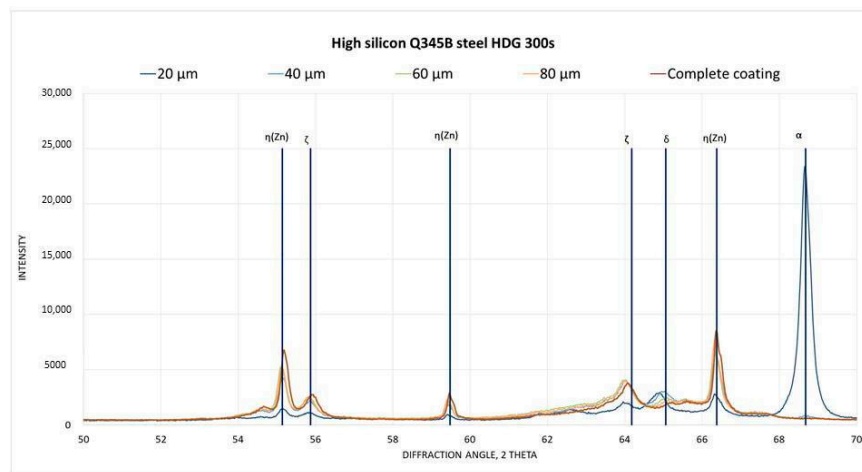
Figure 12. High-silicon steel XRD pattern.
