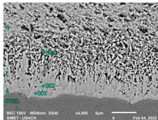
Figure 6. \alpha/\delta/\zeta/\eta interface analysis in 15 s, high-silicon steel.
