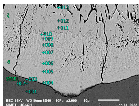
Figure 8. \alpha/\delta/\zeta interface analysis in 300 s, high-silicon steel.
