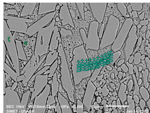
Figure 9. \zeta/\eta interface analysis in 300 s, high-silicon steel.
