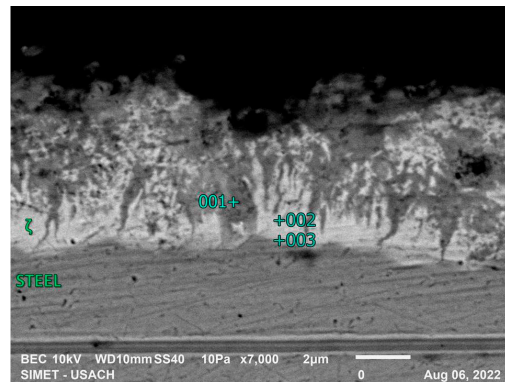
Figure 4. Steel/zinc interface analysis in 5 s, low-silicon steel.
