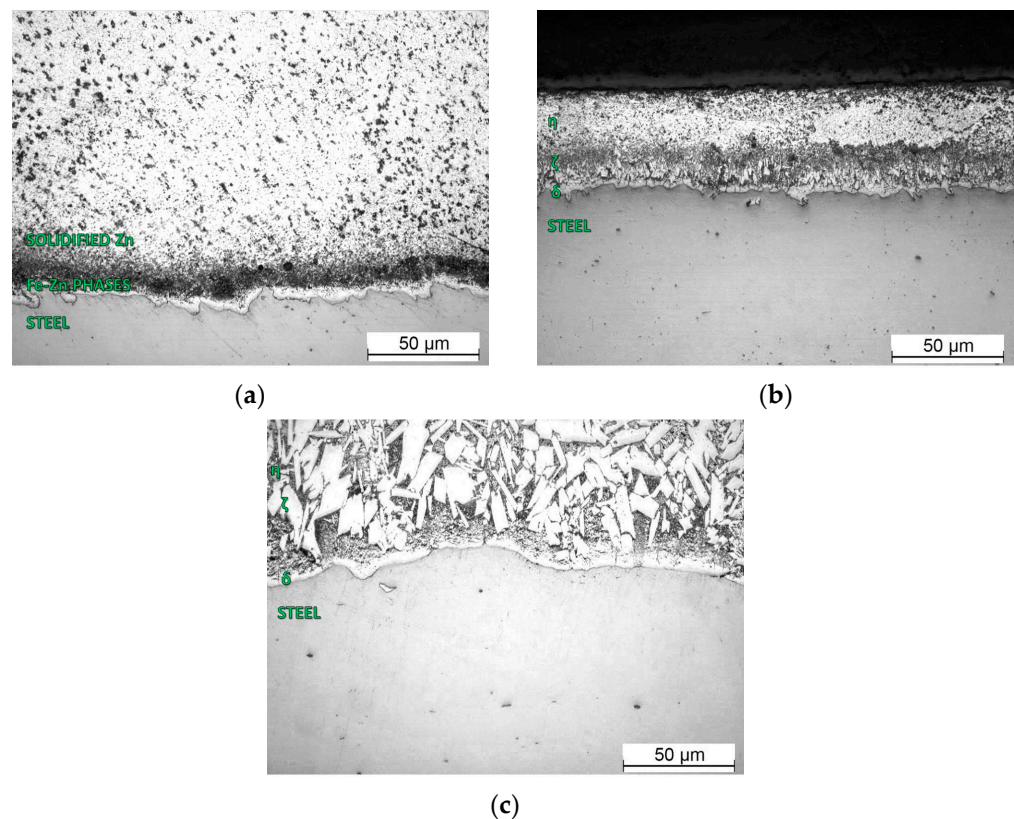
Figure 3. Microstructural evolution of galvanized steel Q345B high in silicon: (a) 15 s; (b) 30 s; (c) 300 s.
