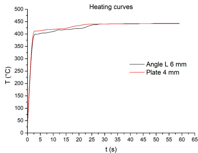
Figure 1. Heating curves during galvanizing.
