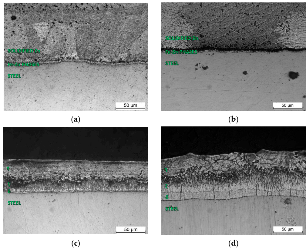
Figure 2. Microstructural evolution of galvanized ASTM A36 low-silicon steel: (a) 5 s; (b) 15 s; (c) 30 s; (d) 300 s.
