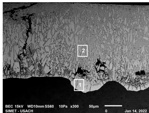
Figure 7. 300 s microstructure, high-silicon steel.
