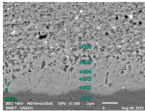
Figure 5. Steel/zinc interface analysis in 15 s, low-silicon steel.
