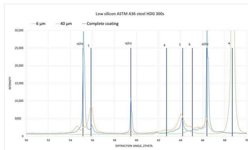
Figure 11. Low-silicon steel XRD pattern.
