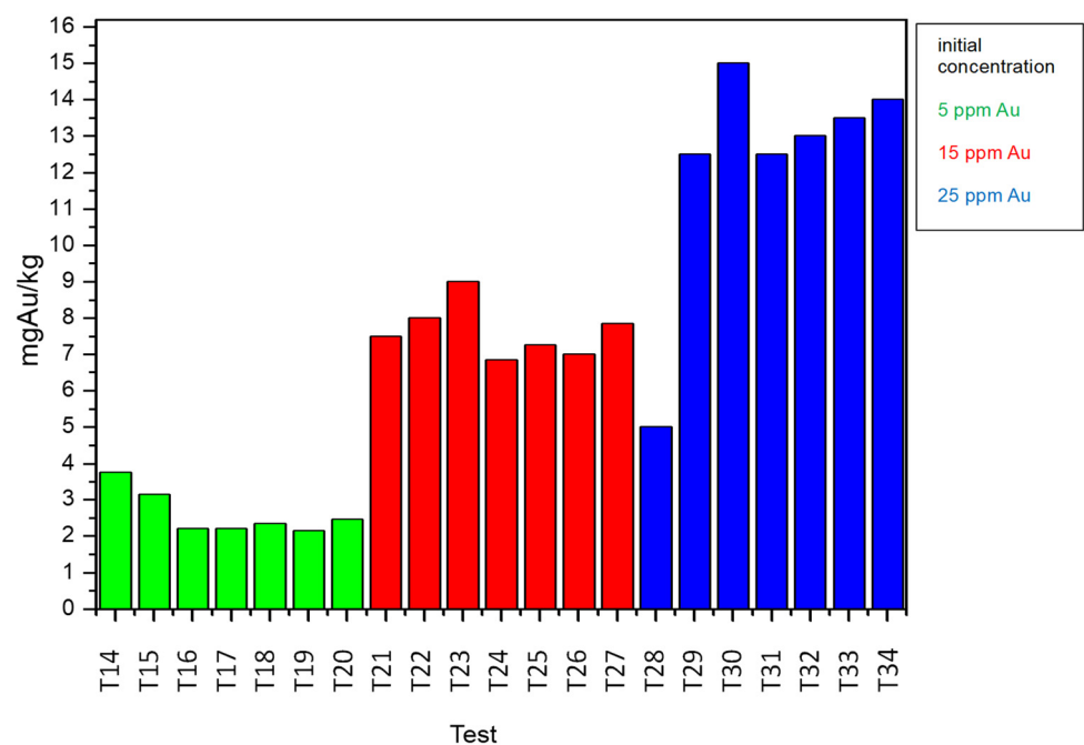
Figure 5. mg Au/kg-ql loss in the accurate ratio tests.
