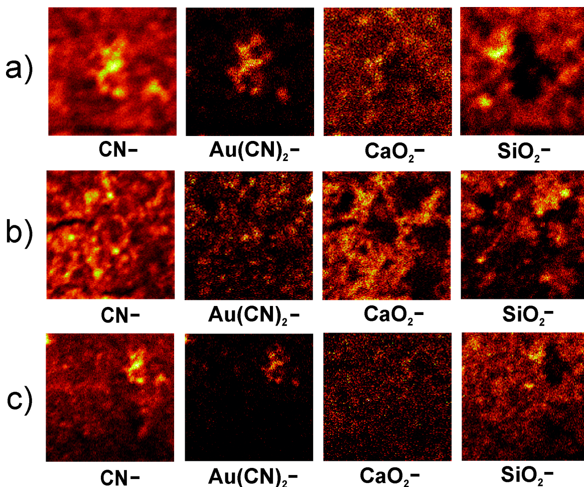
Figure 15. Secondary ion images of some cluster ions for samples (a) T14, (b) T15, and (c) T16. Image size is 250 \times 250 microns ( 256 \times 256 pixels).
