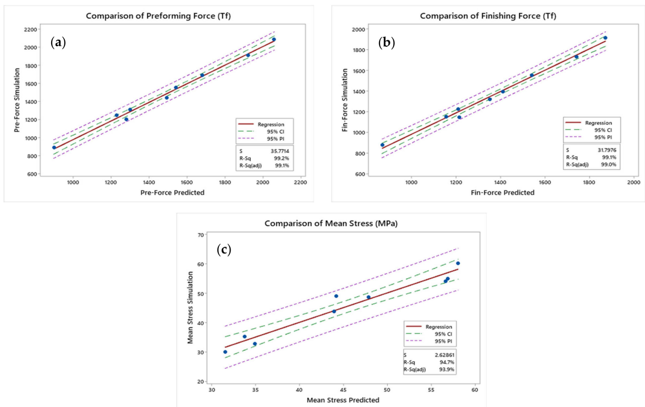
Figure 6. Comparison of (a) maximum preforming force, (b) maximum finishing force, and (c) maximum mean stresses: simulation vs. predictions by linear regression model.
