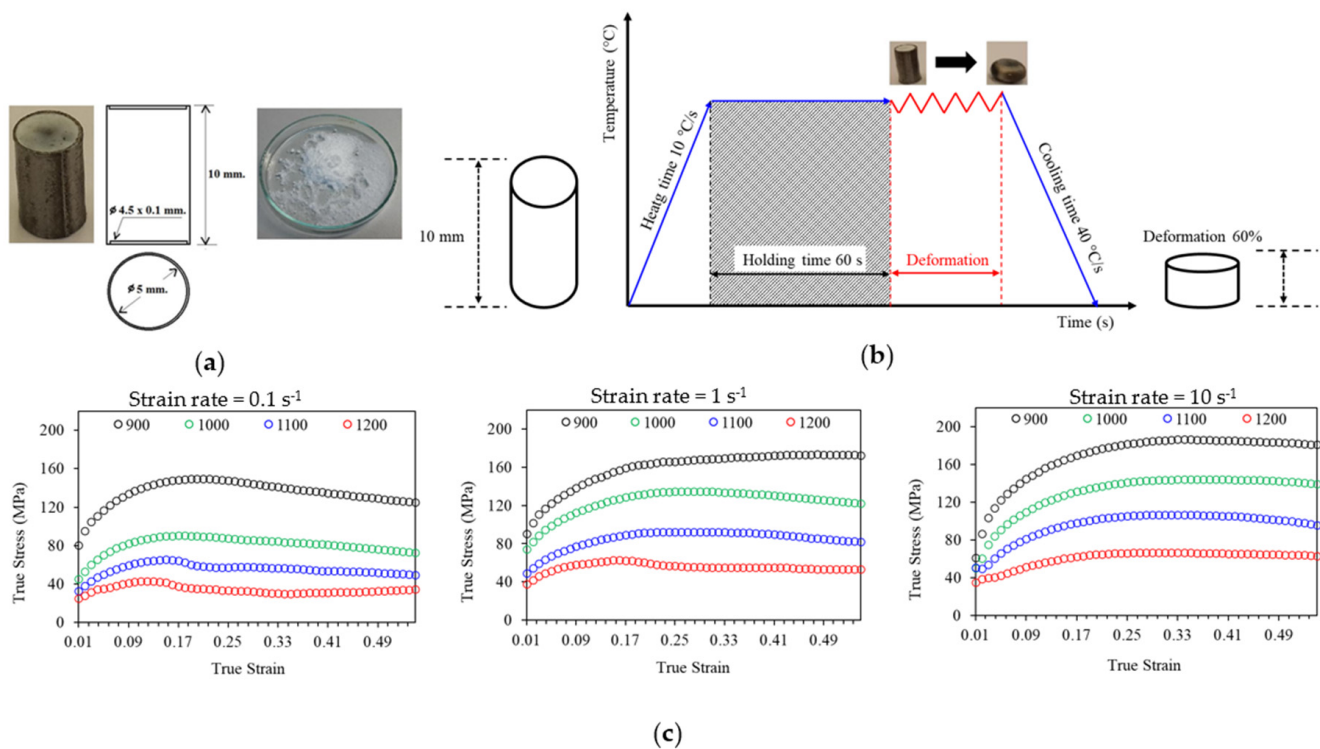
Figure 1. (a) Alumina punch; (b) schematic diagram of the hot compression test; and (c) flow curves from the hot compression test at strain rates of 0.1, 1, and 10 s −1 under various deformation conditions.
