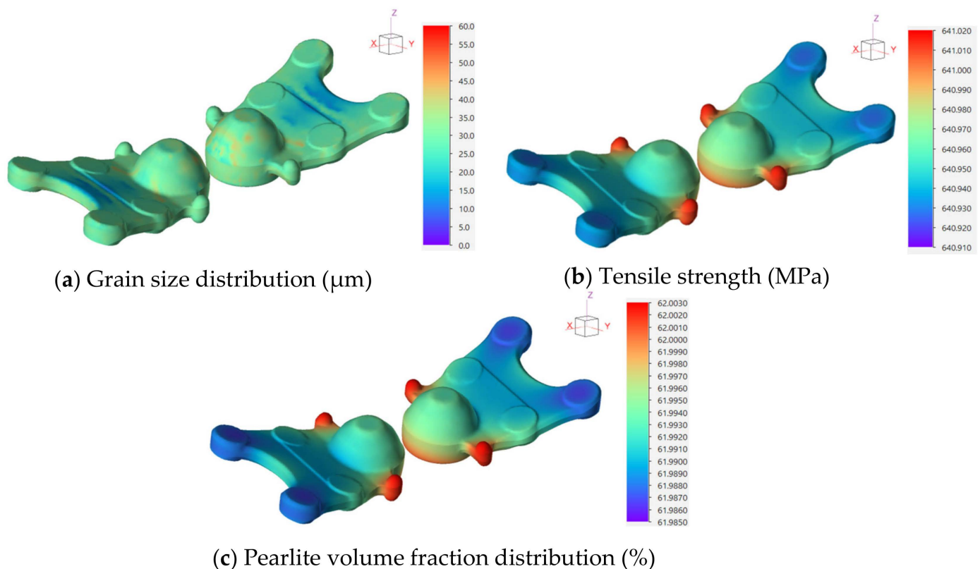
Figure 8. FE simulation results of the forged part: (a) grain size ( \mu\text{m} ), (b) tensile strength (MPa), and (c) pearlite volume fraction distribution (%).
