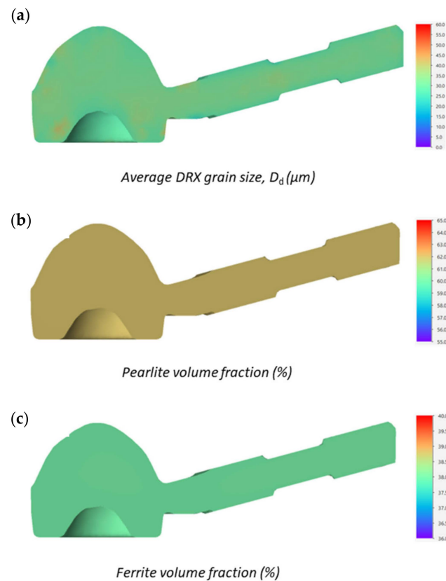
Figure 10. FE simulation results showing the distribution of (a) the average DRX grain size, (b) the pearlite volume fraction, and (c) the ferrite volume fraction in the cross-section of the forged ball joint.
