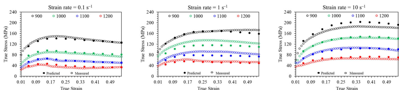
Figure 4. Comparing the experimental flow curves with the prediction from the Arrhenius-based constitutive equation.
