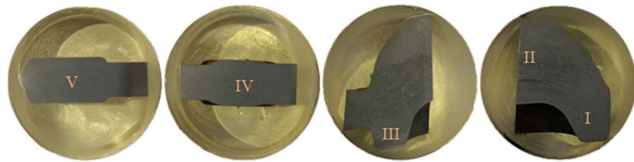
Figure 9. Mounted cross-section of the ball joint, prepared for a microstructure analysis, with the study points indicated.
