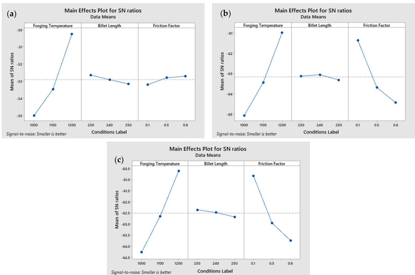
Figure 5. Main effects plots for S/N ratios (lower is better) for (a) the preforming force, (b) the finishing force, and (c) the mean stress during the FEM simulation.
