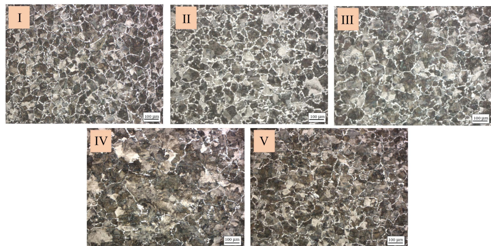
Figure 11. Observed microstructures at the study points in the ball joint cross-section.
