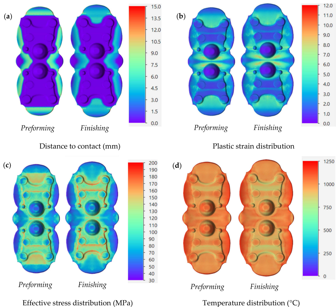
Figure 7. Contour color of (a) distance to contact, (b) plastic strain, (c) effective stress, and (d) temperature distribution after preforming and finishing processes.
