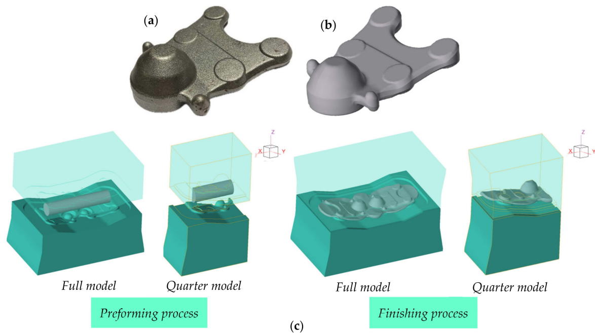
Figure 2. Final shape of the ball joint, depicting (a) the actual object, (b) the CAD model, and (c) the FE of the hot forging process, which is shown in full and quarter models.
