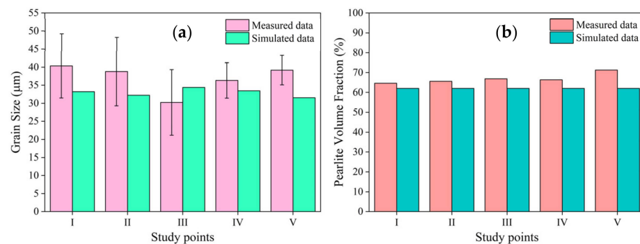
Figure 12. Bar graph showing the comparison of the simulated and measured values for (a) the DRX grain size and (b) the pearlite volume fraction of the ball joint after it cooled to room temperature at the study points.
