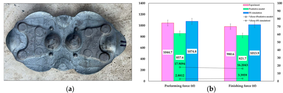
Figure 13. Verification result; (a) experimental outcome; and (b) forging load comparison between the experiment, predictive model, FE simulation, and % error.
