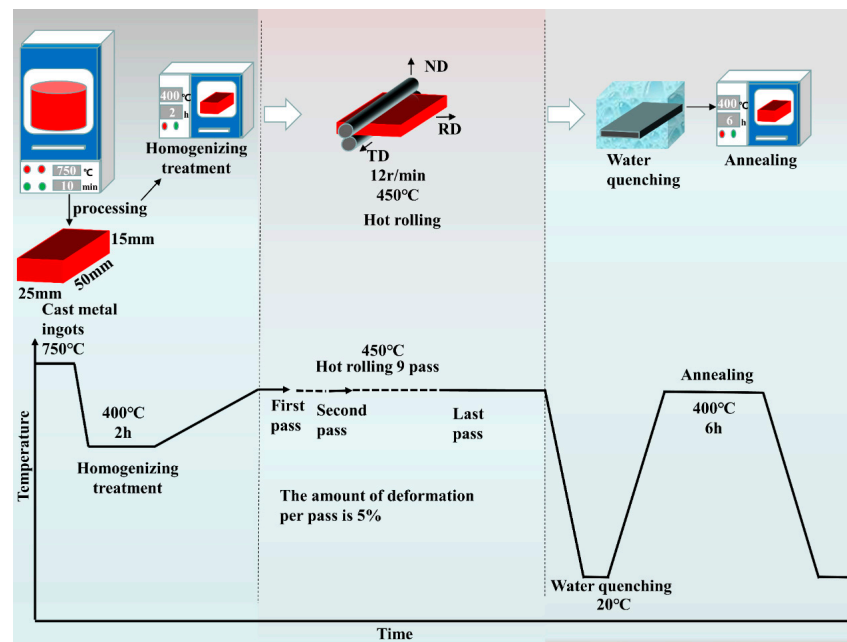
Figure 1. Schematic diagram of the magnesium alloy preparation process.
