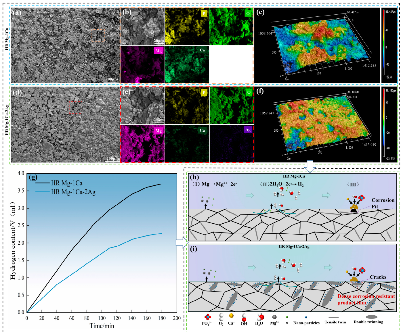
Figure 5. Morphological characterization of alloys after 3 h immersion in simulated body fluid (SBF): (a) SEM micrograph showing corrosion morphology of HR Mg-1Ca alloy; (b) EDS elemental mapping of HR Mg-1Ca alloy; (c) 3D topographic profile of corroded HR Mg-1Ca alloy surface; (d) SEM micrograph of corroded HR Mg-1Ca-2Ag alloy; (e) EDS elemental mapping of HR Mg-1Ca-2Ag alloy; (f) 3D surface topography of corroded HR Mg-1Ca-2Ag alloy; (g) Corrosion rate comparison between HR Mg-1Ca and HR Mg-1Ca-2Ag alloys; (h) Schematic representation of corrosion mechanism in HR Mg-1Ca alloy; (i) Schematic representation of corrosion mechanism in HR Mg-1Ca-2Ag alloy.
