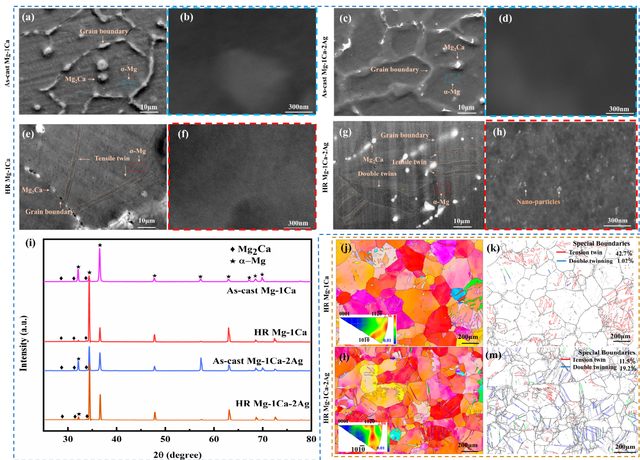
Figure 2. (a,b) FESEM images of as-cast Mg-1Ca alloy; (c,d) FESEM images of as-cast Mg-1Ca-2Ag alloy; (e,f) FESEM images of hot-rolled Mg-1Ca alloy; (g,h) FESEM images of hot-rolled Mg-1Ca-2Ag alloy; (i) XRD spectra of Mg-1Ca and Mg-1Ca-2Ag alloys; (j,k) Grain orientation maps and twin type distribution of hot-rolled Mg-1Ca alloy; (l,m) Grain orientation maps and twin type distribution of hot-rolled Mg-1Ca-2Ag alloy.
