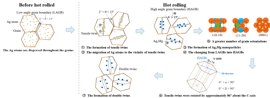
Figure 4. Schematic diagram of the effect of Ag 3 Mg nanoscale particles on twin formation and grain orientation evolution during deformation in hot-rolled Mg-1Ca-2Ag.
