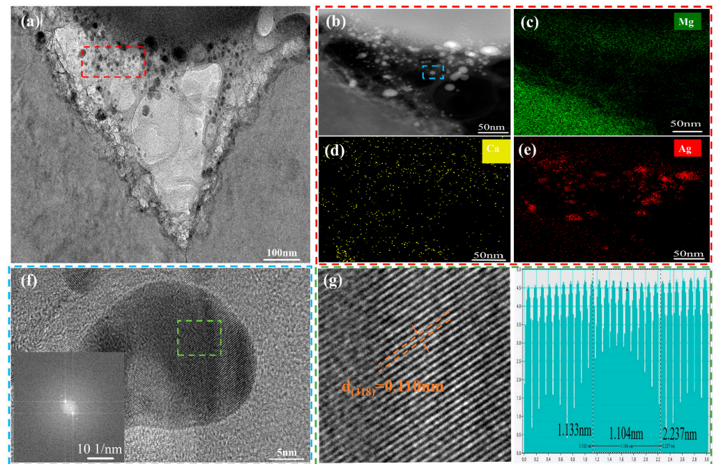
Figure 3. Phase distribution and TEM analysis of hot-rolled Mg-1Ca-2Ag alloy: (a) Twins and nanoscale precipitates in hot-rolled Mg-1Ca-2Ag; (b–e) TEM images and EDS elemental maps of nanoscale precipitates; (f,g) Lattice spacing of nanoscale particles.
