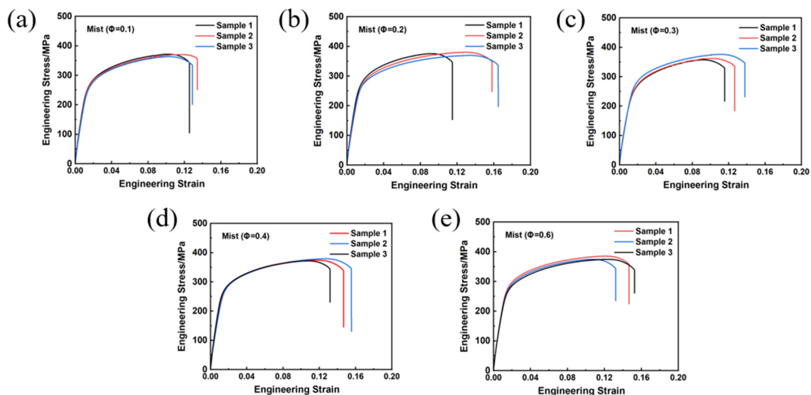
Figure 7. Tensile test at room temperature of the samples after heat treatment: (a) mist ( \phi = 0.10\% ); (b) mist ( \phi = 0.20\% ); (c) mist ( \phi = 0.30\% ); (d) mist ( \phi = 0.40\% ); (e) mist ( \phi = 0.60\% ).
