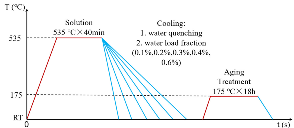
Figure 3. Schematic diagram of water-mist spray-quenching experiments. Red lines represent the heating stage, and blue lines represent the cooling/quenching stage.
