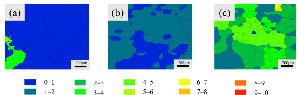
Figure 11. GND under different O-state pre-strains: (a) O-state pre-strain: 0; (b) O-state pre-strain: 0.1; (c) O-state pre-strain: 0.2.
