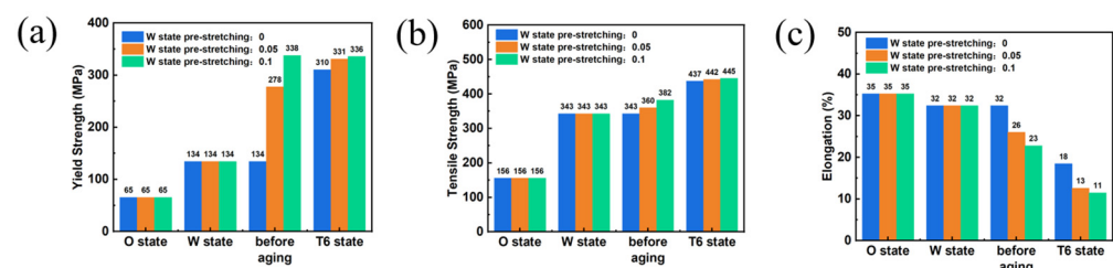
Figure 13. Tensile properties with no O-state pre-strain under different W-state pre-strain levels at room temperature of the samples after: (a) yield strength; (b) tensile strength; (c) elongation.
