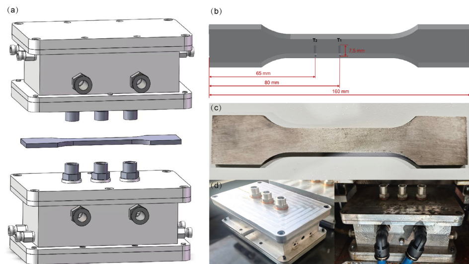
Figure 2. Cooling platform and workpiece. (a) 3D top and bottom cooling assembly with the workpiece in the middle; (b) dimensions and temperature sensor location; (c) photograph of the work piece; (d) photograph of the upper cooling platform (left). The cooling platform connected with the working media piping.
