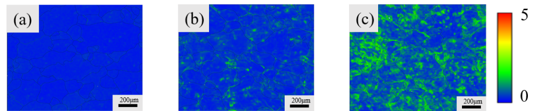
Figure 14. GND under different W-state pre-strains: (a) W-state pre-strain: 0; (b) W-state pre-strain: 0.05; (c) W-state pre-strain: 0.1.
