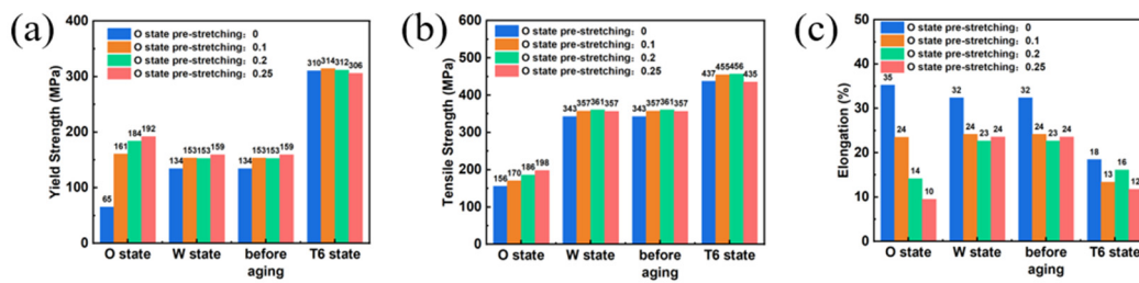
Figure 10. Tensile properties with no W-state pre-strain under different O-state pre-strain levels at room temperature of the samples after heat treatment: (a) yield strength; (b) tensile strength; (c) elongation.
