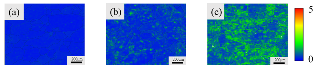
Figure 11. GND under different O-state pre-strains: (a) O-state pre-strain: 0; (b) O-state pre-strain: 0.1; (c) O-state pre-strain: 0.2.
