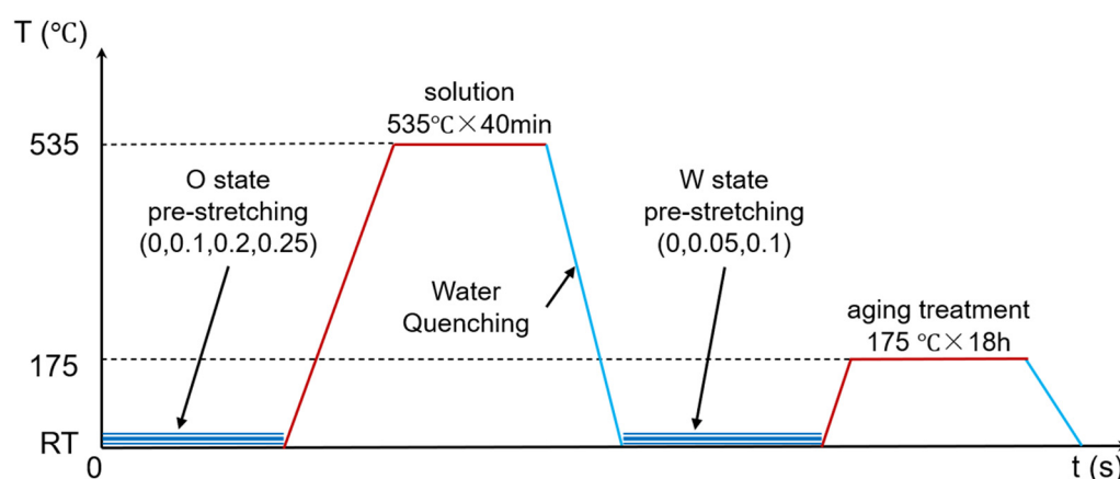
Figure 4. Schematic diagram of pre-strain heat treatment at different deformation levels. Red lines represent the heating stage, and blue lines represent the cooling/quenching stage.
