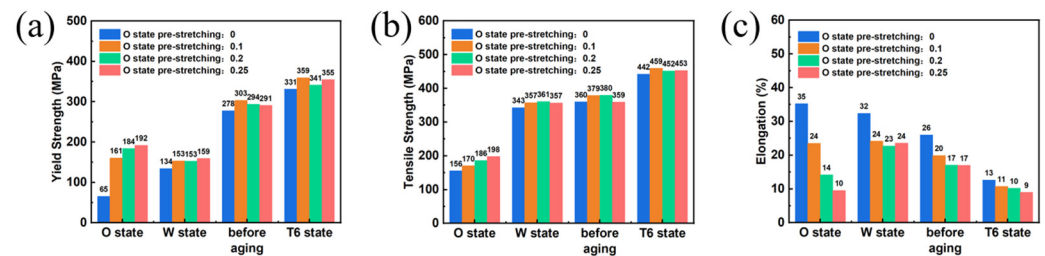
Figure 16. Tensile properties with W-state pre-strain of 0.05 under different O-state pre-strain levels at room temperature of the samples after heat treatment: (a) yield strength; (b) tensile strength; (c) elongation.
