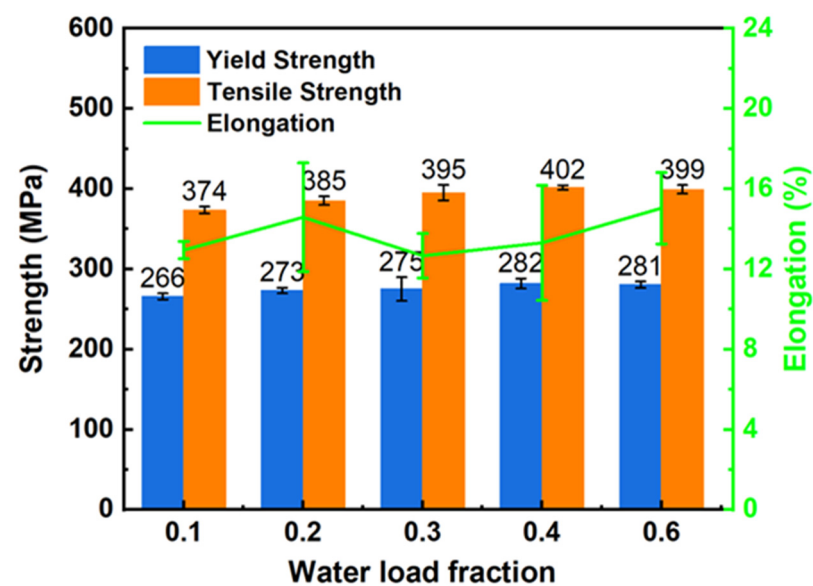
Figure 8. Comparison of material mechanical properties at different water loading fractions.
