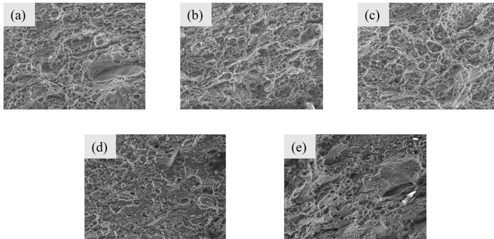
Figure 9. Fracture morphology of room-temperature tensile specimens under different water vapor ratios: (a) mist ( \phi = 0.10\% ); (b) mist ( \phi = 0.20\% ); (c) mist ( \phi = 0.30\% ); (d) mist ( \phi = 0.40\% ); (e) mist ( \phi = 0.60\% ).
