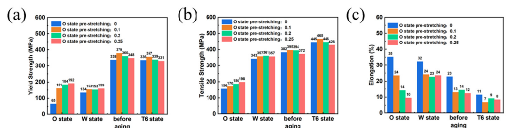
Figure 17. Tensile properties with W-state pre-strain of 0.10 under different O-state pre-strain levels at room temperature of the samples after heat treatment: (a) yield strength; (b) tensile strength; (c) elongation.
