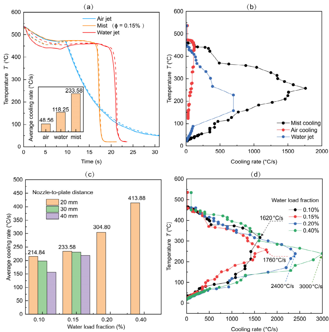
Figure 5. Temperature profile and cooling rate (a) T_1 (solid line) and T_2 (dashed line) evolution under different cooling media: air jet ( U_0 = 110\text{ m/s} ), mist ( U_0 = 110\text{ m/s} , \phi = 0.15\% ), water jet ( U_0 = 4.86\text{ m/s} ); (b) instantaneous cooling rate for different cooling media; (c) average cooling rate for different \phi and nozzle-to-plate distance; (d) instantaneous cooling rate for different \phi . The values shown represent average results from three repeated tests.
