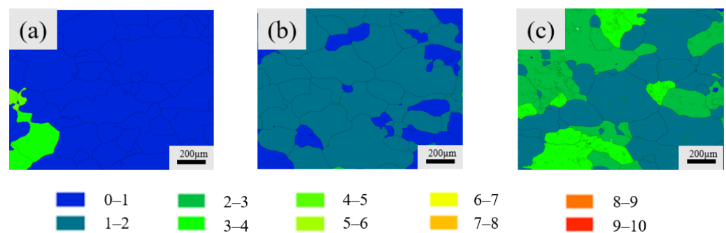
Figure 15. GOS under different W-state pre-strains: (a) W-state pre-strain: 0; (b) W-state pre-strain: 0.05; (c) W-state pre-strain: 0.1.
