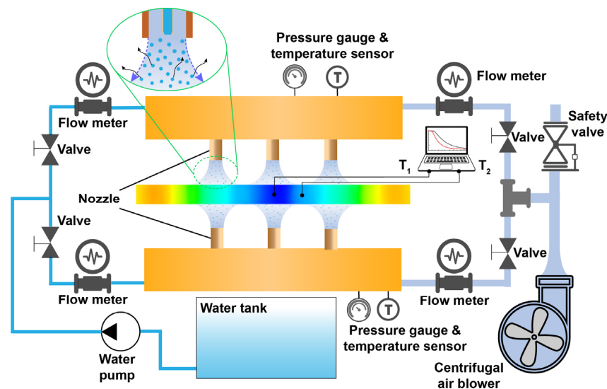
Figure 1. Schematic of the experimental system. The transfer apparatus, the furnace, and the intelligence system are not presented for better clarity.
