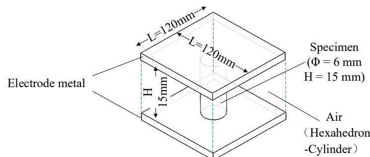
Figure 5. Schematic diagram of the specimen and air domain.
