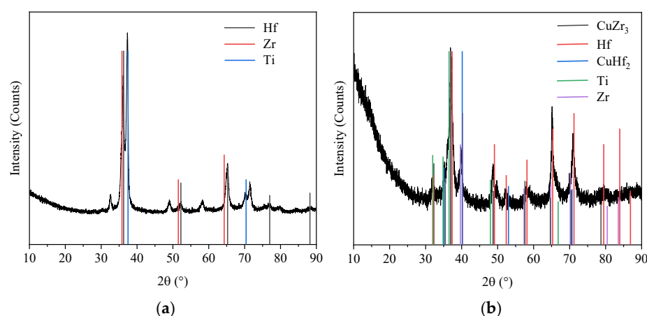
Figure 1. XRD analysis results and typical phase analysis results of the original specimens: (a) TiZrHf; (b) TiZrHfCu 0.8 .
