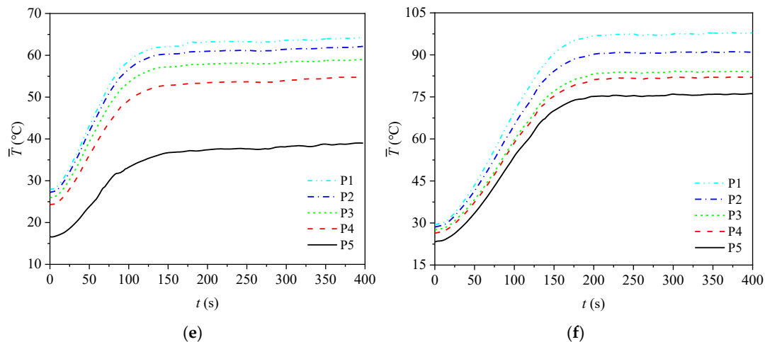
Figure 11. The \bar{T} time history of TiZrHf and TiZrHfCu 0.8 : (a) TiZrHf, 50 °C; (b) TiZrHf, 100 °C; (c) TiZrHf, 150 °C; (d) TiZrHfCu 0.8 , 50 °C; (e) TiZrHfCu 0.8 , 100 °C; (f) TiZrHfCu 0.8 , 150 °C.
