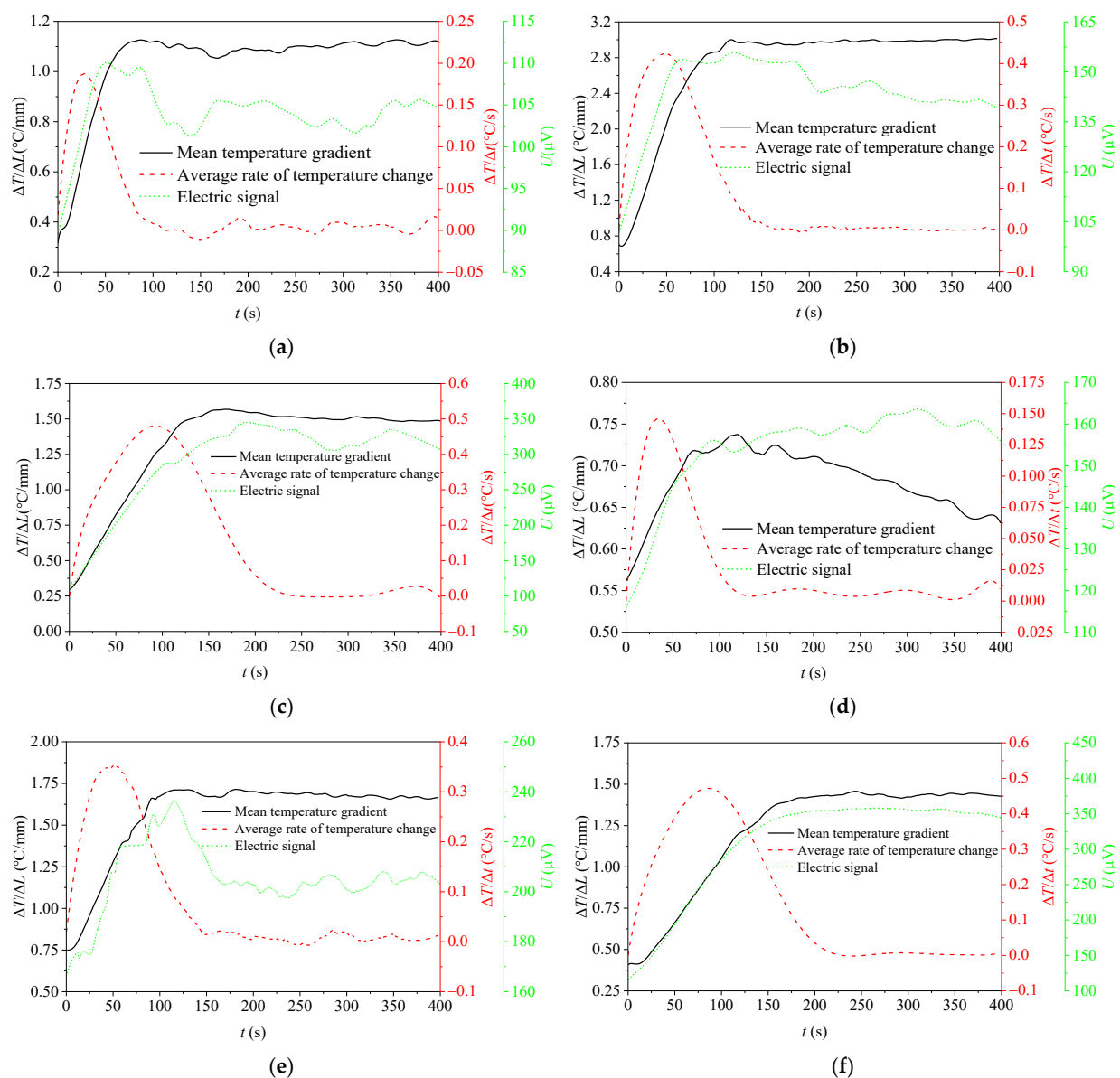
Figure 12. The relationship between U and T of TiZrHf and TiZrHfCu 0.8 : (a) TiZrHf, 50 °C; (b) TiZrHf, 100 °C; (c) TiZrHf, 150 °C; (d) TiZrHfCu 0.8 , 50 °C; (e) TiZrHfCu 0.8 , 100 °C; (f) TiZrHfCu 0.8 , 150 °C.
