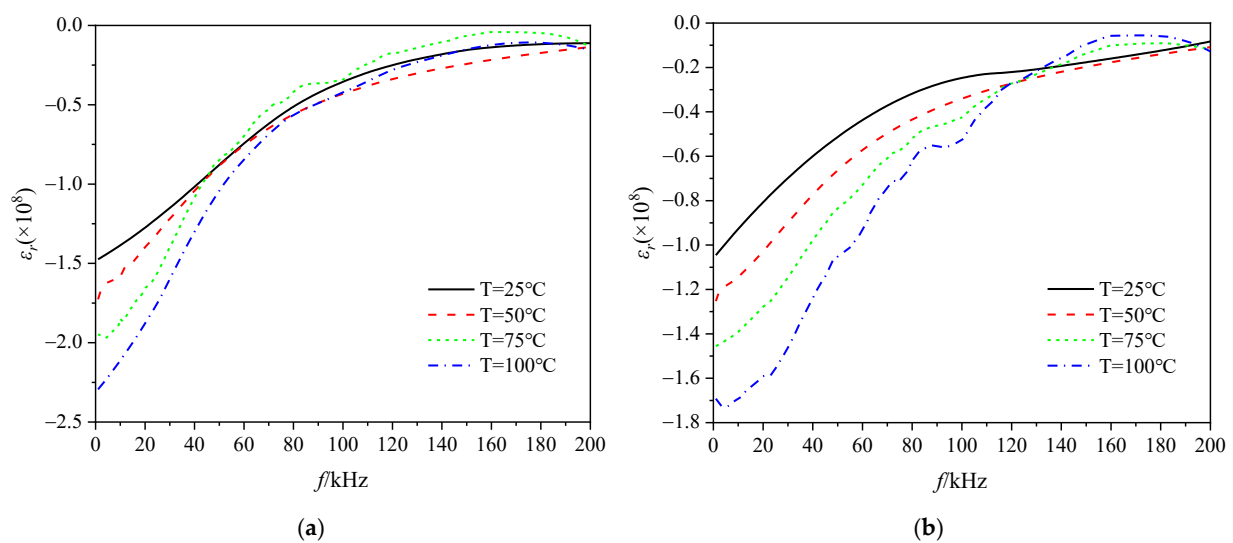
Figure 7. \epsilon_r of TiZrHf under different T and \sigma : (a) 0 MPa; (b) 300 MPa; (c) 600 MPa; (d) 900 MPa.
