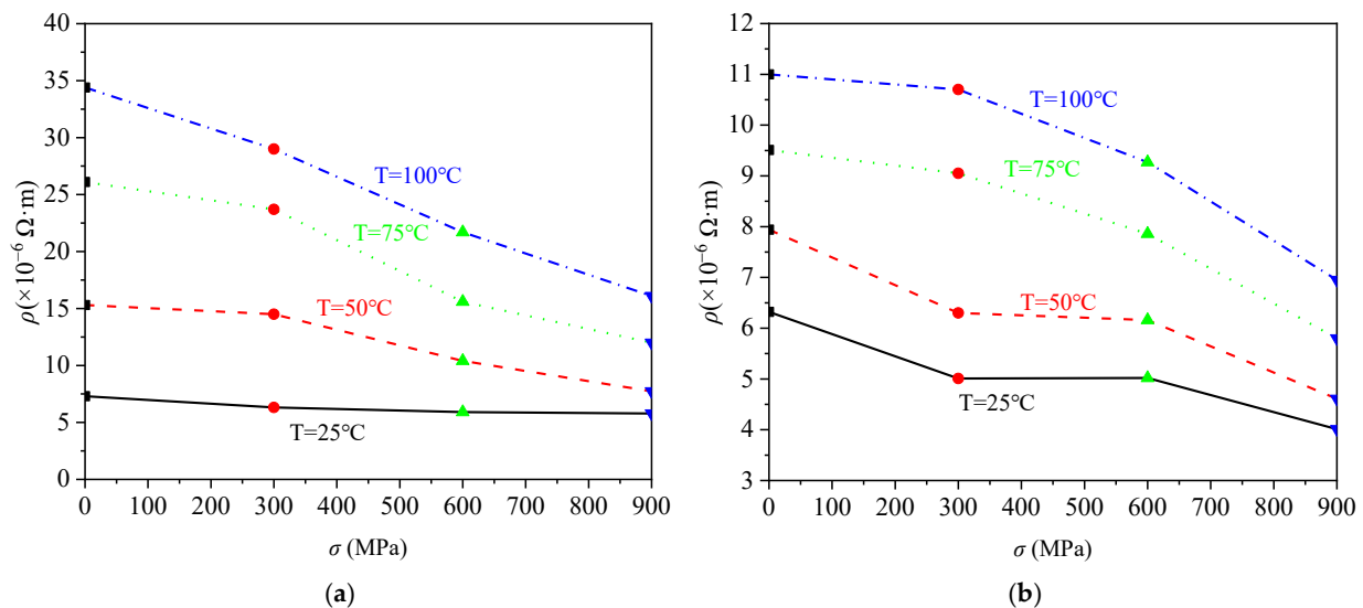
Figure 6. The modified resistivities of TiZrHf and TiZrHfCu 0.8 : (a) TiZrHf; (b) TiZrHfCu 0.8 .
