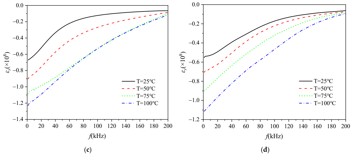
Figure 8. \varepsilon_r of TiZrHfCu 0.8 under different T and \sigma : (a) 0 MPa; (b) 300 MPa; (c) 600 MPa; (d) 900 MPa.
