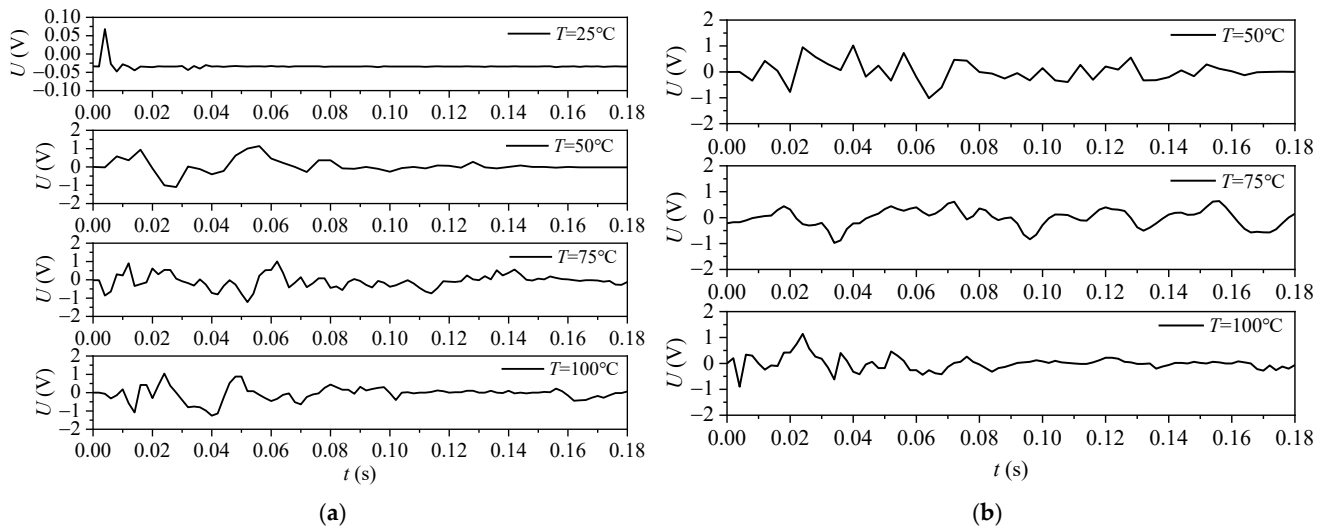
Figure 4. Compressive fracture—induced electrical signals under different T : (a) TiZrHf; (b) TiZrHfCu 0.8 .
