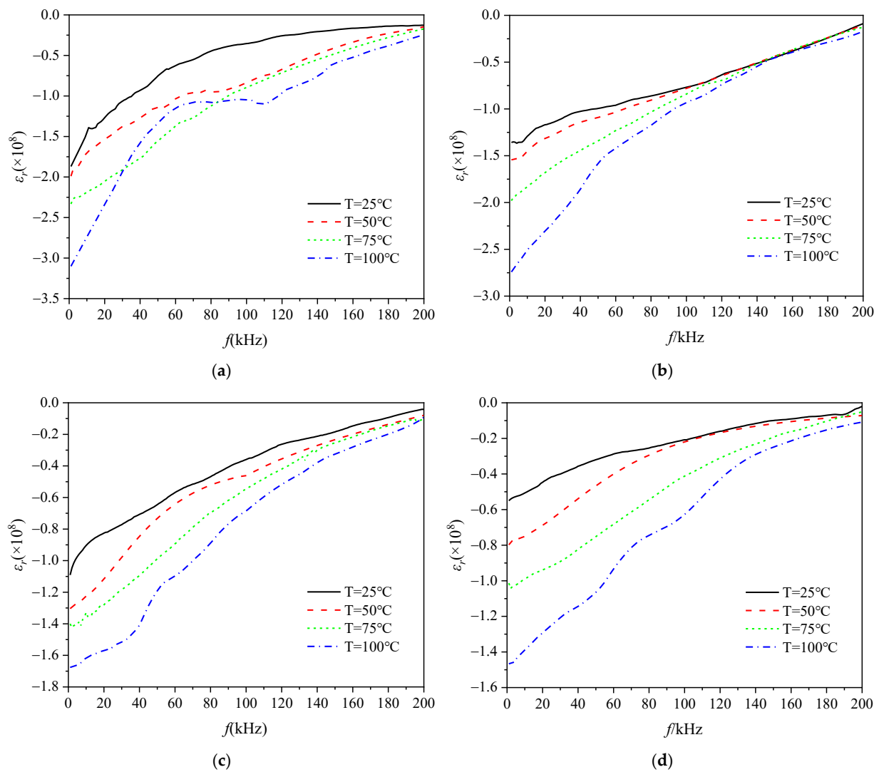
Figure 7. \epsilon_r of TiZrHf under different T and \sigma : (a) 0 MPa; (b) 300 MPa; (c) 600 MPa; (d) 900 MPa.
