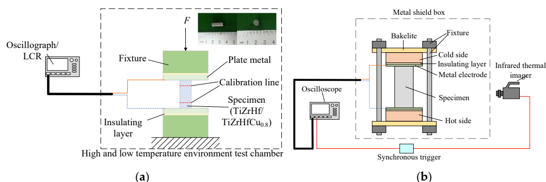
Figure 2. Experimental systems: (a) High temperature quasi—static compression and electrical parameter measurement; (b) Thermoelectricity measurement.
