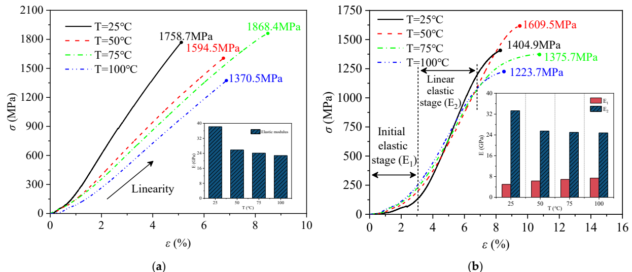
Figure 3. \sigma – \varepsilon curves of specimens at different T : (a) TiZrHf; (b) TiZrHfCu 0.8 .
