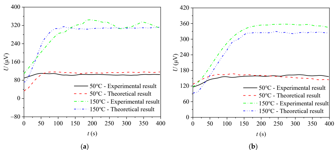
Figure 15. Comparison between the thermoelectric experimental results and the theoretical results: (a) TiZrHf; (b) TiZrHfCu 0.8 .
