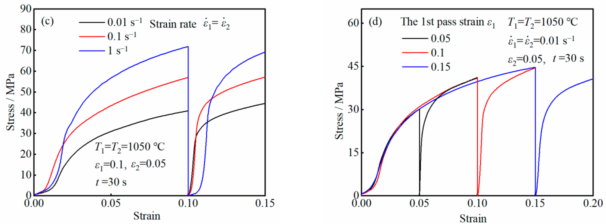
Figure 2. The stress–strain curve of double-pass hot compression under different deformation process parameters: (a) inter-pass time, (b) deformation temperature, (c) strain rate, and (d) the first-pass strain.
