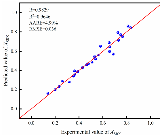
Figure 6. Comparison of X_{SRX} predicted values and experimental values under all deformation conditions and model accuracy indicators.
