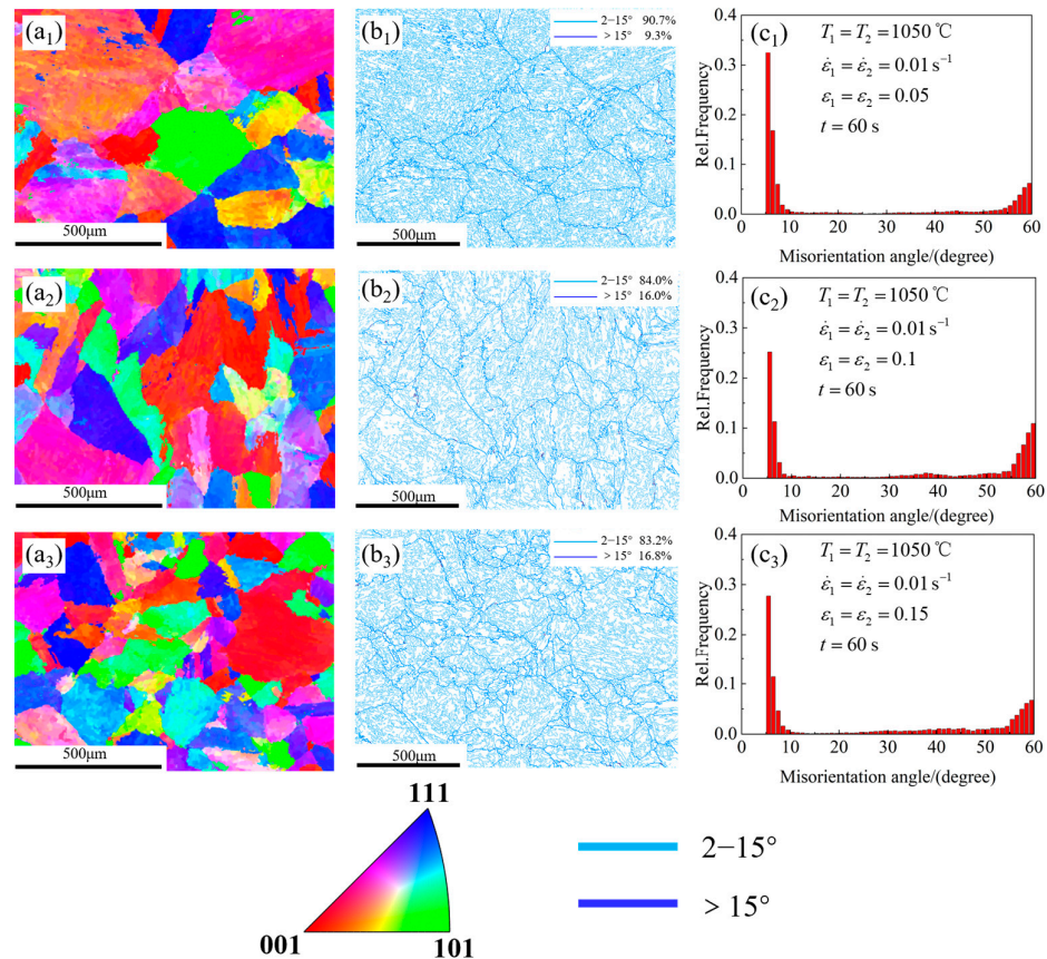
Figure 9. The EBSD characterization of SA-508M Gr.3 steel after the double-pass hot compression with the first-pass strains of 0.05 ( a1 , b1 , c1 ), 0.1 ( a2 , b2 , c2 ), and 0.15 ( a3 , b3 , c3 ). ( a1–a3 ) IPF after parent phase reconstruction, ( b1–b3 ) BC (backscattered electron contrast) + GBs (grain boundaries), and ( c1–c3 ) orientation difference distribution diagram.
