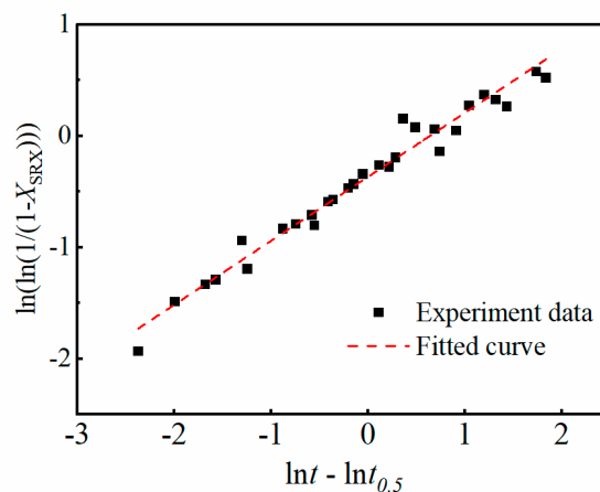
Figure 4. The fitted line of (\ln t - \ln t_{0.5}) and \ln\{\ln[1/(1-X_{SRX})]\} .
