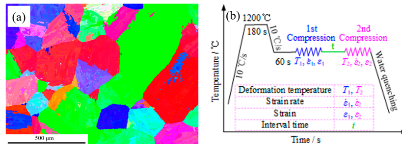
Figure 1. The double-pass hot compression experiment: (a) the IPF diagram of the sample before compression, (b) the schematic diagram of the experimental process.
