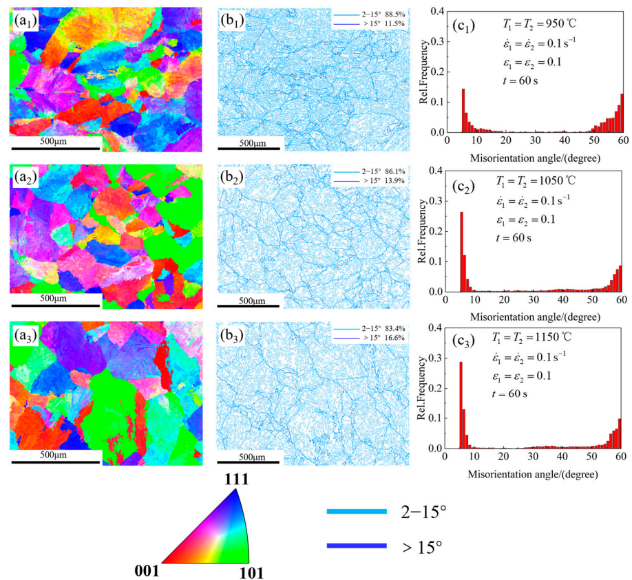
Figure 7. The EBSD characterization of SA-508M Gr.3 steel after the double-pass hot compression under deformation temperatures of 950 °C (a 1 ,b 1 ,c 1 ), 1050 °C (a 2 ,b 2 ,c 2 ), and 1150 °C (a 3 ,b 3 ,c 3 ). (a 1 –a 3 ) IPF after parent phase reconstruction, (b 1 –b 3 ) BC (backscattered electron contrast) + GBs (grain boundaries), and (c 1 –c 3 ) orientation difference distribution diagram.
