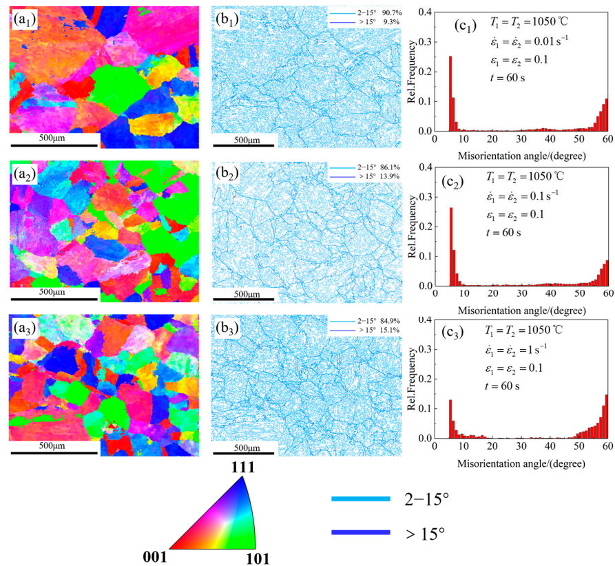
Figure 8. The EBSD characterization of SA-508M Gr.3 steel after the double-pass hot compression at strain rates of 0.01 s -1 (a 1 , b 1 , c 1 ), 0.1 s -1 (a 2 , b 2 , c 2 ), and 1 s -1 (a 3 , b 3 , c 3 ). (a 1 –a 3 ) IPF after parent phase reconstruction, (b 1 –b 3 ) BC (backscattered electron contrast) + GBs (grain boundaries), and (c 1 –c 3 ) orientation difference distribution diagram.
