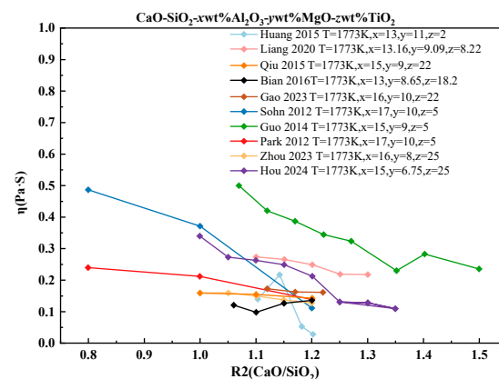
Figure 9. Effect of basicity (CaO/SiO 2 ) on viscosity Adapted from Refs. [45,47–50,55–57,60,62].
