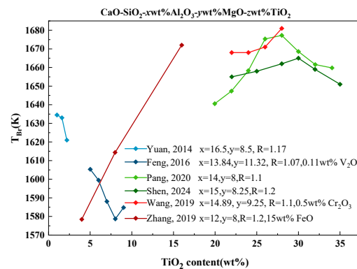
Figure 3. Effect of TiO_2 content on T_{Br} Adapted from Refs. [14,15,39–43].
