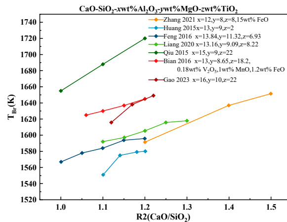
Figure 5. Effect of basicity (CaO/SiO 2 ) on T Br Adapted from Refs. [43,45–50].
