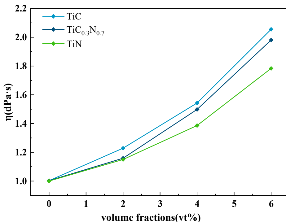
Figure 11. Effects of \text{TiC} , \text{TiN} and \text{Ti}(\text{C}_x\text{N}_y) with different volume fractions on slag viscosity.
