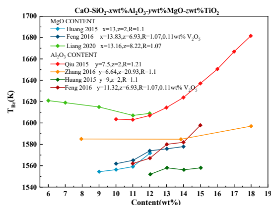
Figure 4. Effect of MgO and Al_2O_3 content on T_{Br} Adapted from Refs. [24,37,40,45–47].
