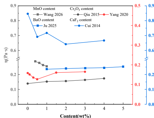
Figure 10. The influence of trace components on the viscosity of slag Adapted from Refs. [15,48,54,58,65].
