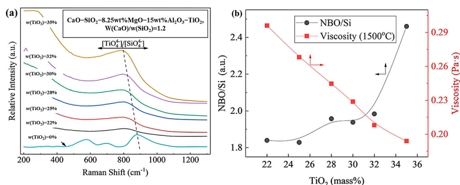
Figure 13. (a) Raman spectra of the \text{CaO-SiO}_2\text{-MgO-Al}_2\text{O}_3\text{-TiO}_2 slag with different \text{TiO}_2 contents; (b) effect of \text{TiO}_2 content on the value of NBO/Si and the viscosity of slag at 1500\text{ }^\circ\text{C} [42]. (Reprinted with permission from Ref. [42]. 2024, Elsevier).
