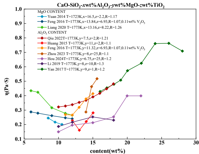
Figure 8. Effect of MgO and Al 2 O 3 content on viscosity Adapted from Refs. [24,39,40,45–47,60,62–64].
