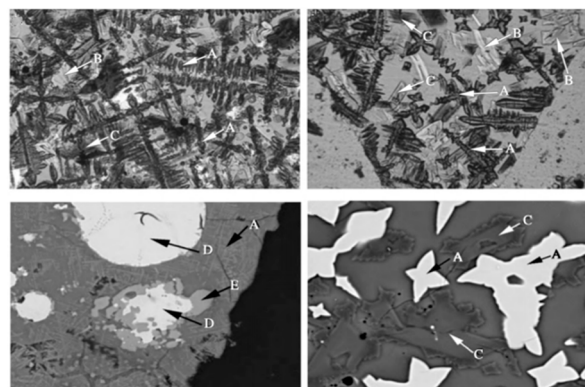
Figure 2. Microstructural morphology of TBFS from a certain steel plant. The figure represent different regions of one sample and are intended to illustrate the types of phases present in the sample. (A) perovskite. (B) Clinocllore Diopside. (C) Titanium-rich diopside. (D) metallic iron. (E): TiC. (Reprinted with permission from Ref. [20]. 2017, Metallurgical Analysis).
