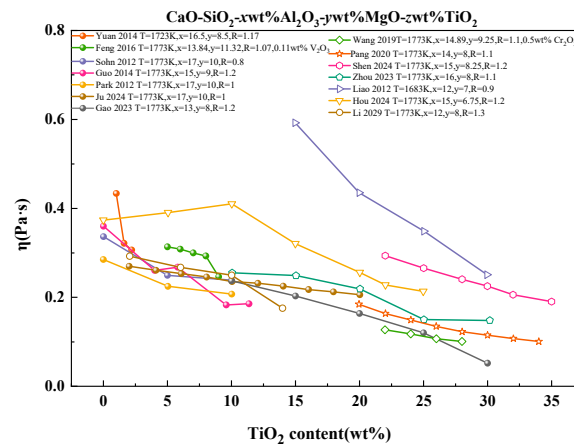
Figure 7. Effect of TiO 2 content on viscosity Adapted from Refs. [14,15,39,41,42,55–63].
