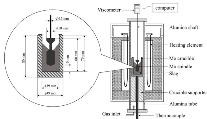
Figure 6. Schematic diagram for the viscosity measurement and dimension of the spindle (Re-printed with permission from Ref. [42], 2024, Elsevier).
