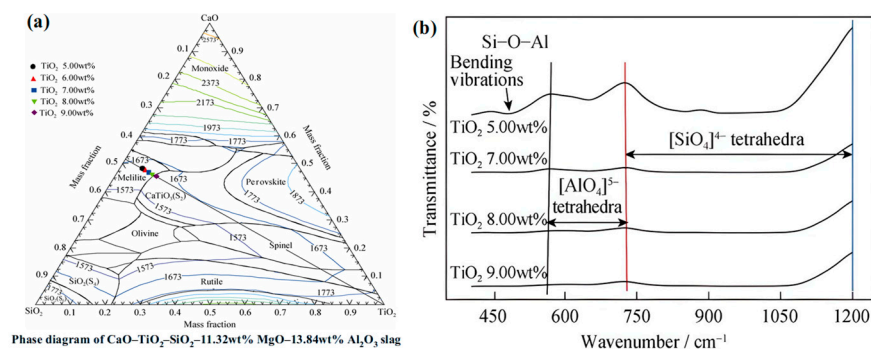
Figure 12. (a) Phase diagrams of five-component slag system under different conditions—CaO–TiO 2 –SiO 2 –11.32 wt% MgO–13.84 wt% Al 2 O 3 [40]; (b) FTIR spectra of slags with different TiO 2 contents [40]. (Reprinted with permission from Ref. [40], 2016, Springer Nature).
