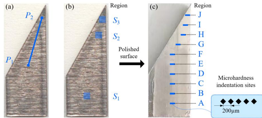
Figure 7. Schematic of the designated regions for evaluating the surface quality of LPBF specimens: (a) line roughness, (b) surface topography, and (c) microhardness.
