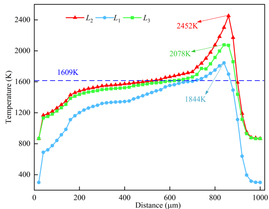
Figure 3. Spatial temperature distribution profiles extracted along a longitudinal isoelevation line near the melt pool centers. The three curves correspond to the specific thermal states depicted in the side views of Figure 2c, 2f, and 2i, respectively.
