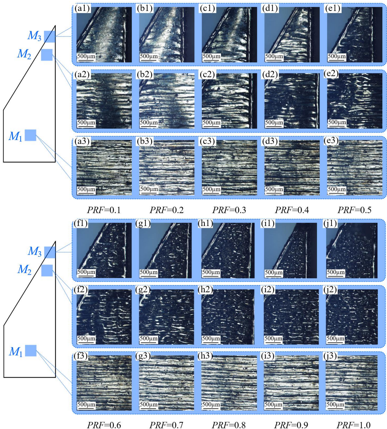
Figure 11. Ultra-depth-of-field magnified morphologies of different regions on the X-Y plane for specimens fabricated with \text{PRF} values ranging from 0.1 to 1.0. Panels (a1–j3) correspond to \text{PRF} =
