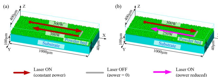
Figure 1. Schematic of the multiphysics thermal simulation: (a) control group utilizing constant laser power for both consecutive tracks; (b) optimized group implementing active energy modulation with reduced laser power for the second adjacent track.
