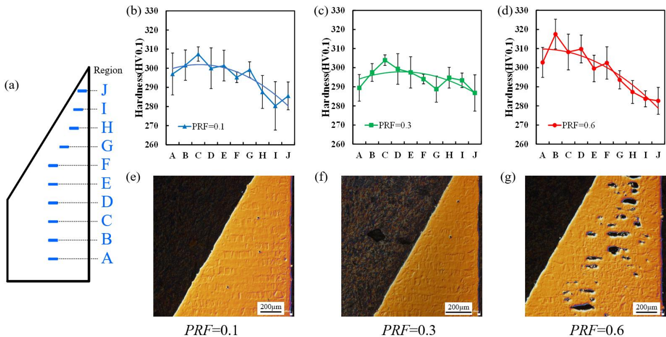
Figure 13. Microhardness distribution and polished surface morphologies of the fabricated specimens: (a) designated regions for microhardness profiling; (b–d) spatial hardness distribution curves measured within the highlighted region for PRF values of 0.1, 0.3, and 0.6, respectively; (e–g) macroscopic morphologies of the top surfaces after polishing.
