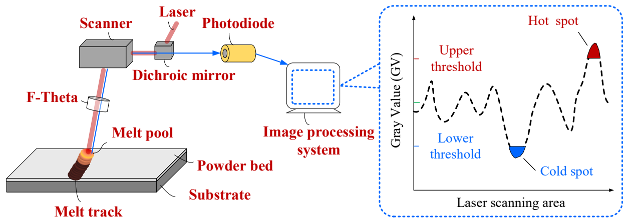
Figure 5. Configuration of the LPBF system and optical monitoring system.
