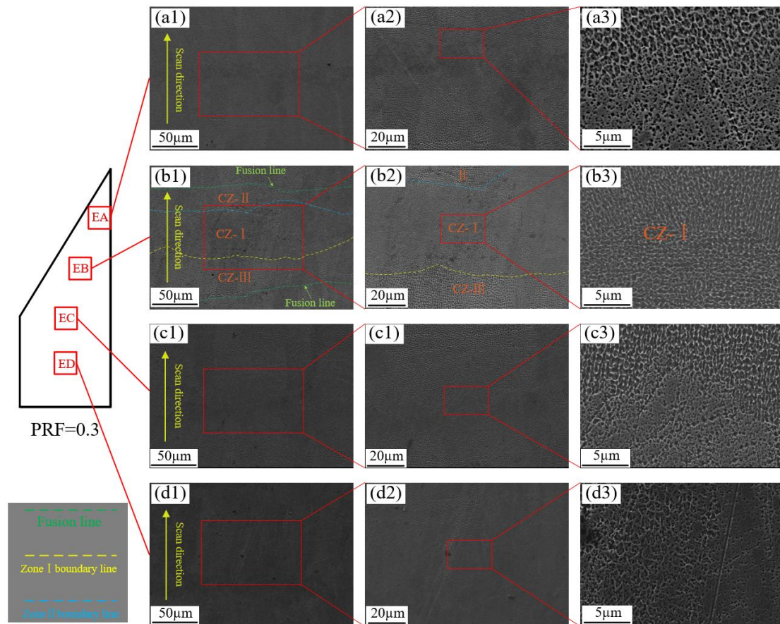
Figure 15. SEM micrographs of the cellular dendritic substructures on the X–Y plane of the specimen fabricated with PRF = 0.3 : (a1–d3) correspond to four representative sampling regions, EA, EB, EC, and ED, along the sharp-edged geometry. The numbered subpanels in each group show enlarged views of individual melt tracks and their internal cellular features.
