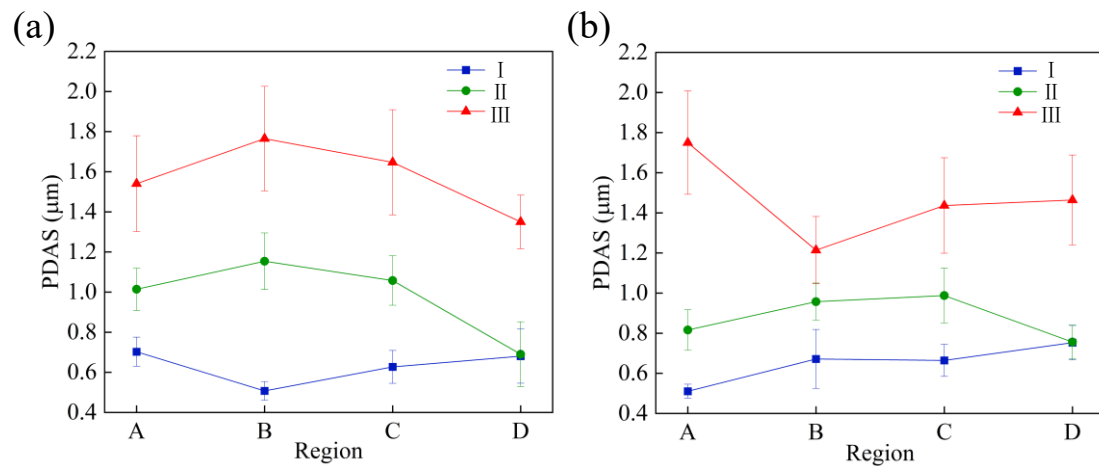
Figure 16. PDAS evolution under PRF-based active energy modulation: (a) PDAS statistics of cellular Regions CZ-I–CZ-III at sampling locations A–D for the specimen fabricated with PRF = 0.1; (b) corresponding PDAS statistics for PRF = 0.3.
