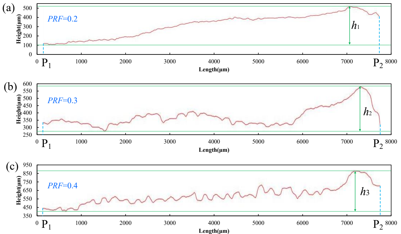
Figure 12. Cross-sectional height profiles along line P_1P_2 at the apical region for evaluating the line roughness ( R_a ): (a) PRF = 0.2 , (b) PRF = 0.3 , and (c) PRF = 0.4 .
