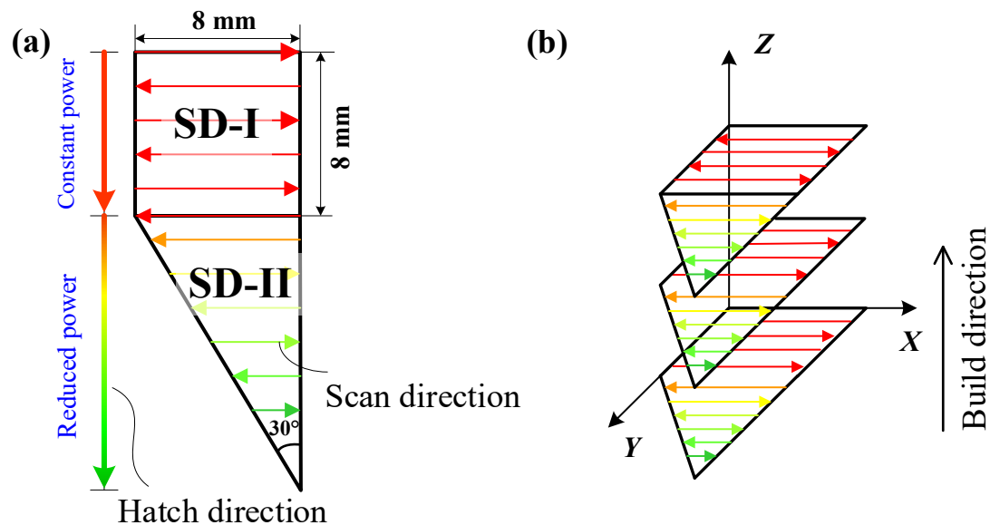
Figure 6. Schematic of the experimental specimen geometry and laser scanning strategy: (a) top view illustrating the dimensions, scanning path, and the structural division; (b) illustration of the build direction. Different colors schematically represent different laser powers..
