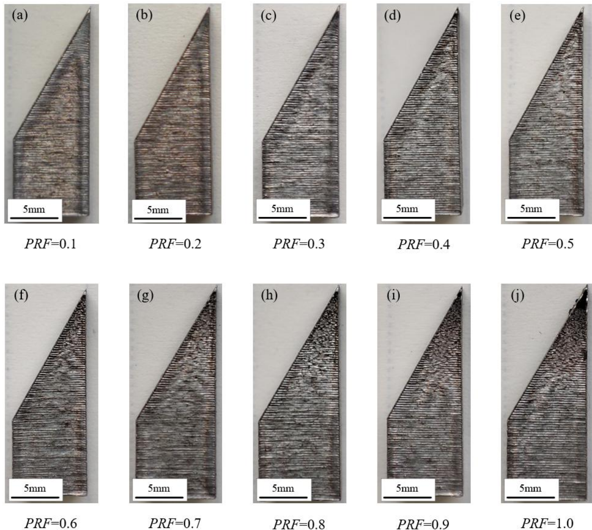
Figure 10. Panoramic top-surface morphologies of all 10 fabricated specimens: (a–j) specimens corresponding to PRF values ranging from 0.1 to 1.0, respectively.
