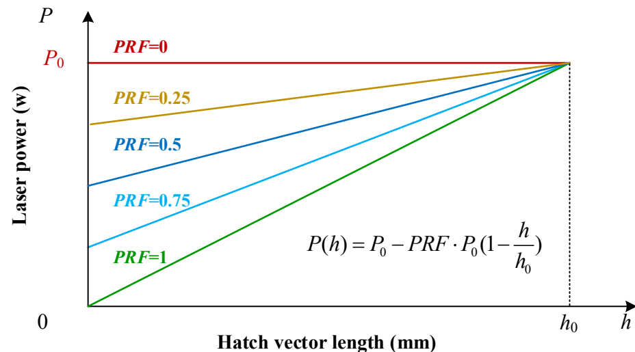
Figure 4. Linear correlation between dynamically modulated laser power and scanning vector length under varying PRF values. The distinct slopes illustrate the specifically controlled gradients of power reduction, ranging from constant power ( PRF = 0 ) to complete decay ( PRF = 1.0 ), aimed at achieving localized thermal balance in sharp corner regions.
