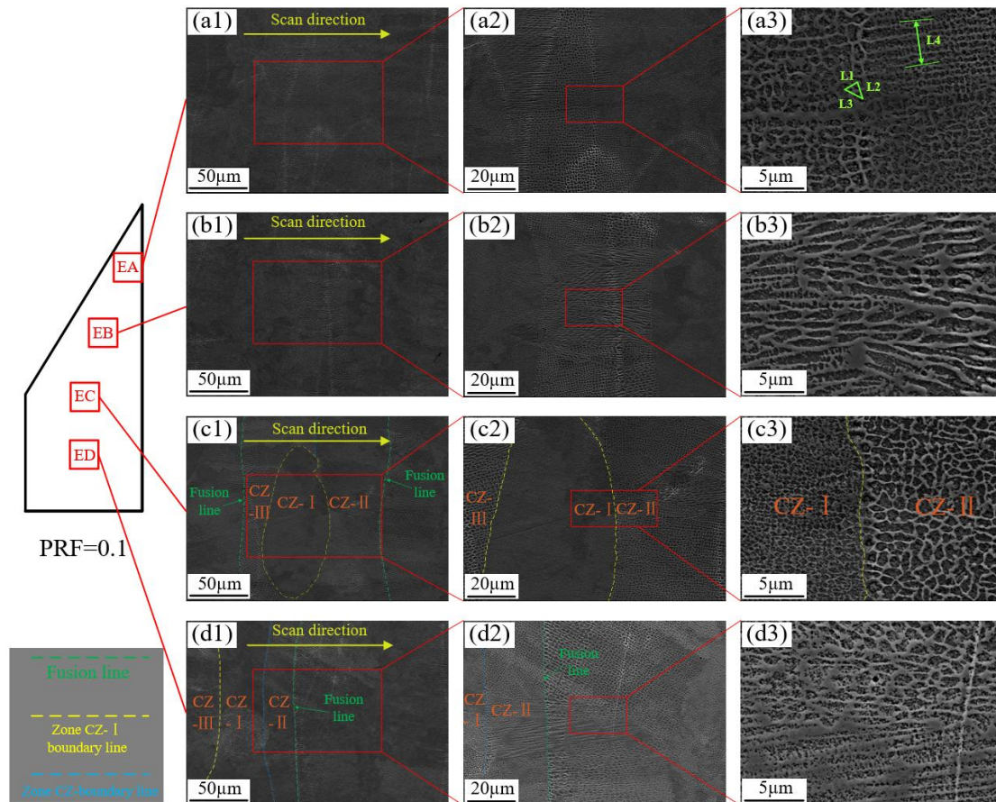
Figure 14. SEM micrographs of the cellular dendritic substructures on the X–Y plane of the specimen fabricated with PRF = 0.1 : (a1–d3) correspond to four representative sampling regions, EA, EB, EC, and ED, along the sharp-edged geometry. The numbered subpanels in each group show enlarged views of individual melt tracks and their internal cellular features.
