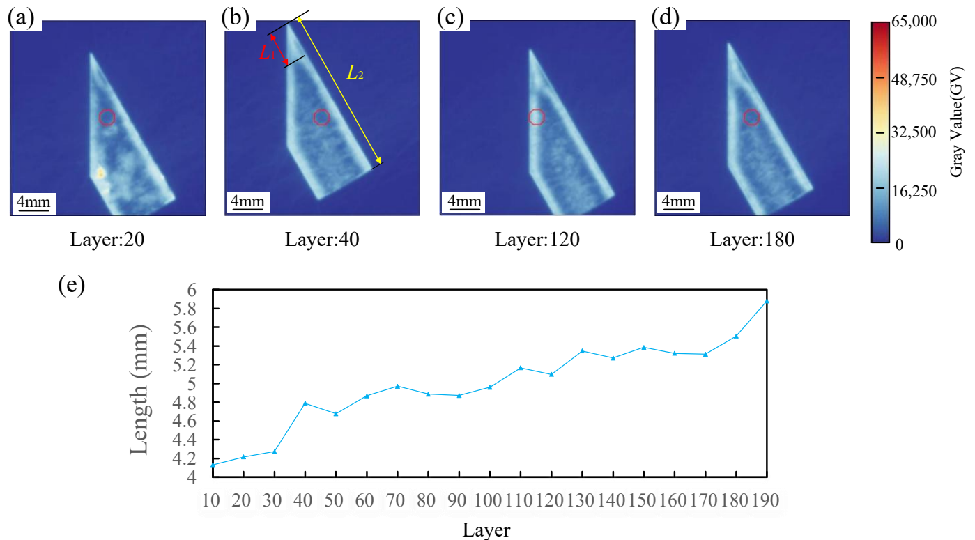
Figure 8. In situ monitoring of the heat-accumulation evolution for the PRF = 0.1 specimen: (a–d) grayscale monitoring images of four representative layers; (e) evolution of the axial extent L_1 of the connected apical high-intensity region with build layer number.
