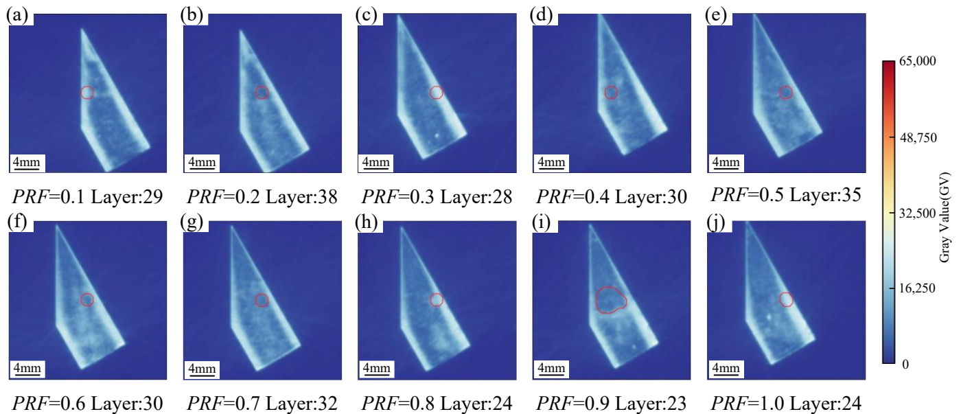
Figure 9. Comparative in situ monitoring images of layers across specimens fabricated with different PRF gradients: (a–j) grayscale maps corresponding to PRF values ranging from 0.1 to 1.0, respectively.
