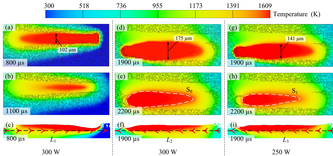
Figure 2. Simulated temporal evolution of melt pool morphologies and temperature distributions under distinct power inputs: (a–c) the first track (300 W), showing top views at the end of active scanning (800 \mu s, (a)) and during the cooling stage (1100 \mu s, (b)), alongside a side view at 800 \mu s (c); (d–f) the second track without power modulation (control group, 300 W), showing top views at the end of scanning (1900 \mu s, (d)) and during cooling (2200 \mu s, (e)), alongside a side view at 1900 \mu s (f); (g–i) the second track with active energy modulation (optimized group, 250 W), showing top views at the end of scanning (1900 \mu s, (g)) and during cooling (2200 \mu s, (h)), alongside a side view at 1900 \mu s (i). The arrows on the dashed lines in (c,f,i) indicate the temperature-profile extraction directions used in Figure 3. The upper limit of the temperature scale was fixed at the liquidus temperature of Inconel 718 (1609 K); therefore, red regions represent saturated high-temperature regions close to or above the liquidus temperature rather than exact quantitative melt pool boundaries.
