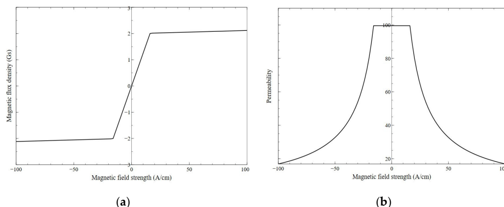
Figure 5. Electromagnetic properties of 42CrMo4: (a) B-H curve of 42CrMo4; (b) permeability of 42CrMo4.
