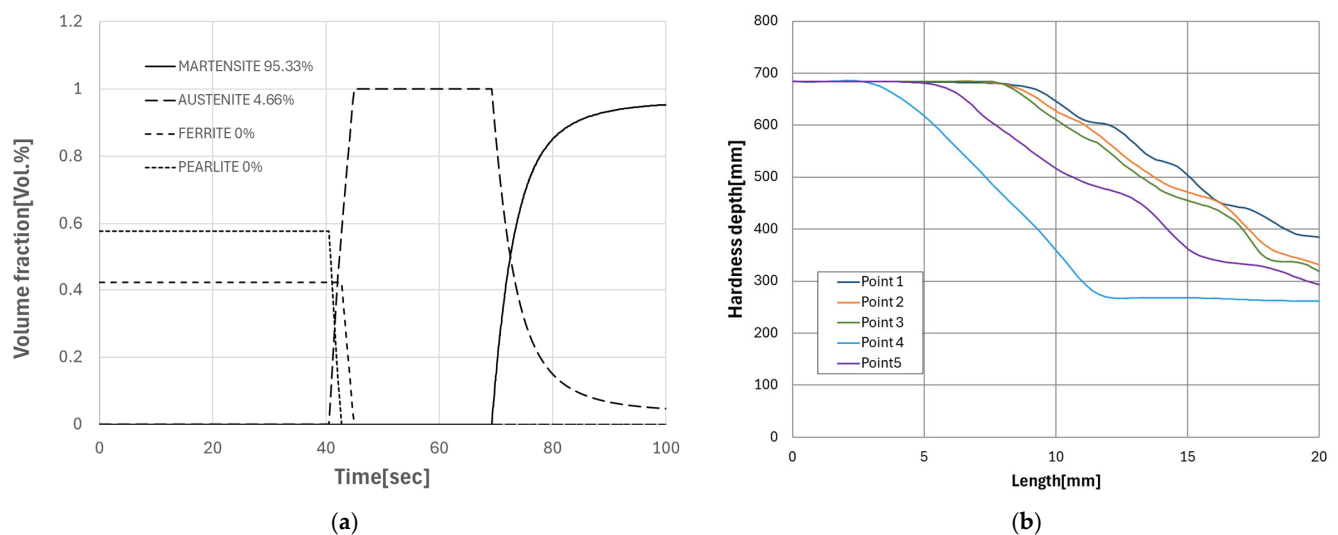
Figure 12. Finite element analysis results for microstructure fraction and hardness: (a) microstructure fraction of position 4; (b) hardness distribution with depth at each position.
