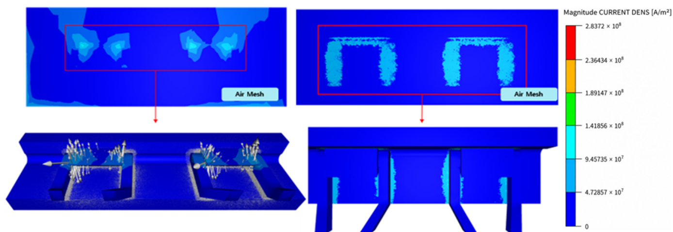
Figure 7. Magnetic flux distribution in the induction heating analysis.
