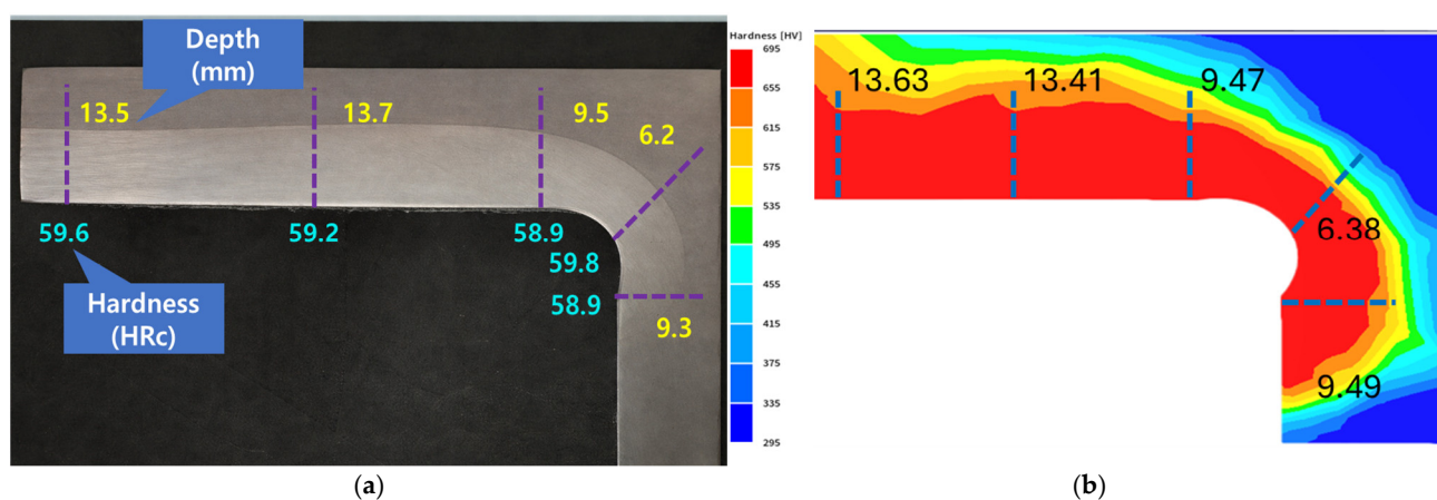
Figure 14. Comparison of measured data and finite element analysis: (a) induction heating image provided by the bearing manufacturer; (b) results of finite element analysis based on DNN training.
