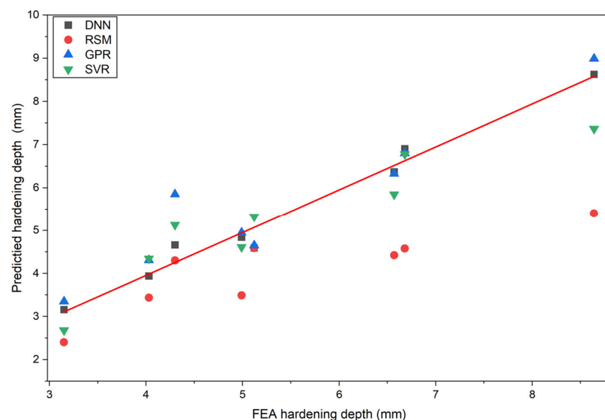
Figure 10. Parity plot comparing the FEA-calculated and surrogate-model-predicted hardening depths at position 4. The diagonal line represents perfect agreement. ( y = x ).
