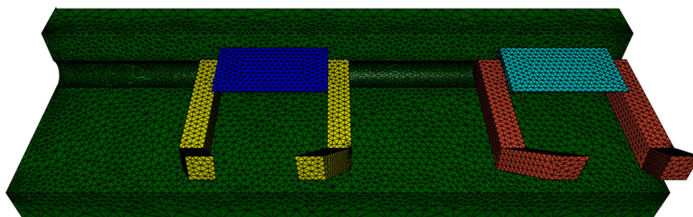
Figure 4. Three-dimensional mesh configuration of the dual-inductor heating model.
