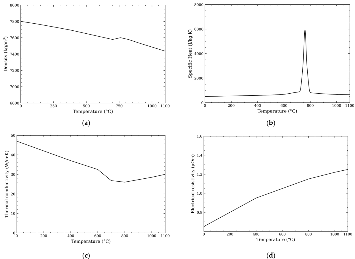
Figure 6. Temperature-dependent thermophysical and electrical properties: (a) density changes with temperature; (b) specific heat changes with temperature; (c) thermal conductivity changes with temperature; and (d) electrical resistivity with temperature.
