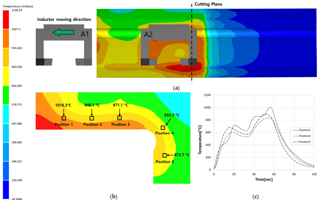
Figure 11. Finite element analysis results for induction hardening conditions selected using a surrogate model: (a) 3D induction heating analysis results and cutting position; (b) temperature distribution of section plane; and (c) time-dependent temperature variations at different locations during heating and cooling.
