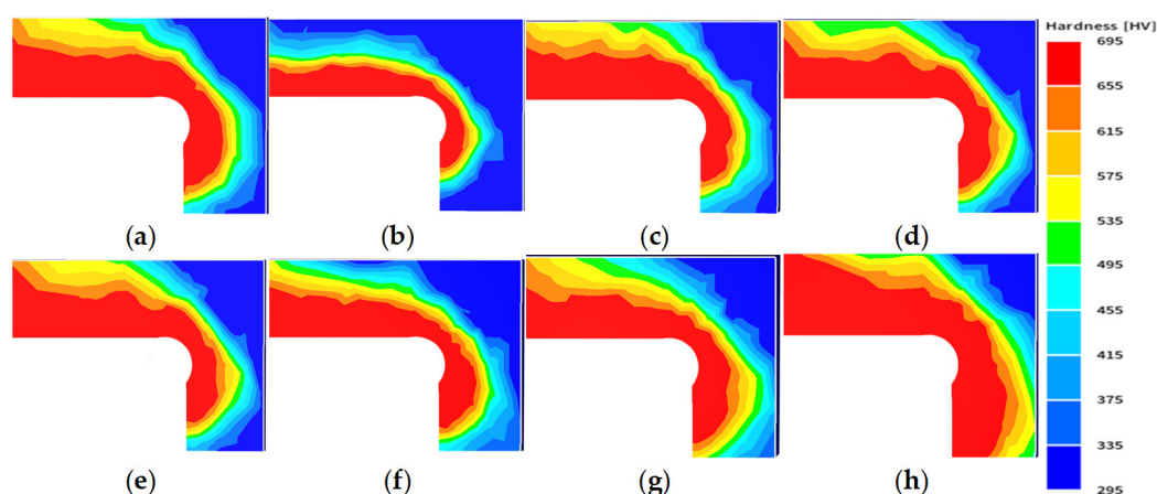
Figure 9. Hardness distribution after induction hardening calculated by FEA: (a) 3-8000-8000; (b) 4-7000-7000; (c) 4-7000-8000; (d) 4-7000-9000; (e) 4-8000-8000; (f) 5-9000-7000; (g) 5-9000-8000; and (h) 5-9000-9000.
