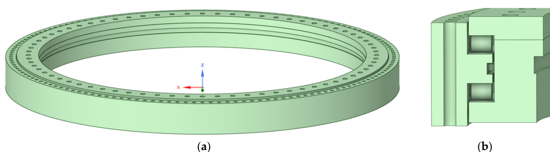
Figure 1. Pitch bearing geometry in wind turbine generators: (a) overall geometry of wind turbine bearing; (b) cross-sectional geometry.
