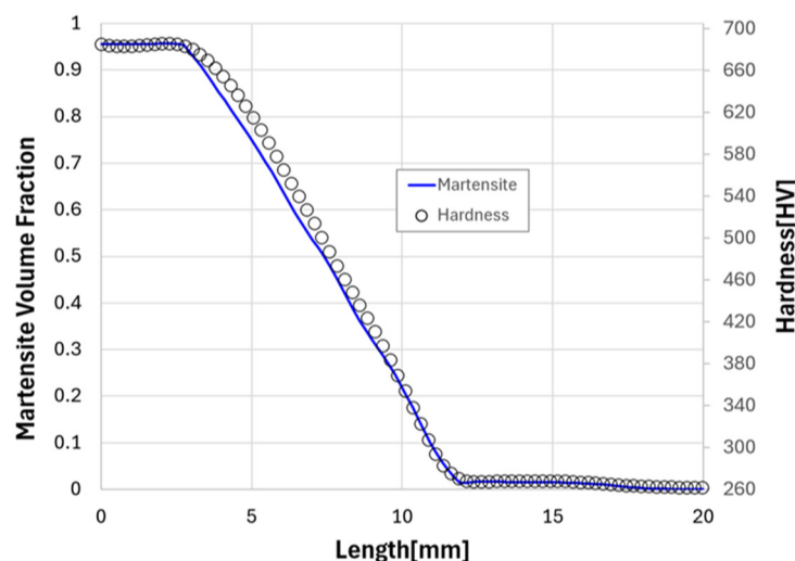
Figure 13. Hardness and martensite fraction profiles as a function of depth from the surface calculated by finite element analysis.
