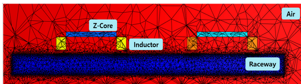
Figure 3. Cross-sectional mesh configuration of the electromagnetic computation model.
