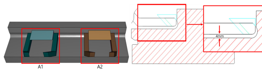
Figure 2. Arrangement of dual inductor position and air gap.
