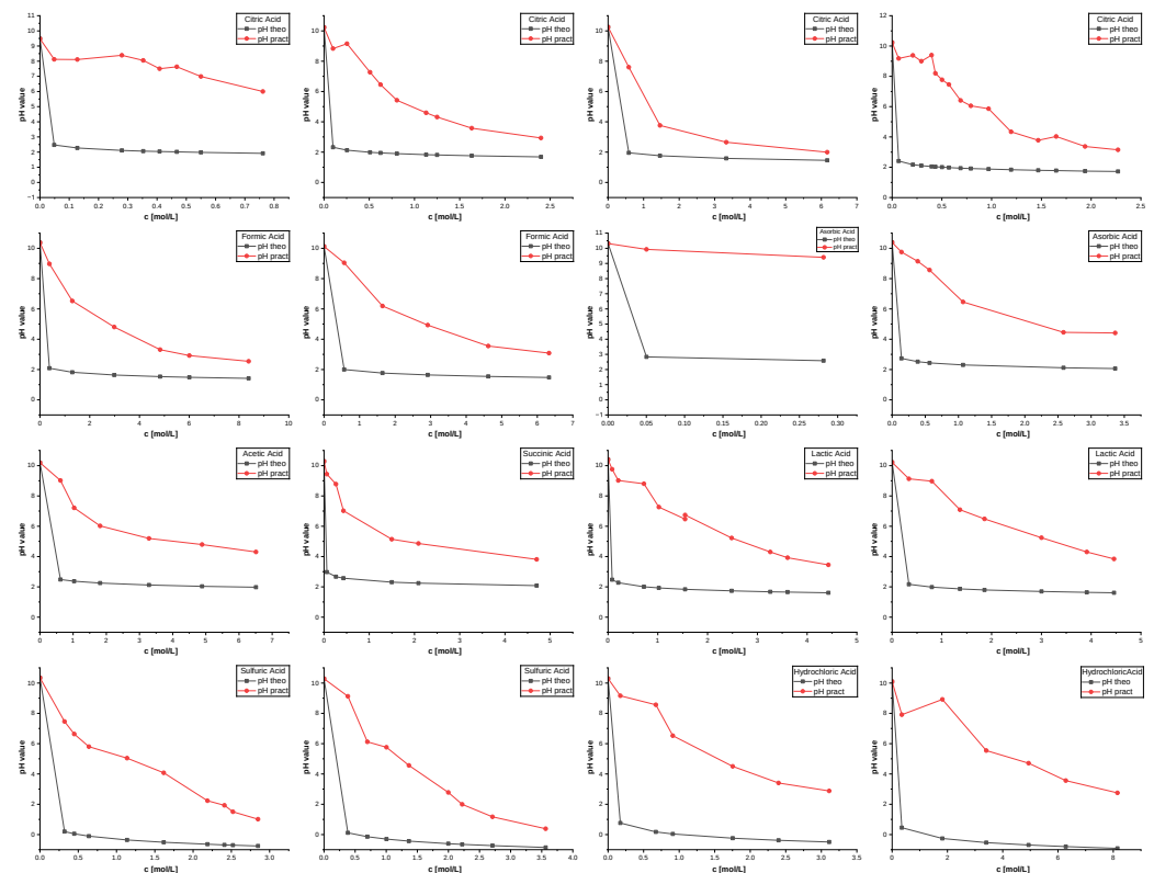
Figure A2. The red lines with spherical points show measured pH values, and black lines with square points are the calculated pH values, based on Formulae (1) and (2) and pK_a values from Table 2. On each subgraph is written which acid was used in the experiment.
