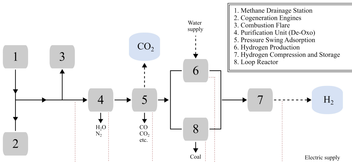
Figure 3. Example diagram of a hydrogen production installation.
