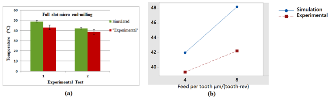
Figure 13. (a) Comparison of experimental and simulated maximum temperature distribution and (b) interaction plot of temperature distribution
