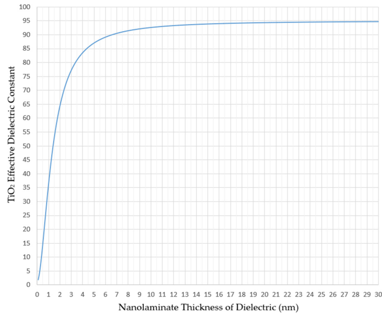
Figure 4. \kappa_A with respect to \text{TiO}_2 thickness calculated by Equation (2).
