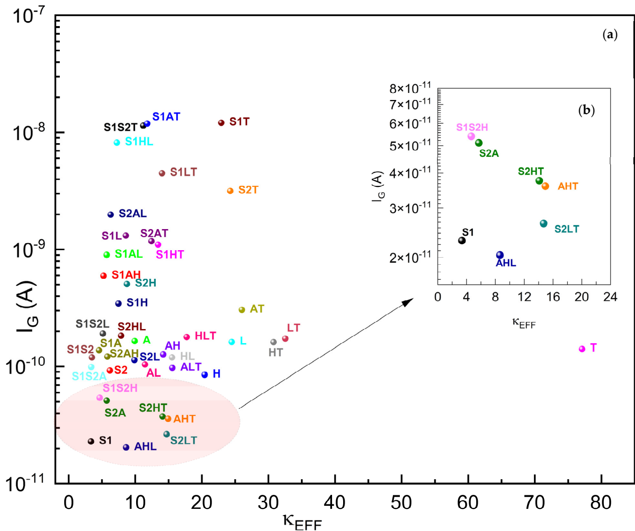
Figure 11. (a) I_G of g \kappa -FinFETs with single, two-stage, and three-stage \kappa -graded gate oxides, (b) I_G zoomed around \kappa_{\text{EFF}} = 0\sim 24 . See Table 9 for concise results.
