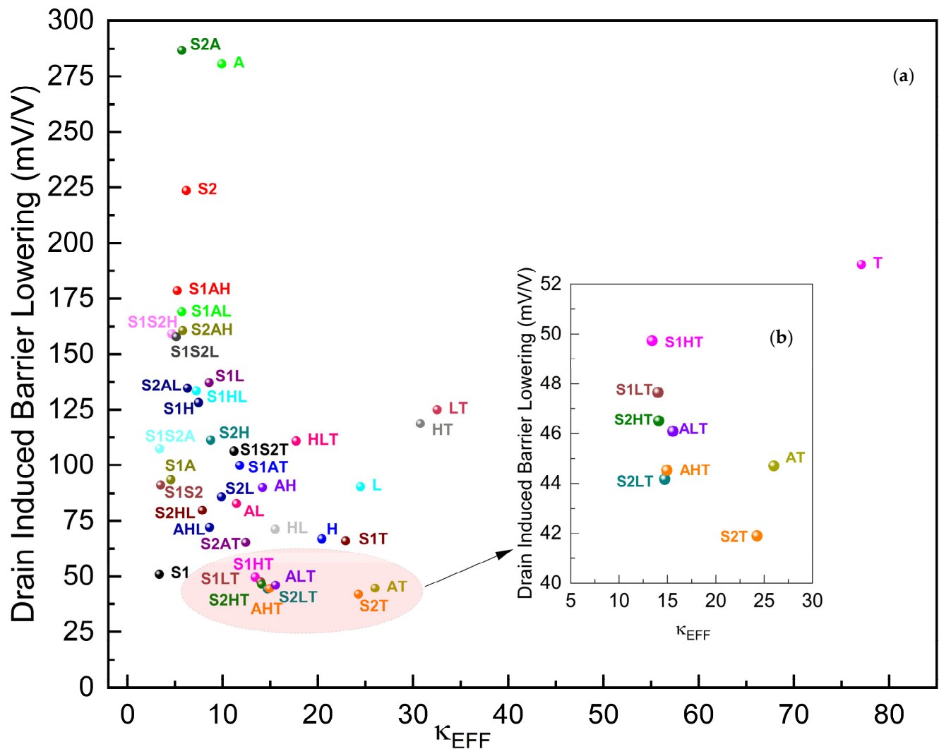
Figure 7. (a) DIBL of gκ-FinFETs with single, two-stage, and three-stage κ-graded gate oxides, (b) DIBL zoomed around \kappa_{\text{EFF}} = 5\sim 30 . See Table 5 for concise results.
