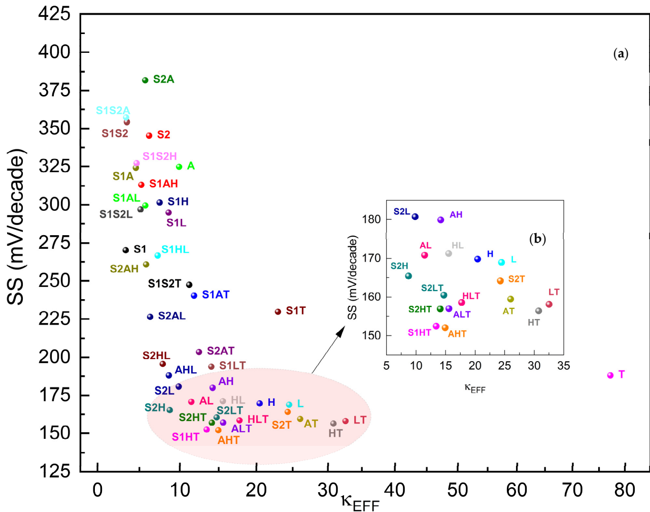
Figure 8. (a) SS of gκ-FinFETs with single, two-stage, and three-stage κ-graded gate oxides, (b) SS zoomed around \kappa_{\text{EFF}} = 5\sim 35 . See Table 6 for concise results.
