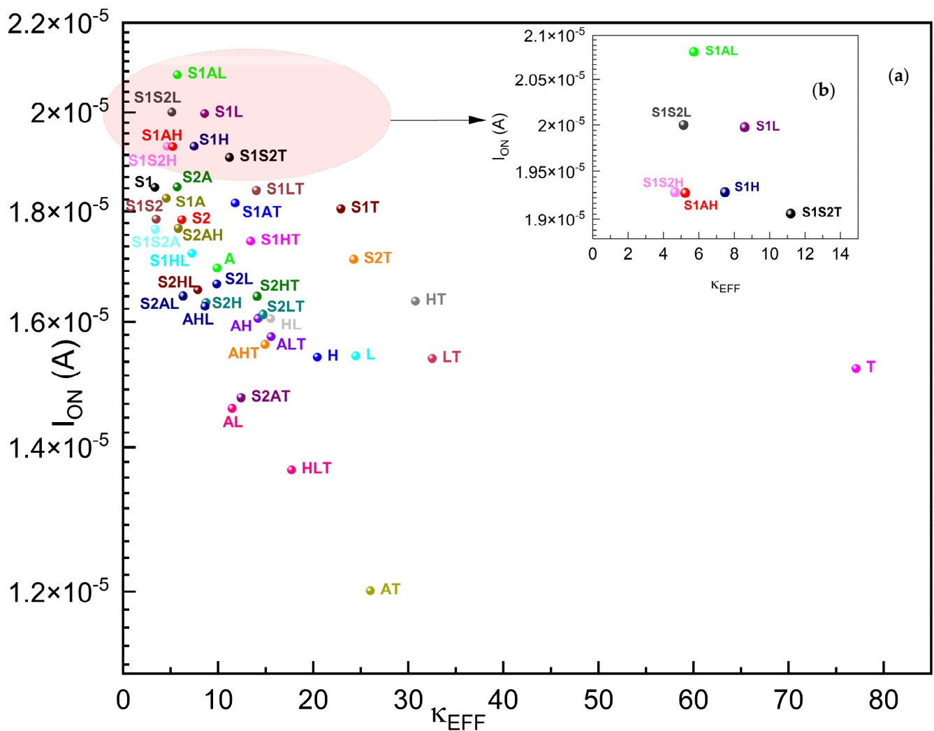
Figure 10. (a) I_{ON} of \gamma\kappa -FinFETs with single, two-stage, and three-stage \kappa -graded gate oxides, (b) I_{ON} zoomed around \kappa_{EFF} = 0 \sim 14 . See Table 8 for concise results.
