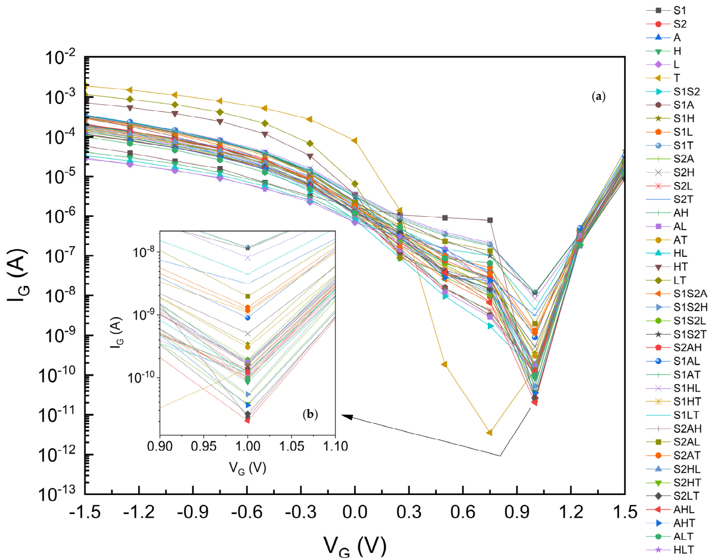
Figure 6. (a) Leakage Current I_G for gk-FinFETs with single, two-stage, and three-stage \kappa -graded gate oxides, (b) I_G zoomed for V_G between 0.90 and 1.1 V. See Tables 9 and 12 for summarized results of this figure.
