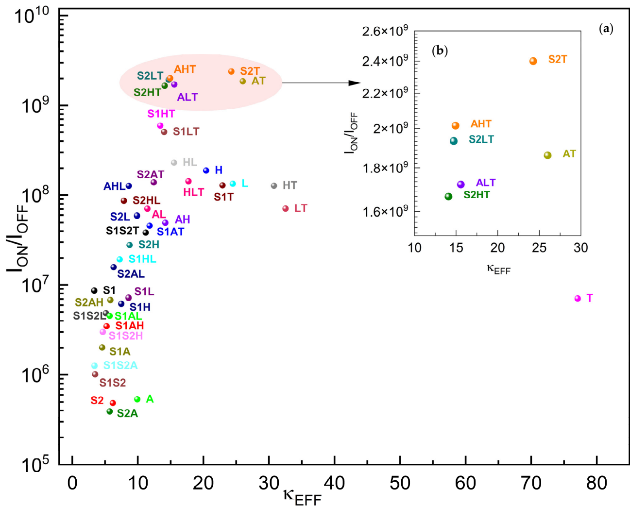
Figure 12. (a) I_{ON}/I_{OFF} of g \kappa -FinFETs with single, two-stage, and three-stage \kappa -graded gate oxides, (b) I_{ON}/I_{OFF} zoomed around \kappa_{EFF} = 10\sim 30 . Observe Table 10 for concise results.
