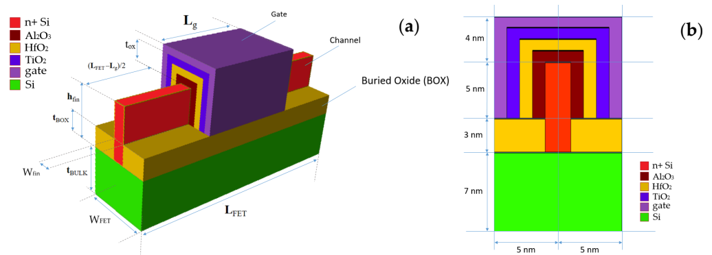
Figure 1. (a) gκ-FinFET geometric model with 3-stage κ-graded gate oxide with thickness t_{ox} , (b) inset of the cross-section, with geometry parameters in Table 1.
