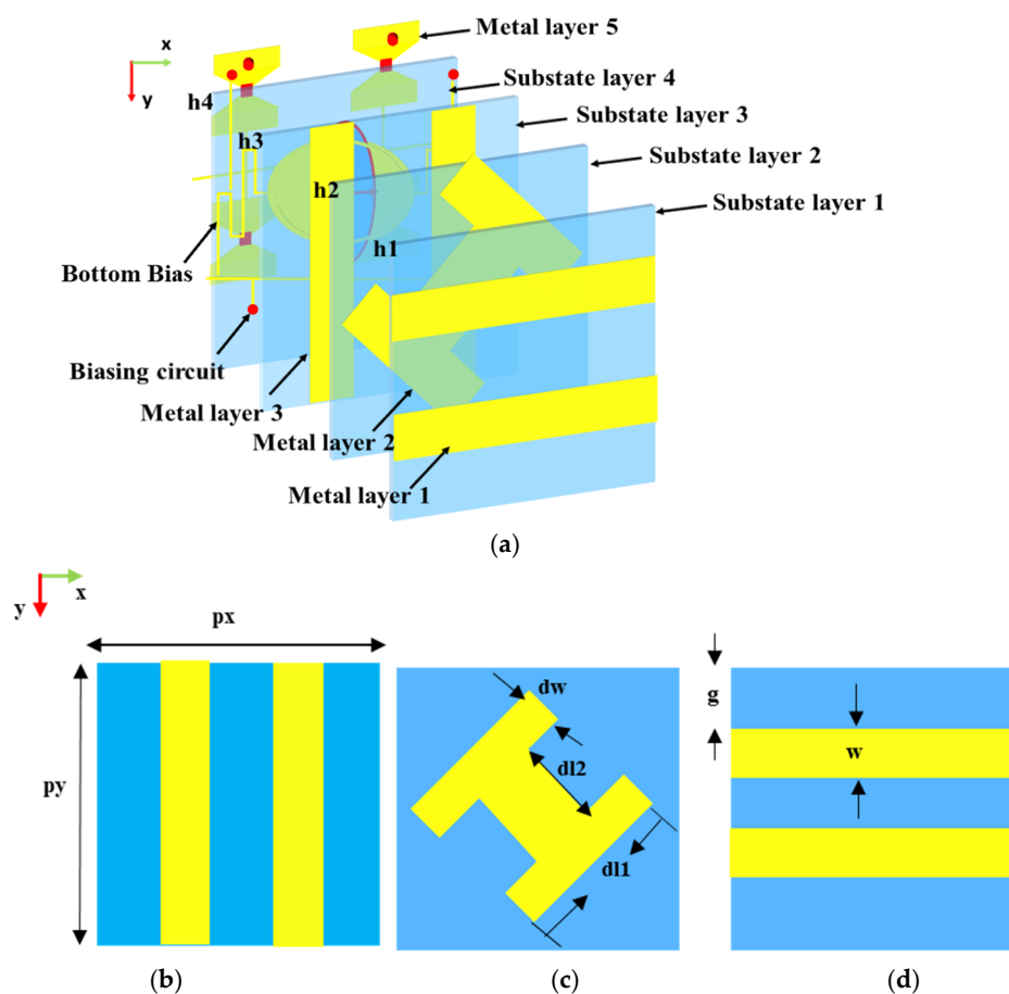
Figure 1. The schematic diagram of the suggested RMM working for full-space.
