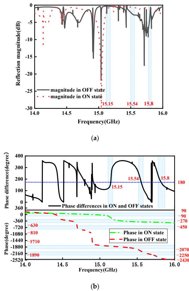
Figure 9. Simulated reflection coefficients of the presented MS in the ON and OFF states: (a) reflection coefficient; (b) reflection phase and reflection phase differences between p-i-n diode ON and OFF states.
