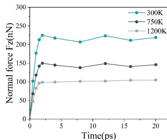
Figure 6. Evolution of the normal force in the spinning contact zone under different temperature conditions.
