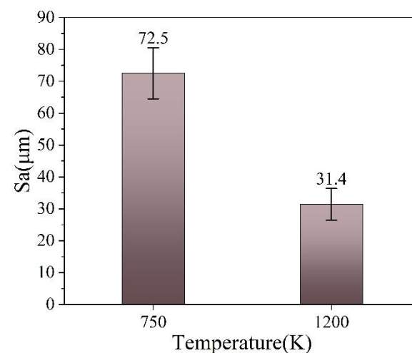
Figure 13. Variation in workpiece surface roughness S_a under different temperature conditions.
