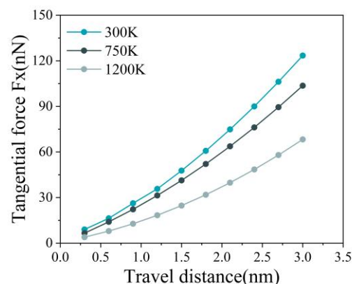
Figure 7. Evolution of the tangential force in the spinning contact zone under different temperature conditions.
