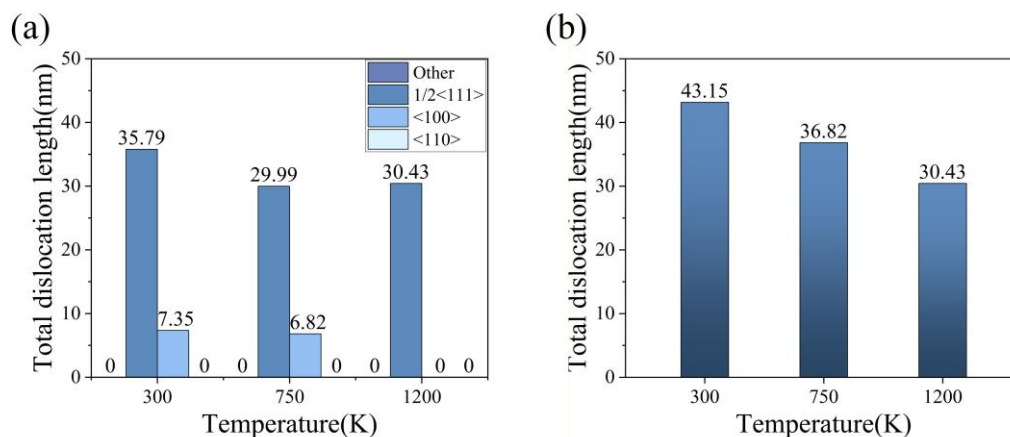
Figure 9. Evolution of dislocation line length under different temperature conditions: (a) dislocation type distribution and (b) total dislocation line length.
