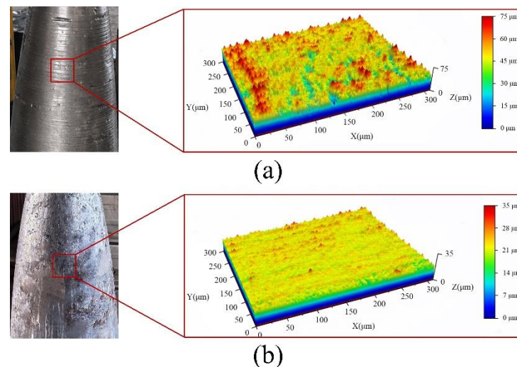
Figure 12. Three-dimensional surface morphologies of workpieces under different temperature conditions: (a) 750 K and (b) 1200 K.
