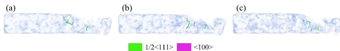
Figure 8. Dislocation evolution characteristics during spinning deformation under different temperature conditions: (a) 300 K, (b) 750 K, and (c) 1200 K.
