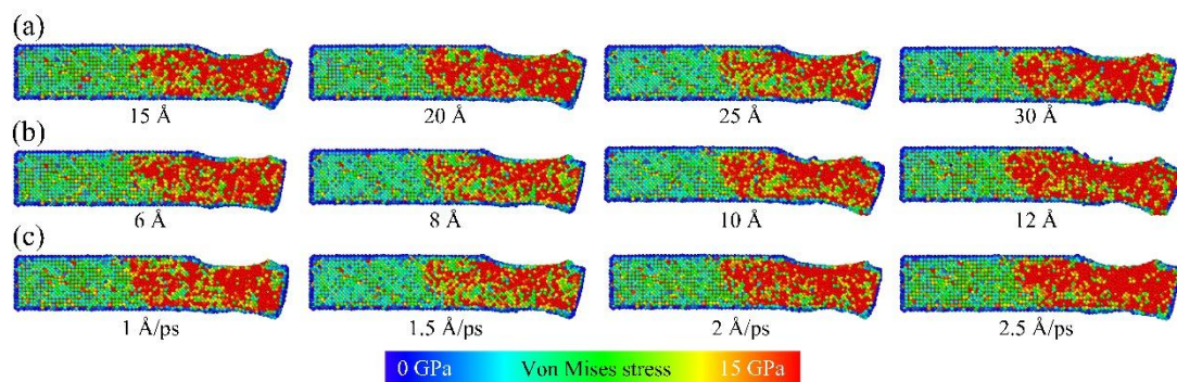
Figure 3. Effects of different process parameters on the Von Mises stress distribution in the local spinning contact zone: (a) different arc radii, (b) different indentation depths, and (c) different tangential sliding velocities.
