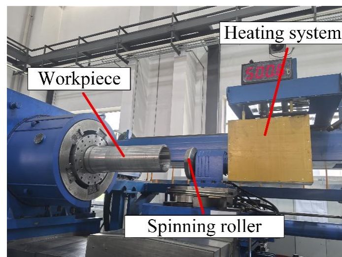
Figure 2. Experimental equipment.
