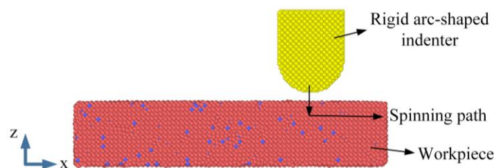
Figure 1. Schematic diagram of the indenter and workpiece model.
