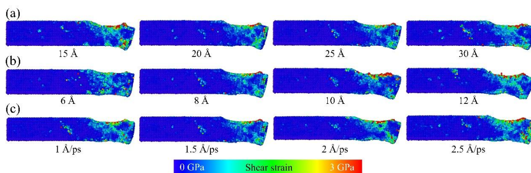
Figure 4. Effects of different process parameters on the shear-strain distribution in the local spinning contact zone: (a) different arc radii, (b) different indentation depths, and (c) different tangential sliding velocities.
