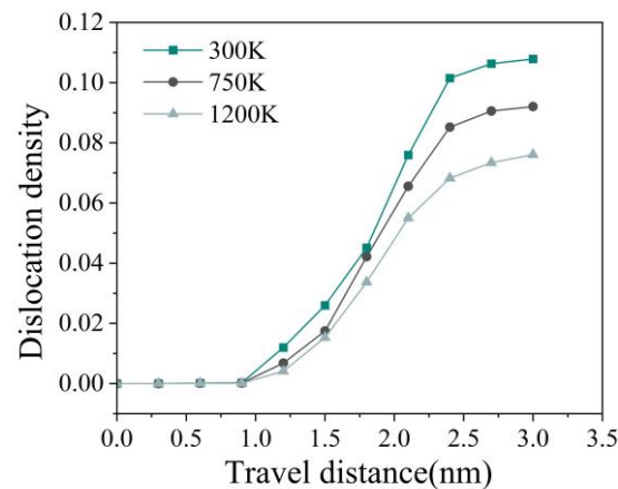
Figure 10. Evolution of dislocation density with sliding distance under different temperature conditions.
