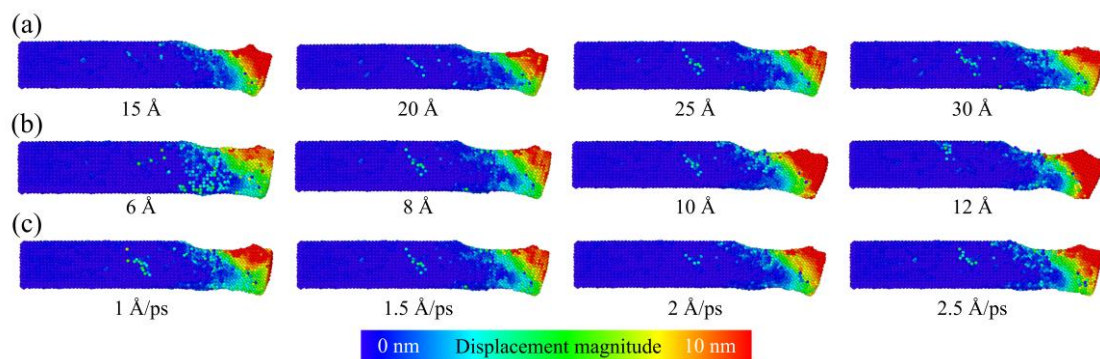
Figure 5. Atomic displacement distributions in the spinning contact zone under different process parameters: (a) different arc radii, (b) different indentation depths, and (c) different tangential sliding velocities.
