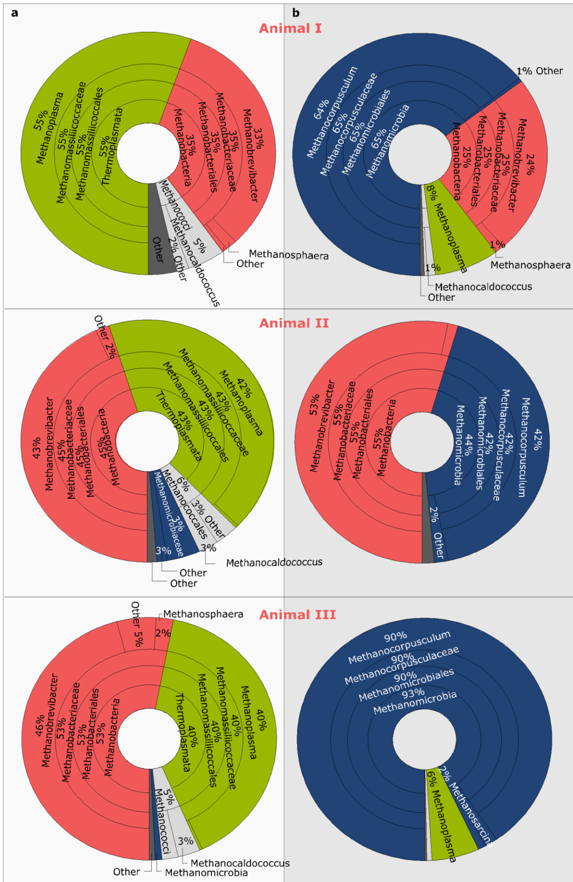
Figure S2. Krona charts illustrating the methanogenic community composition of (a) the rumen samples and (b) the manure samples from three individuals on phylum, class, order and family levels.
