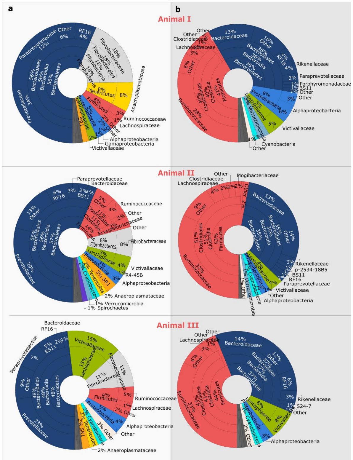
Figure S1. Krona charts illustrating the bacterial community composition of (a) the rumen samples and (b) the manure samples from three individuals on phylum, class, order and family levels.
