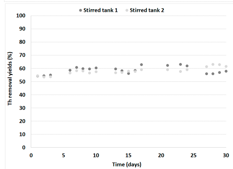
Supplementary Figure S1. Evolution of LREEs (a), HREEs (b), U (c) and Th(d) removal yields for RAT tailings
