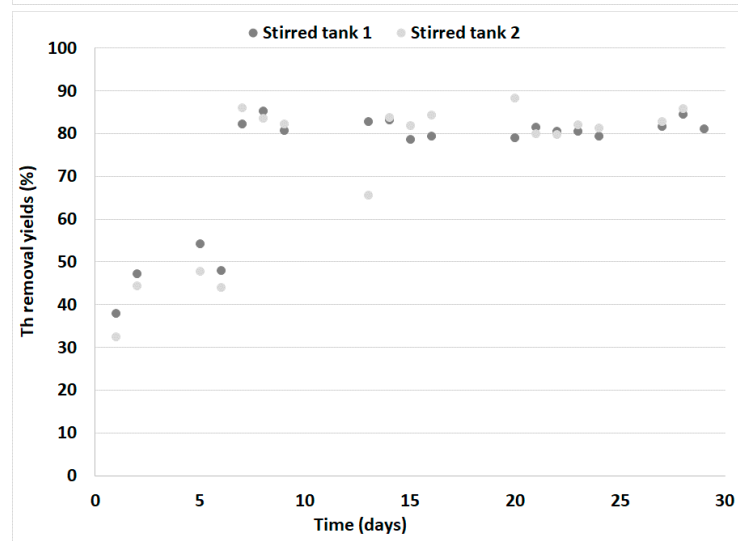
Supplementary Figure S2. Evolution of LREEs (a), HREEs (b), U (c) and Th(d) removal yields for DT tailings
