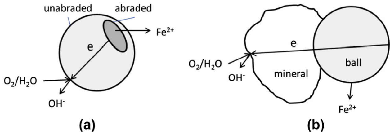
Figure 1. Showing corrosion wear for (a) differential abrasion cell (b) ball – mill galvanic cell. Adapted from [37].
