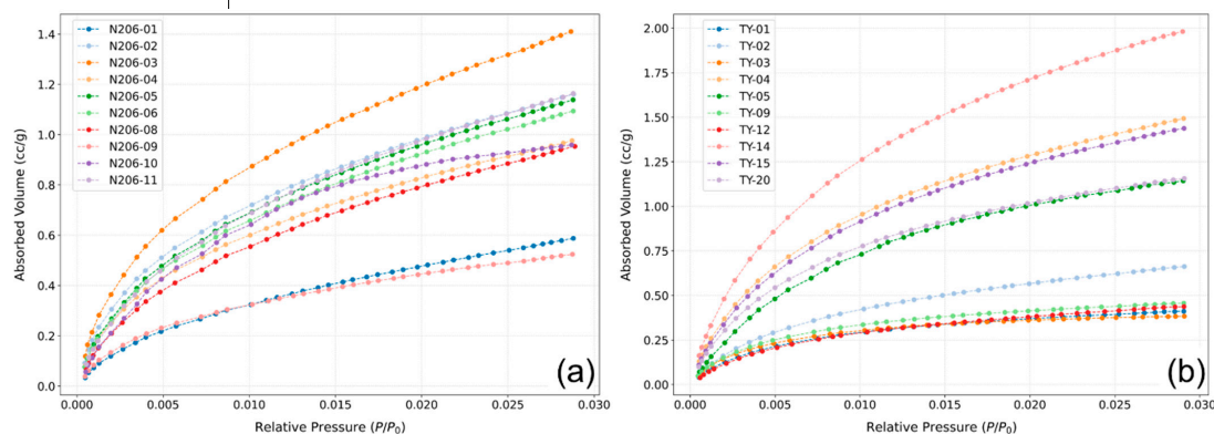
Figure 9. Low-pressure CO 2 adsorption curves of (a) Qiongzhusi (N206) and (b) Longmaxi (TY1) shales.
