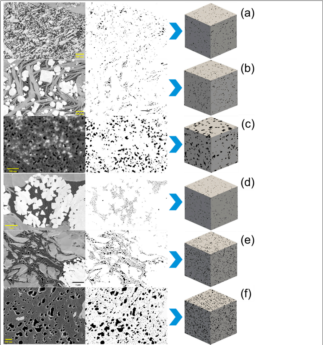
Figure 19. Shale pore reconstruction with the corresponding SEM images, for samples (a) N206-5 ( \varphi = 2.24\% ), (b) N206-2 ( \varphi = 2.48\% ), (c) N206-2 ( \varphi = 11.78\% ), (d) TY1-4 ( \varphi = 2.24\% ), (e) TY1-6 ( \varphi = 7.39\% ), (f) TY1-2 ( \varphi = 16.59\% ).
