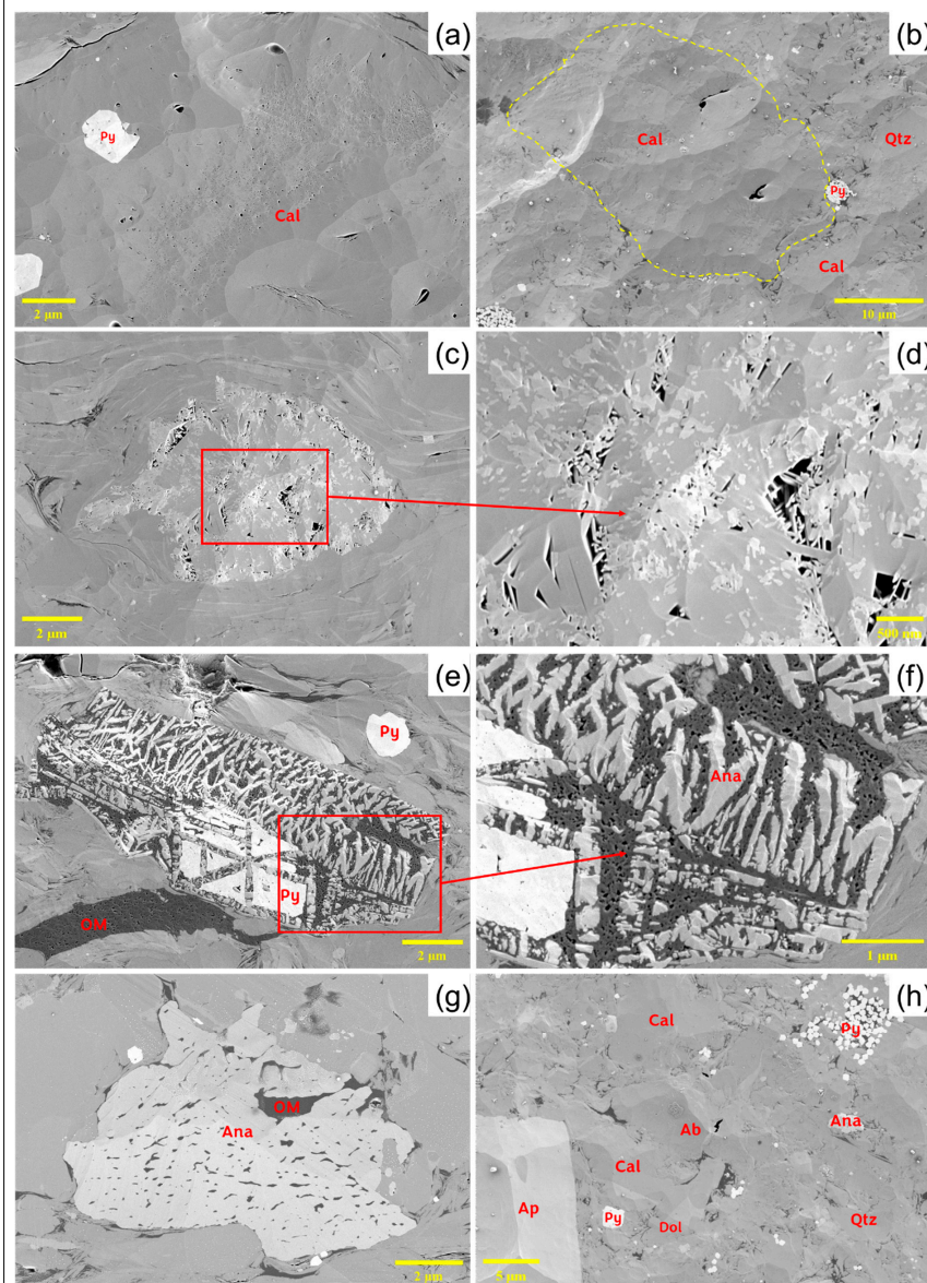
Figure 8. SEM images showing grains with associated porosity. (a) Calcite in Longmaxi shale (TY1) exhibiting sparse intragranular pores and embedded pyrites; (b) calcite in Qiongzhusi shale (N206), with localized intergranular pores; (c) porous anatase aggregate in TY1 sample; (d) magnified view of the region in (c), revealing submicron-scale intercrystalline pores. (e) Coexistence of anatase, pyrite, and organic matter in N206 shale; (f) close-up of (e) displaying anatase developed in OM nanopores; (g) compact anatase grain in N206 shale, embedded in non-porous OM, (h) mineralogical diversity in N206 shale. Ab: albite, Ana: Anatase, Ap: Apatite, Cal: Calcite, Dol: Dolomite, OM: Organic matter, Py: pyrite, Qtz: Quartz.
