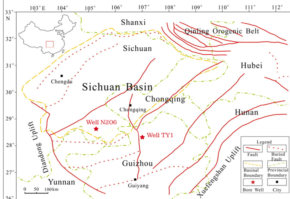
Figure 1. Sichuan basin geologic map showing well locations (modified from Sun et al. [99]).
