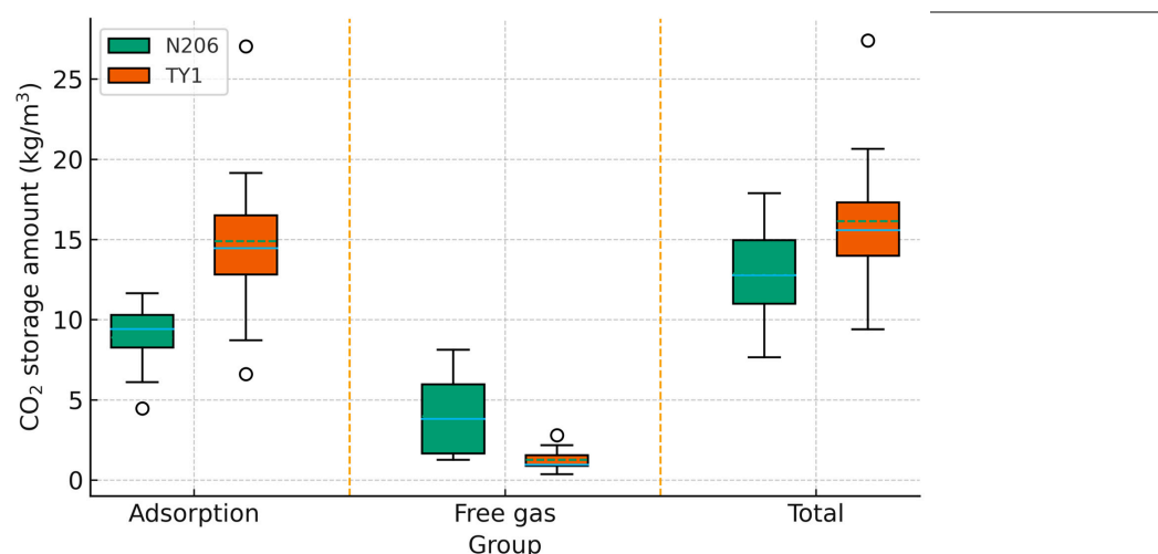
Figure 22. Comparison of adsorption, free-gas, and total CO 2 storage distributions for N206 and TY1.
