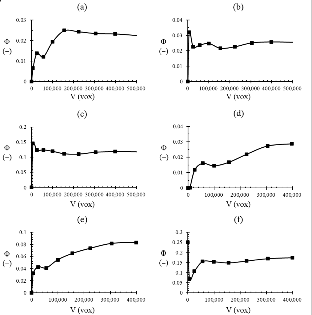
Figure A1. Plots to determine that the representative elementary volume (REV) has been reached for segmented SEM images (a–f) corresponding to Figure 19.
