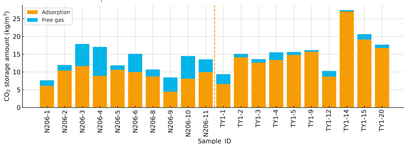
Figure 21. Comparison of CO_2 storage amount per sample for N206 and TY1: adsorption and free gas.
