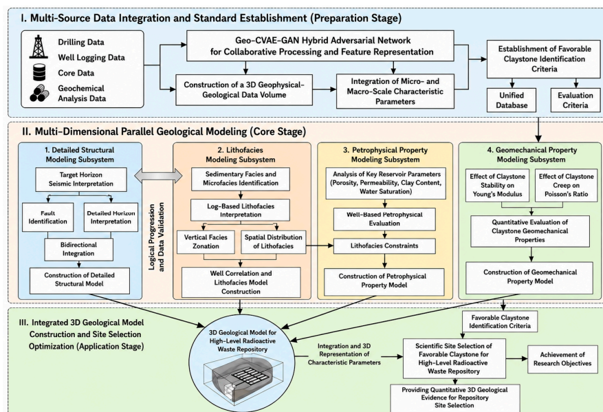
Figure 11. Schematic diagram of the research framework.
