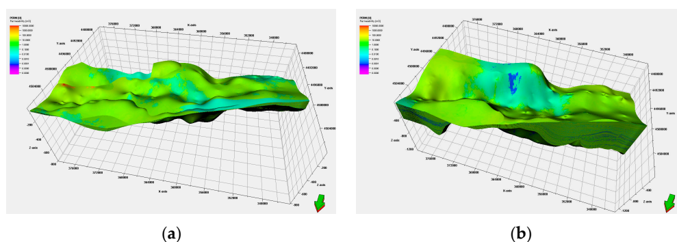
Figure 10. Permeability (PERM) attribute models of the (a) shallow and (b) deep layers (all axes in meters).
