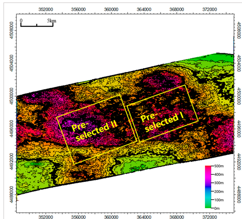
Figure 13. Thickness map of the deep layer of the study area.
