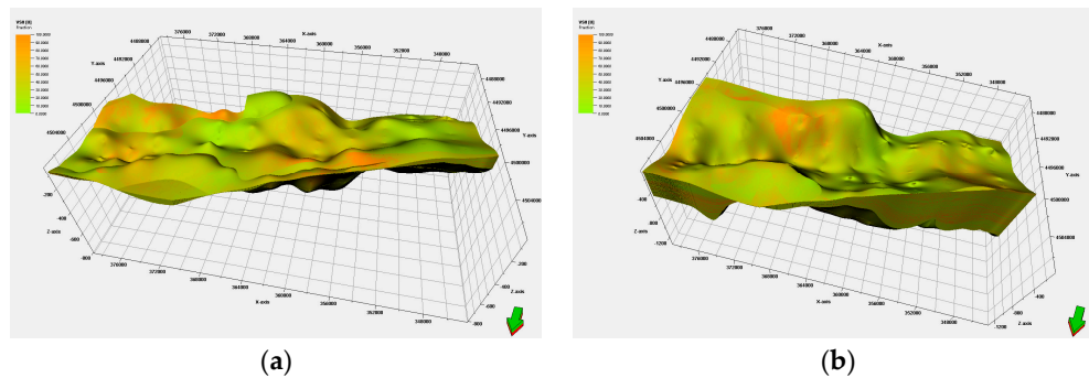
Figure 7. Vsh content attribute models for (a) shallow and (b) deep (all axes in meters).
