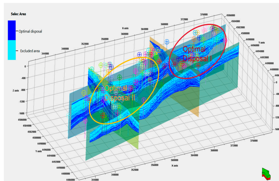
Figure 15. Geological modeling map of the preferred area for the repository in the Tamusu area (all axes in meters).
