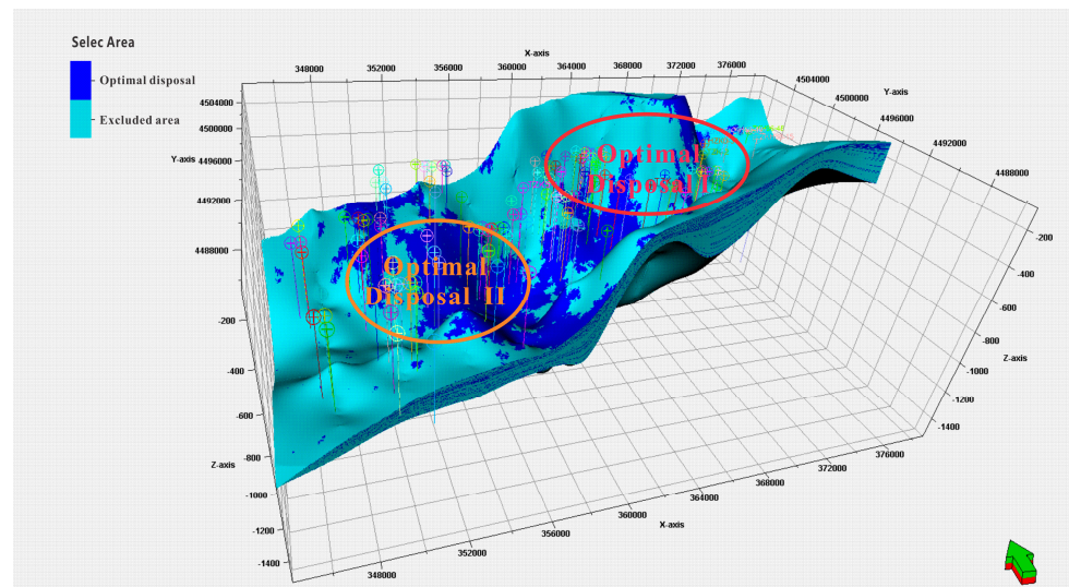
Figure 14. Geological modeling map of the preferred area for the repository in the Tamusu area (all axes in meters).
