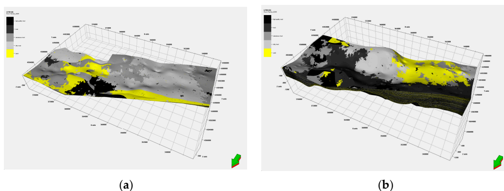
Figure 5. Three-dimensional lithofacies models of the (a) shallow and (b) deep layers (all axes in meters).
