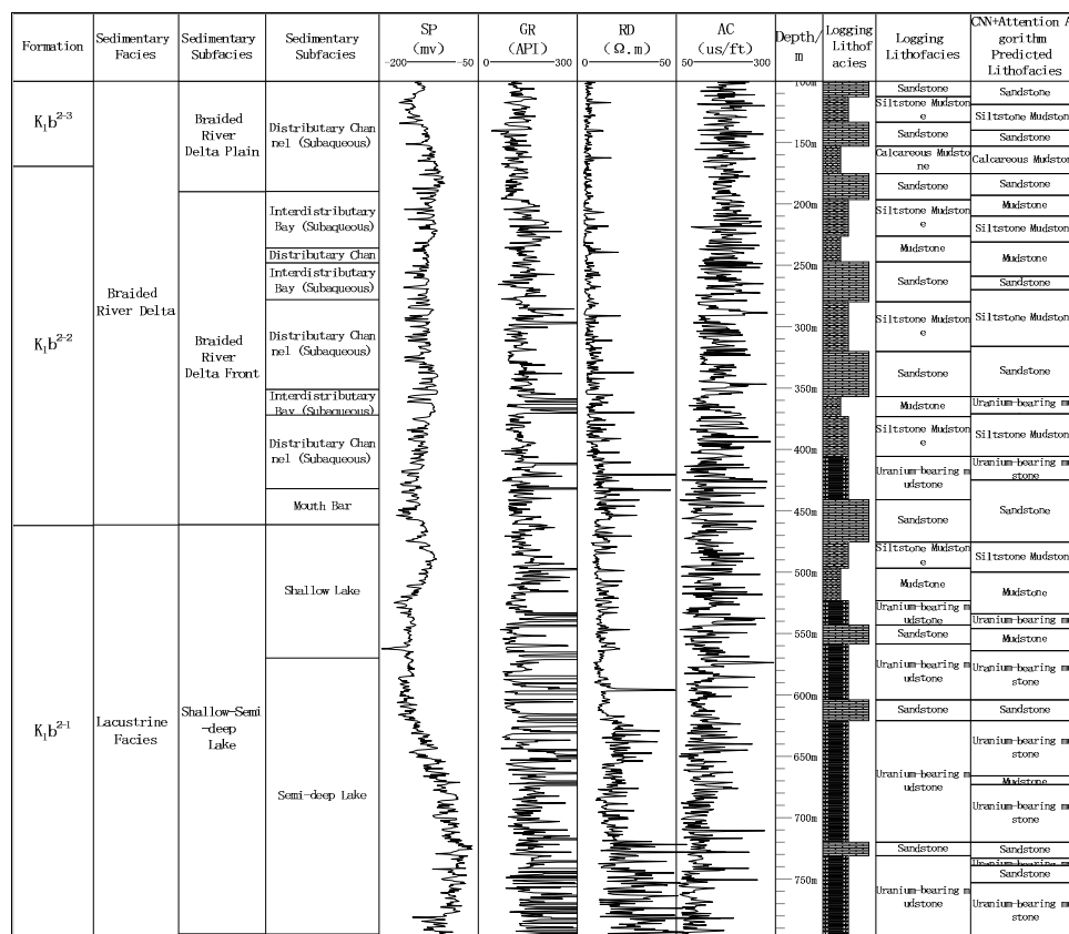
Figure 3. Comparison between lithofacies predicted by CNN + attention algorithm and logging lithofacies.
