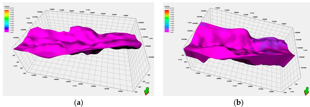
Figure 8. Porosity (POR) attribute models for (a) shallow and (b) deep (all axes in meters).
