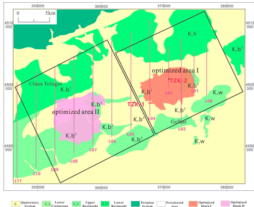
Figure 16. Map of preferred disposal zones in the Tamusu area.
