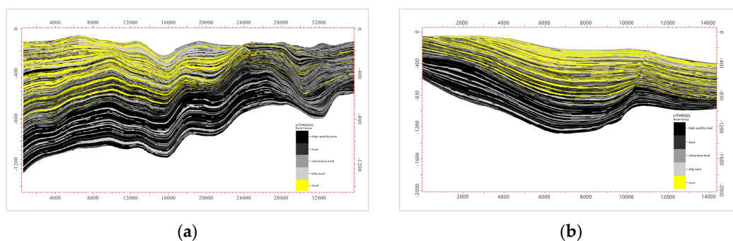
Figure 6. Deep lithofacies profiles for (a) E–W and (b) S–N (all axes in meters).
