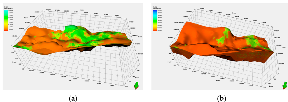
Figure 9. Water saturation ( S_w ) attribute models for (a) shallow and (b) deep (all axes in meters).
