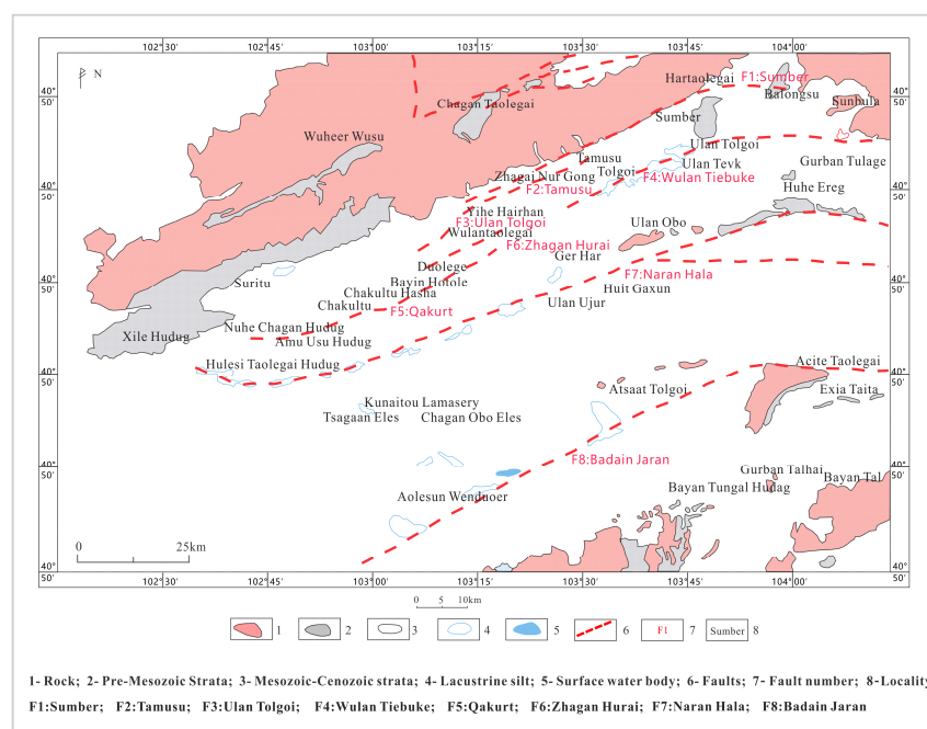
Figure 1. Structural system map of Tamusu area [22].
