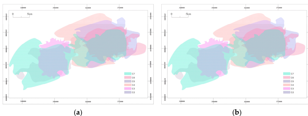
Figure 12. Stratified superposition maps of six property parameters in the (a) shallow and (b) deep layers.
