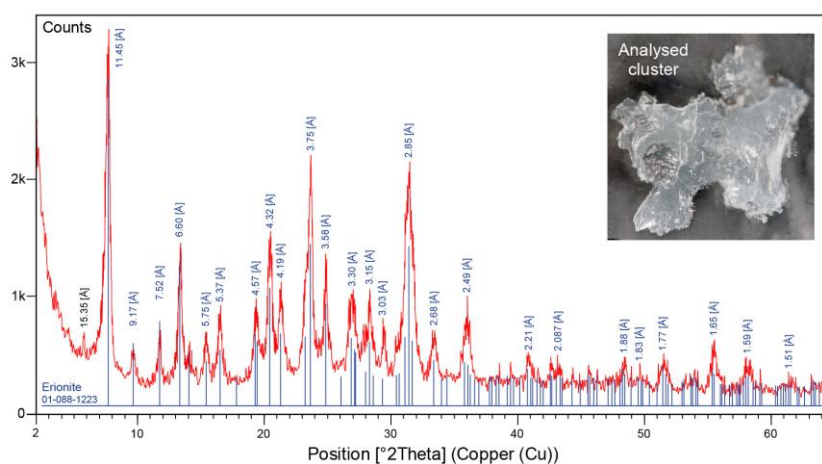
Figure 7. XRPD pattern of a soft cluster of an almost pure, fibrous erionite (see the inset). All reflections shown in blue are consistent with the erionite reference pattern, whereas the reflection shown in black is attributed to saponite impurities.
