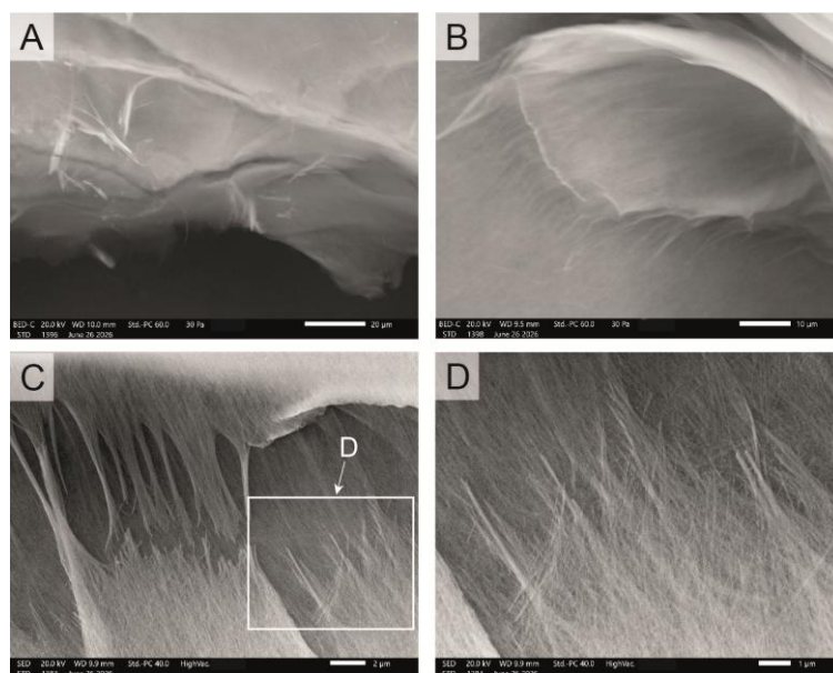
Figure 5. SEM images of Type 2 erionite. (A,B) General views of a delicate, soft film of erionite. (C) Detail of a curved area, showing extremely fine erionite fibers ( <0.1\ \mu\text{m} in diameter) that locally appear stretched and broken. (D) Higher-magnification view of a portion of the film, showing densely interwoven fibers that produce a fabric-like texture.
