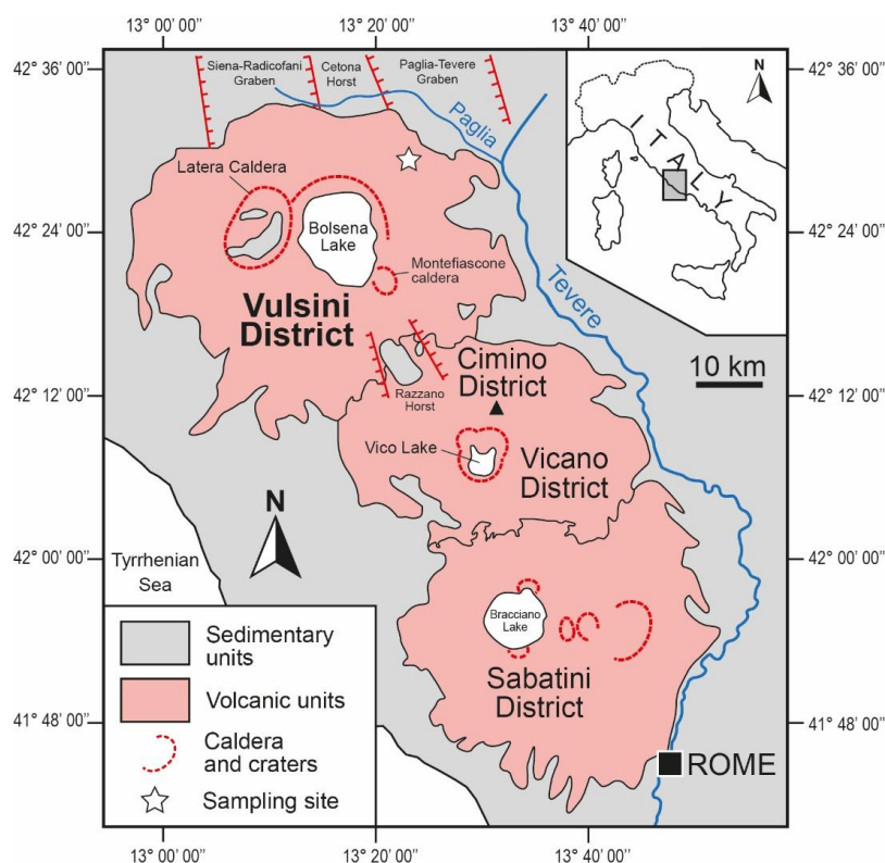
Figure 1. Geological sketch map of Central Italy showing the locations of the Vulsini, Cimino, Vicano, and Sabatini Volcanic Districts. The star indicates the sampling site (Porano quarry).
