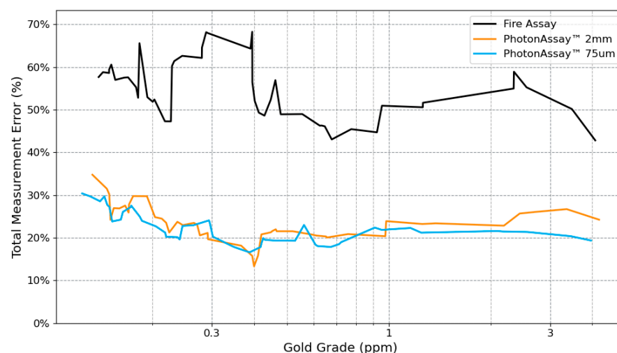
Figure 8. Example precision plot based on a HS comparing FA and PhotonAssay™ (crushed to 2 mm and pulverised to 75 \mu m) for coarse gold-bearing mineralisation.
