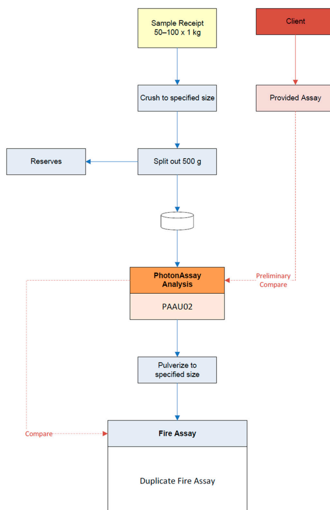
Figure 3. Flowsheet of the transitional feasibility study.
