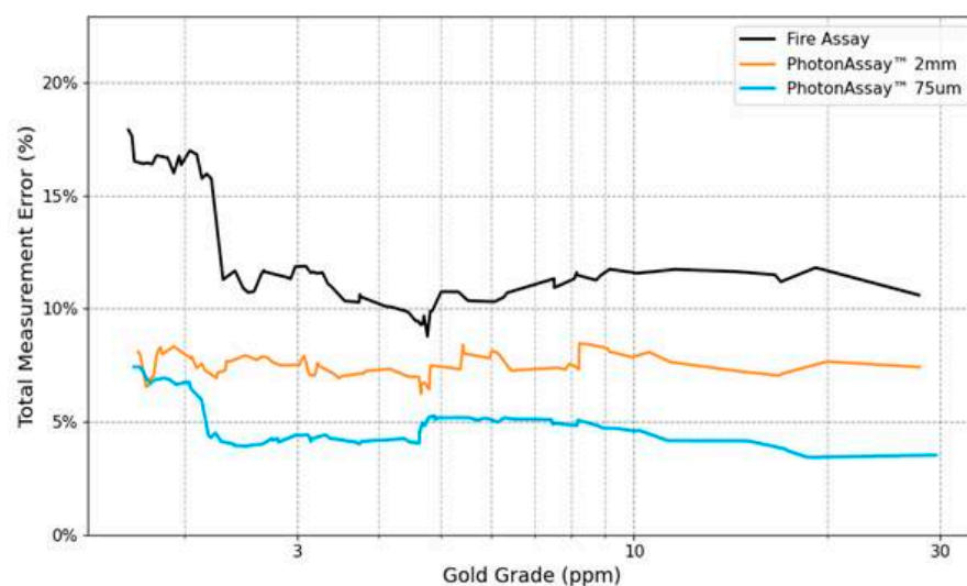
Figure 9. Example precision plot based on a HS comparing FA and PhotonAssay™ (crushed to 2 mm and pulverised to 75 \mu m) for fine gold-bearing mineralisation.
