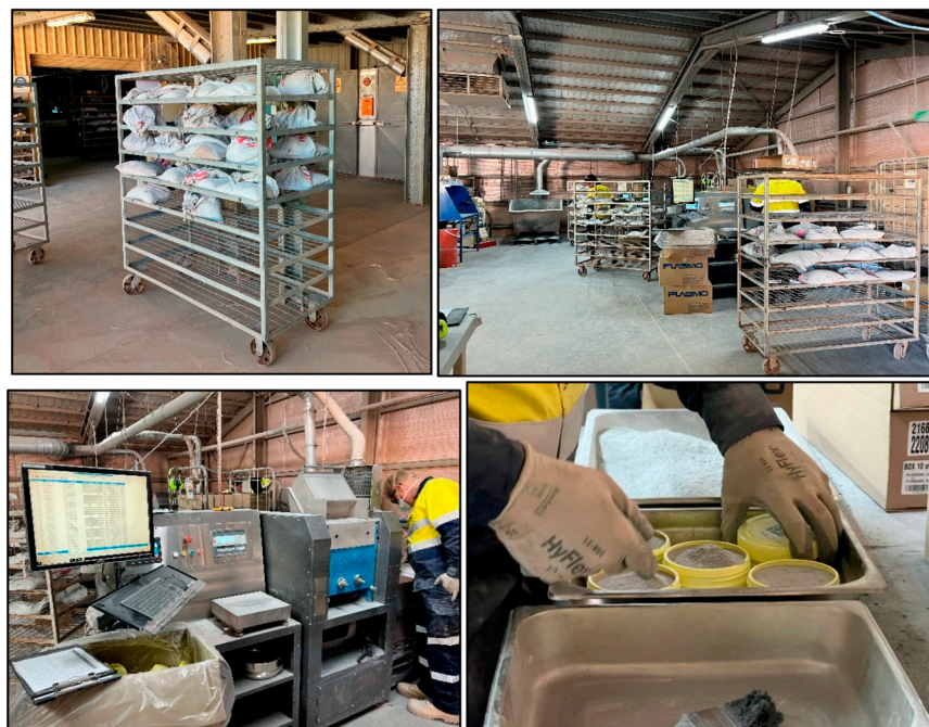
Figure 2. Novo Resources Corp. former Nullagine (WA) site preparation laboratory. ( Top left ) received samples ready to be placed into dryers. ( Top right ) general view of the sample preparation area. ( Bottom left ) Orbis smart crusher. ( Bottom right ) five filled PA jars which comprise one assay sub-sample.
