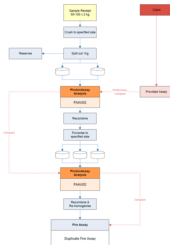
Figure 7. Flowsheet of the heterogeneity study.
