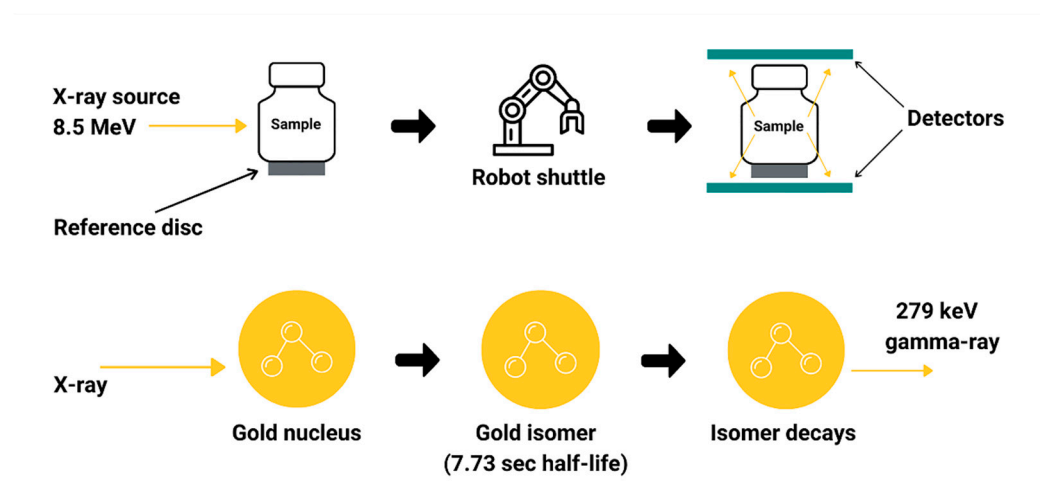
Figure 1. Illustration of the PhotonAssay™ process.
