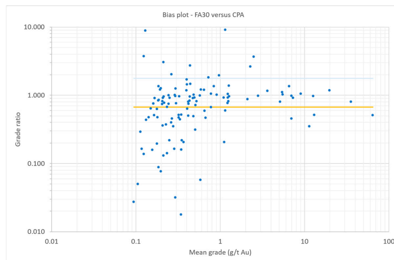
Figure 4. Tukey bias plot showing comparison between 120 FA and PhotonAssay™ (crushed) for coarse gold-bearing mineralisation. Horizontal lines: blue—mean plus 1x standard deviation; yellow—mean grade ratio.
