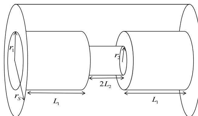
Figure 1. A single wide-and-narrow pore system. Each PC unit consists of n identical wide-and-narrow pore systems connected in series.
