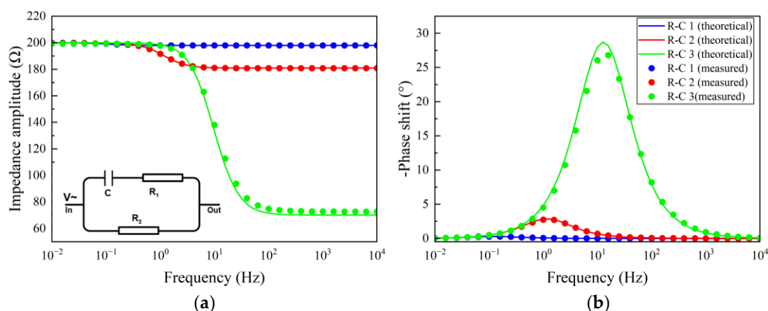
Figure 25. Validation of the impedance analyzer using three phase-bearing R–C reference networks. (a) Measured and theoretical impedance magnitudes. The inset in panel (a) shows the R–C reference
