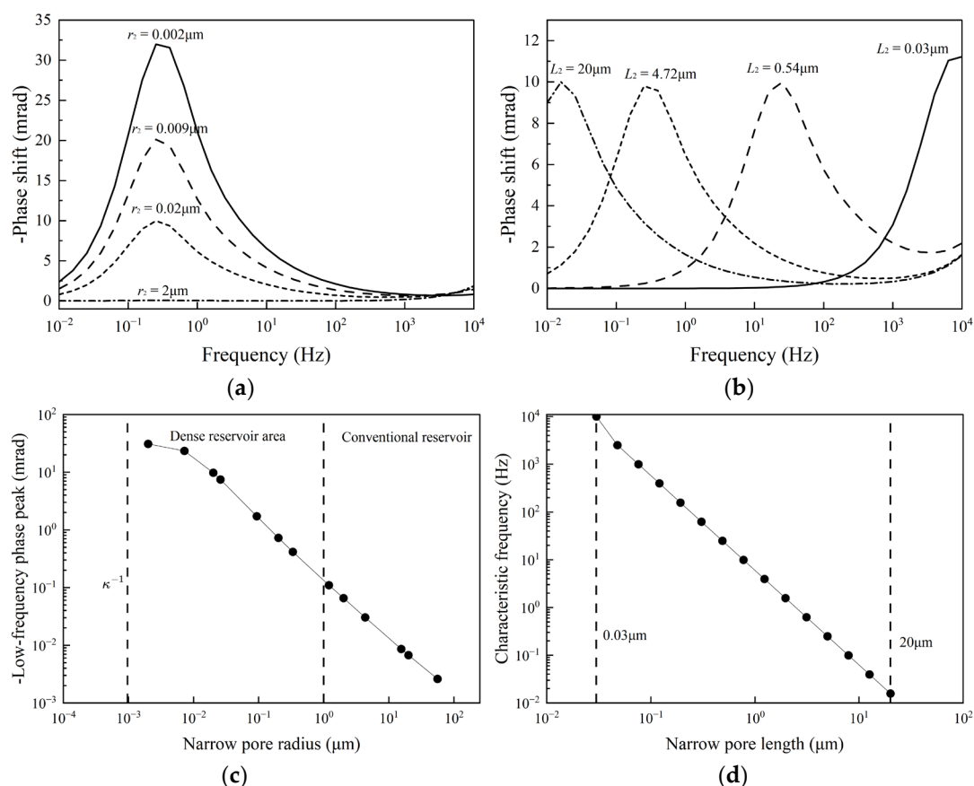
Figure 4. Panels (a,c) show how the single-pore low-frequency phase peak varies with narrow pore radius, and \kappa^{-1} is the Debye length; panels (b,d) show how the single-pore characteristic frequency varies with narrow pore length.
