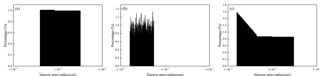
Figure 32. Pore throat distributions obtained from random impedance network model inversion for samples y, y1, and y2. (a) Pore throat distribution of sample y; (b) pore throat distribution of sample y1; (c) pore throat distribution of sample y2.
