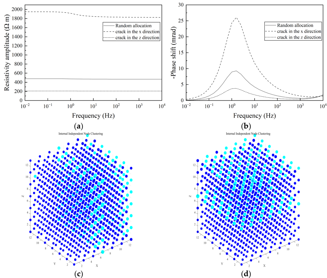
Figure 18. Simulated SIP responses (a,b) and clustering effects (c,d) for impedance networks with different spatial pore configurations, with a network size of 13 and 100 pore types. Dark-blue and cyan nodes represent the small-pore and large-pore/fracture-node classes, respectively. For the fracture network along the measurement direction, the average narrow pore radius r_2 range of independent nodes in the large-pore aggregation class is [0.07015,0.12751] μm; in the small-pore aggregation class, r_2 is [0.00738,0.0373] μm, and the microscopic heterogeneity parameter is \eta = 0.4959 ; for the fracture network perpendicular to the measurement direction, the average narrow pore radius r_2 range of independent nodes in the large-pore aggregation class is [0.0672,0.12786] μm; in the small-pore aggregation class, r_2 is [0.00786,0.03554] μm, and the microscopic heterogeneity parameter is \eta = 0.4952 ; and for the randomly allocated network, the heterogeneity parameter is \eta = 0.9892 .
