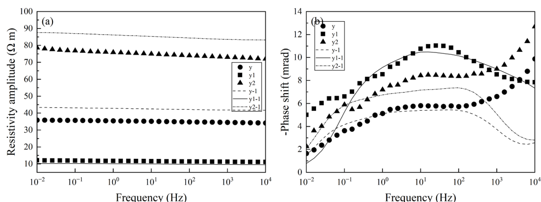
Figure 31. Panels (a,b) display complex resistivity spectra and impedance network simulation results for block and cylindrical samples in the same measurement direction. The dots represent the actual data, while the lines represent the simulated data. Only data within the sample-specific inversion ranges listed in Table 7 were included in the inversion; higher-frequency measurements are shown only to present the complete experimental spectra.
