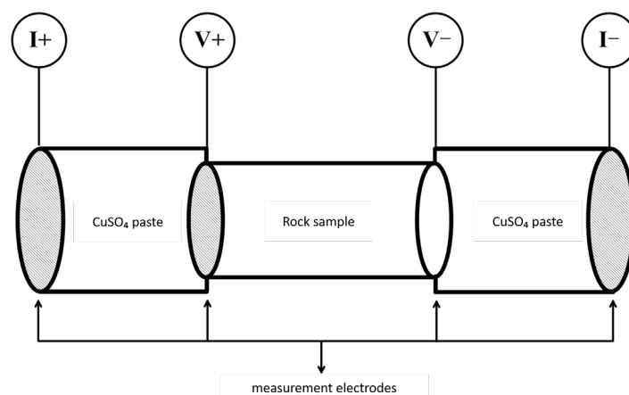
Figure 24. Schematic of the four-electrode configuration used for complex resistivity measurements. The outer electrodes (I+ and I-) were used for current injection, whereas the inner electrodes (V+ and V-) were used to measure the potential difference. CuSO 4 paste was used as the coupling medium between the electrodes and the rock sample.
