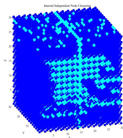
Figure 22. Addition of branch layers perpendicular to the fractures, based on the fractures along the measurement direction in Figure 18. Dark-blue and cyan nodes represent the small-pore and large-pore/fracture-node classes, respectively.
