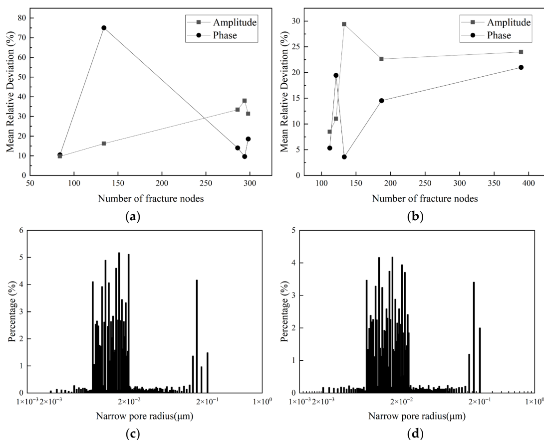
Figure 21. Relative changes in amplitude and phase for subnetworks of sizes 12 and 14 under different numbers of fracture nodes (a,b); (c,d) show the pore size distributions of the two networks with the smallest relative changes.
