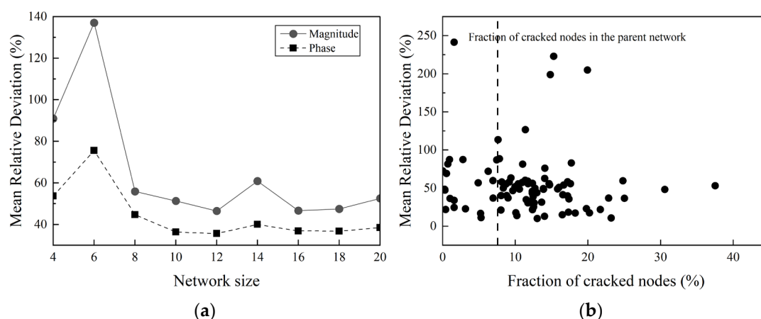
Figure 23. (a) Average relative deviations of SIP responses for subnetworks of different sizes over 10 extraction iterations; parent network parameters are the same as in Figure 19. (b) Average relative deviations in resistivity magnitude and phase for all subnetwork sizes extracted over 10 iterations, plotted against the corresponding fracture node proportions.
