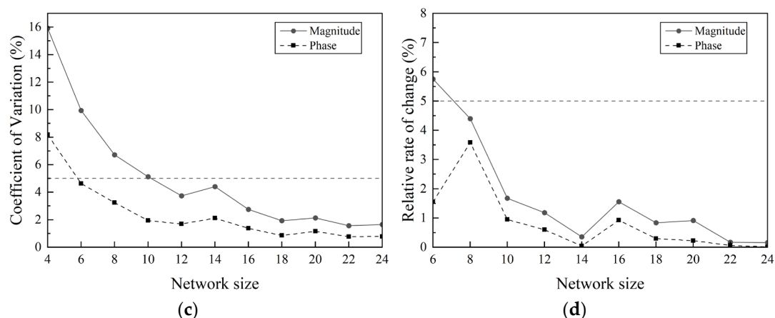
Figure 10. Coefficient of variation between cycles and relative change between sizes for amplitude and phase at different network sizes [(a,b) show results for v = 100 network, (c,d) show results for v = 1000 network]. Different network sizes use the same set of log-normally distributed pore types, with equal extraction probability for each pore type.
