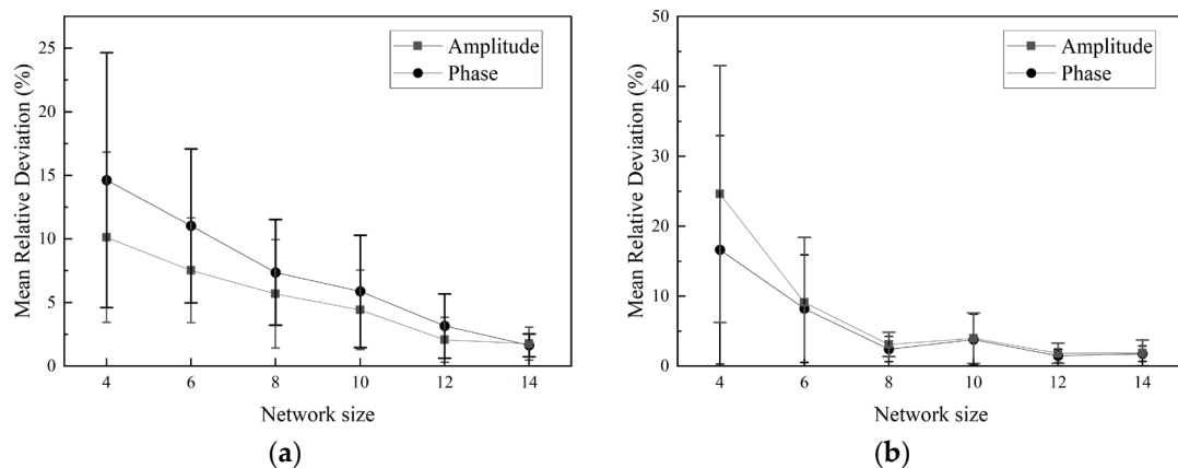
Figure 13. Subnetworks of different sizes extracted from two parent networks with \nu = 100 and \nu = 1000 . (a) Average relative deviation of SIP responses between the parent network ( \nu = 100 ) and its subnetworks; (b) average relative deviation of SIP responses between the parent network ( \nu = 1000 ) and its subnetworks.
