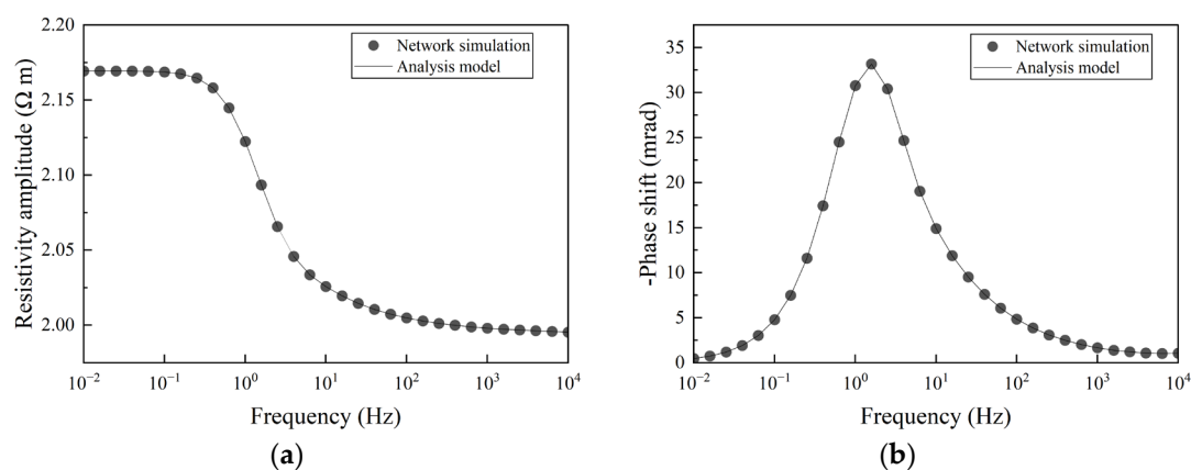
Figure 3. Simulated complex resistivity spectrum for a network of size 24. (a) Resistivity amplitude; (b) phase angle. Contains only one pore type ( r_2 = 0.2 \mu\text{m} , L_2 = 2 \mu\text{m} ). Points are network simulation results, and the curve is the analytical solution of the membrane polarization model for a single pore type.
