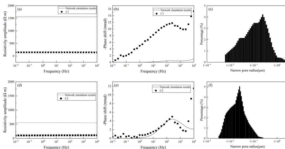
Figure 27. We interpolated the MICP distributions from samples C1 and C2 to construct 50 pore types and simulated them with the impedance network model. Panels (a–c) show the results for sample C1—resistivity amplitude, phase, and pore throat distribution—in that order. Panels (d–f) present the corresponding outputs for sample C2. Solid curves denote the network simulations; scatter points mark the experimental data.
