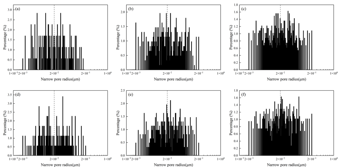
Figure 14. Pore throat distributions of subnetworks with network sizes 4, 6, and 8 in the parent network with \nu = 100 in Figure 13. Panel (a) shows the pore throat distribution of the subnetwork
