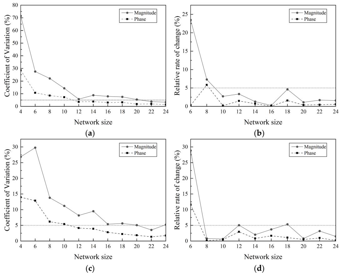
Figure 12. Inter-cycle coefficient of variation and inter-size relative rate of change for magnitude and phase across different network sizes with expanded pore radius and length distribution intervals relative to Figure 10 [(a,b): V = 100 network; (c,d): V = 1000 network].
