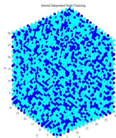
Figure 16. Optimization effect of the \eta = 0.605 network in Figure 15. Different colors represent different classes. The optimization algorithm divides the network into two classes: large-pore clusters and small-pore clusters.
