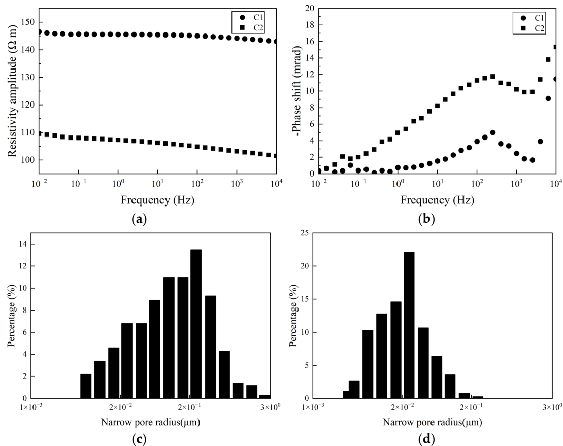
Figure 26. Panels (a,b) show the complex resistivity spectrum data of two measured samples, (c) shows the pore throat distribution of sample C1, and (d) shows the pore throat distribution of sample C2.
