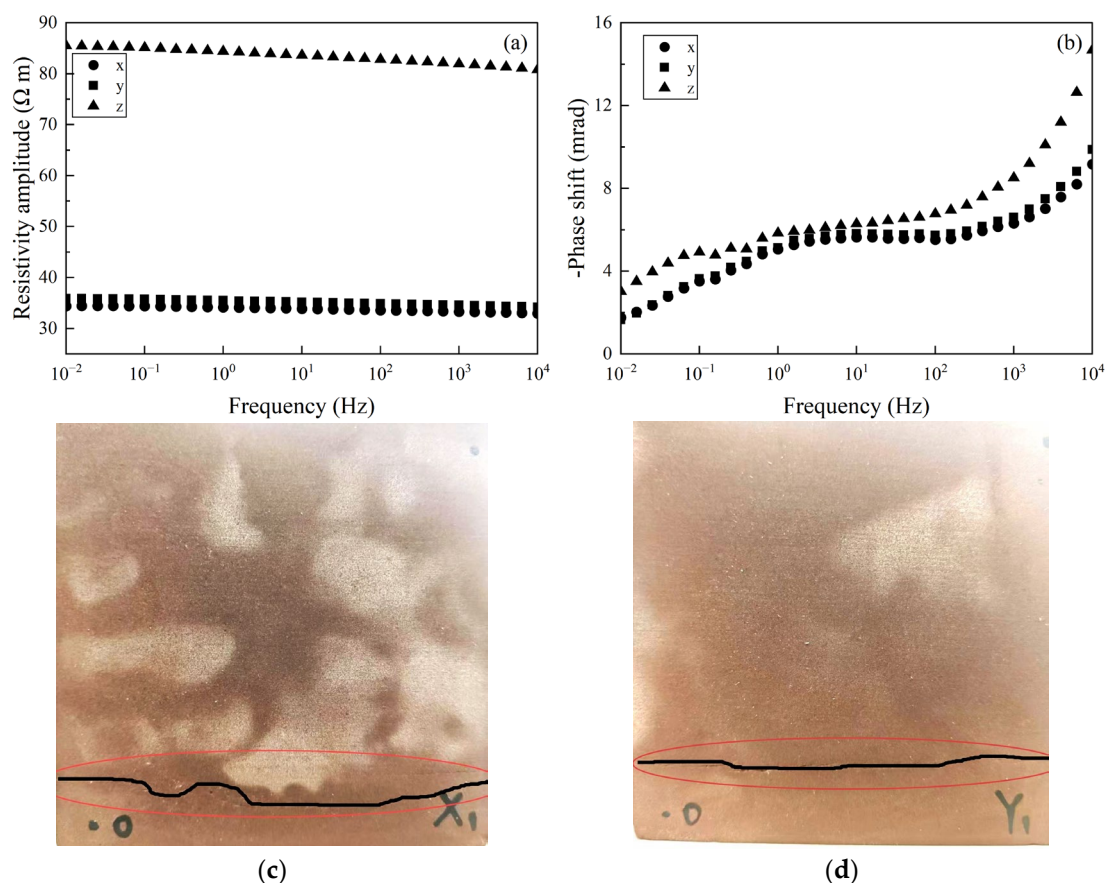
Figure 29. Panels (a,b) show resistivity amplitude and phase spectrum data for block sample S03-3k, with x, y, and z indicating results from different measurement directions; (c) denotes the measurement direction along the x-axis; and (d) denotes the measurement direction along the y-axis. The red outlines in panels (c,d) indicate the visible fracture traces.
