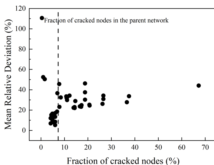
Figure 20. Average relative deviations in resistivity magnitude and phase for all subnetwork sizes across 10 extraction iterations, plotted against the corresponding fracture node proportions. Data points for subnetworks containing no fracture nodes were excluded from the comparison because their relative deviations exceeded tenfold, which would obscure the distribution of the remaining data.
