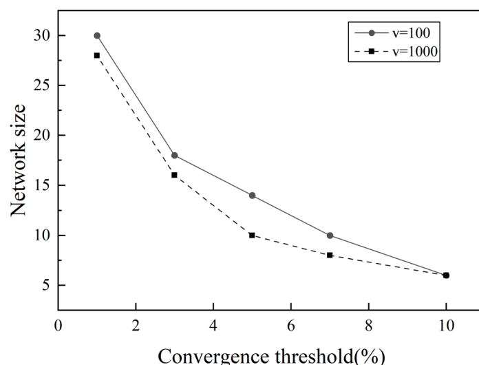
Figure 11. REV size of the random impedance network model under different thresholds.
