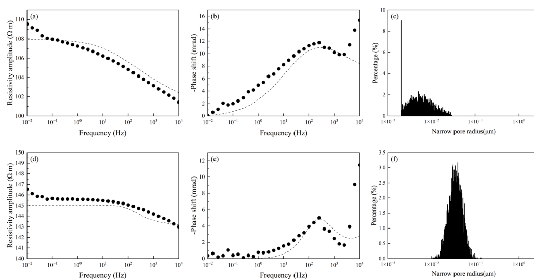
Figure 28. Using Bayesian optimization, we constructed pore types and simulated them with the impedance network model. Panels (a–c) show the results for sample C1 (81 pore types): resistivity amplitude, phase, and pore throat distribution, respectively. Panels (d–f) give the corresponding
