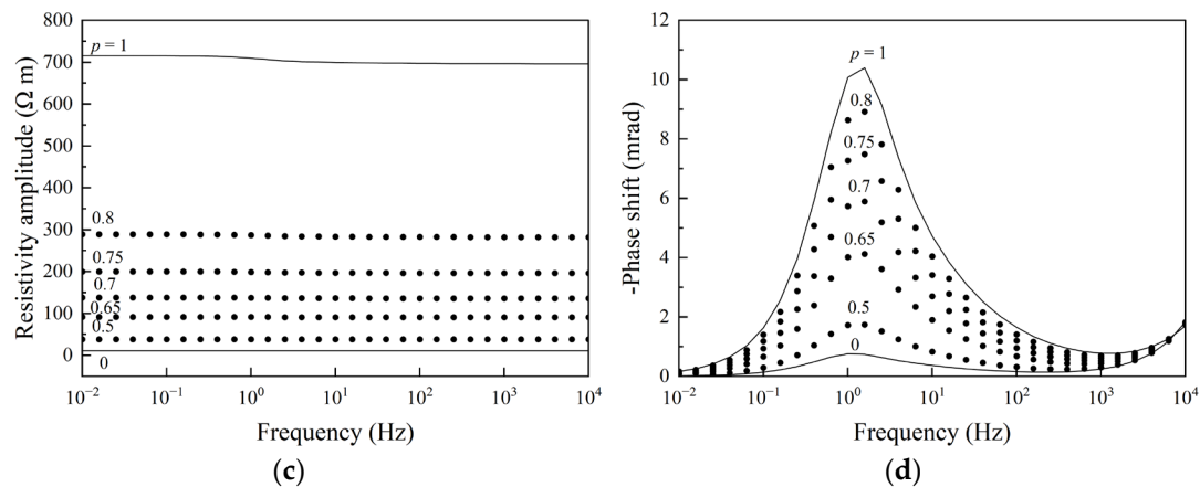
Figure 6. Complex resistivity spectra of a network with size 24 under different pore type proportions, with fixed pore length. The network contains two pore types [(a,b) correspond to r_2 = 0.002 \mu\text{m} , L_2 = 2 \mu\text{m} and r_2 = 0.02 \mu\text{m} , L_2 = 2 \mu\text{m} ; (c,d) correspond to r_2 = 0.02 \mu\text{m} , L_2 = 2 \mu\text{m} and r_2 = 0.2 \mu\text{m} , L_2 = 2 \mu\text{m} ]. p denotes the proportion of the narrower-throat pore type relative to the total pore volume of the network.
