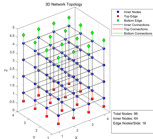
Figure 2. Schematic of the impedance network model with a network size of 4.
