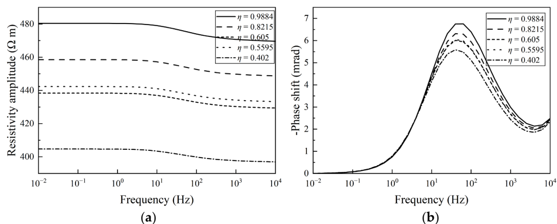
Figure 15. Simulated SIP responses of an impedance network with a network size of 31 and 100 pore types under different heterogeneity parameters: (a) resistivity magnitude and (b) phase. The network parameters used are the same as in Table 3.
