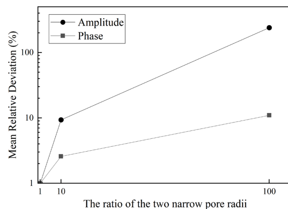
Figure 7. Relative changes in the average value of the membrane polarization analytical model and the network simulation amplitude and phase at p = 0.5 under different pore throat ratios for two pore types.
