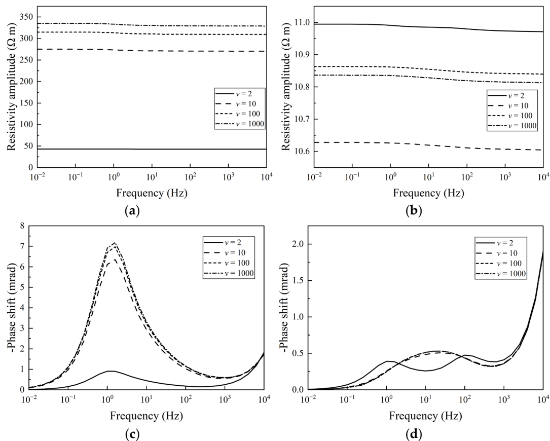
Figure 8. Complex resistivity spectra for different numbers of pore types in a network of size 24. Numbers of pore types \nu = 2, 10, 100 , and 1000 are generated using a logarithmic equal-interval distribution, with each pore type having the same proportion in the network. Panels (a,c) are for fixed pore length: r_{2,\min} = 0.002 \mu\text{m} , r_{2,\max} = 0.2 \mu\text{m} , L_2 = 2 \mu\text{m} . Panels (b,d) are for fixed pore cross-sectional area: L_{2,\min} = 0.08 \mu\text{m} , L_{2,\max} = 2 \mu\text{m} , r_2 = 0.2 \mu\text{m} .
