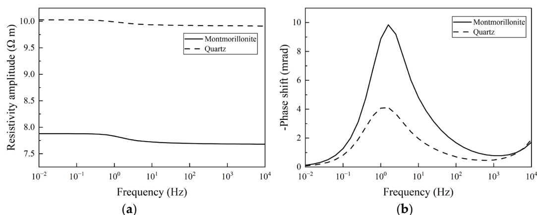
Figure 5. (a) Variations in the resistivity magnitude of a single pore under different electrochemical parameters. (b) Variations in the phase of a single pore under different electrochemical parameters.
