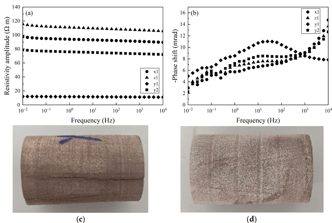
Figure 30. Panels (a,b) show the resistivity amplitude and phase spectrum data of different plug samples. The differences among samples x1-x2 and z1-z3 are less than 5%, so only one curve is plotted for each group. Panel (c) represents sample y1, and (d) represents sample y2.
