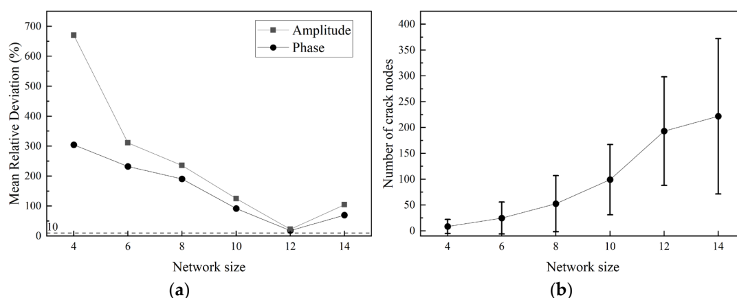
Figure 19. Panel (a) is mean relative deviation of subnetworks of different sizes, with parent network parameters same as in Figure 8, and (b) is number of crack nodes contained in different subnetwork sizes.
