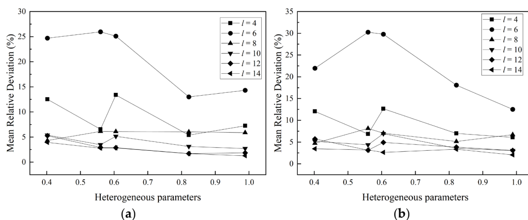
Figure 17. Mean relative deviation of subnetworks of different sizes from the parent network in Figure 15. Panel (a) shows the resistivity amplitude; (b) shows the phase peak. Each subnetwork was extracted 10 times.
