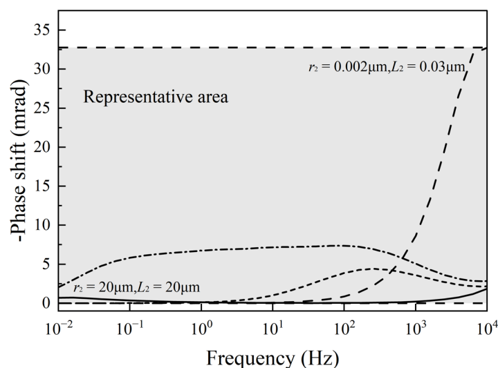
Figure 9. The gray region in the figure represents the representable range of the random impedance network model; this range is bounded by two sets of geometric parameters at the opposite ends of the diagonal.
