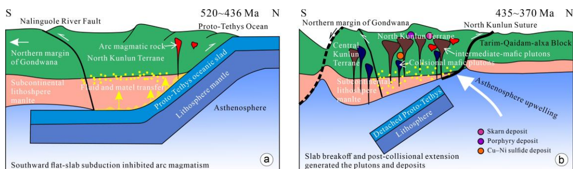
Figure 11. Schematic cartoon showing the tectonic evolution and mineralization of the Qimantage metallogenic belt in the East Kunlun Orogenic Belt (Modified from [106]).
