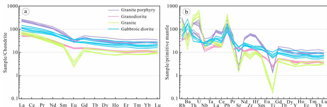
Figure 6. Chondrite-normalized REE pattern (a) and primitive mantle-normalized trace element spider diagram (b) of intrusive rocks in the Niukutoudong deposit. The values of primitive mantle and chondrite are from [71].
