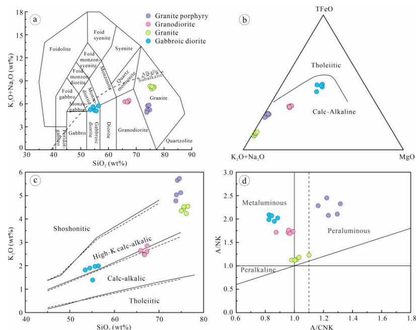
Figure 5. Geochemical diagrams of intrusive rocks from the Niukutoudong deposit. (a) \text{SiO}_2 vs. \text{K}_2\text{O} + \text{Na}_2\text{O} [67]; (b) \text{TFeO}-\text{K}_2\text{O} + \text{Na}_2\text{O}-\text{MgO} [68]; (c) \text{SiO}_2 vs. \text{K}_2\text{O} [69]; (d) \text{A/CNK} vs. \text{A/NK} [70].
