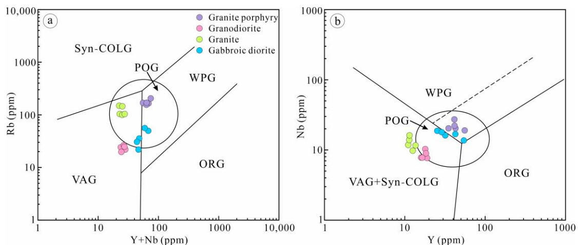
Figure 9. Diagrams for discriminating the tectonic setting of granites. (a) Y + Nb vs. Rb [94]; (b) Y vs. Nb [95]. Syn-COLG: syn-collisional granites; POG: post-collisional granites; WPG: within-plate granites; VAG: volcanic arc granites; ORG: ocean ridge granites.
