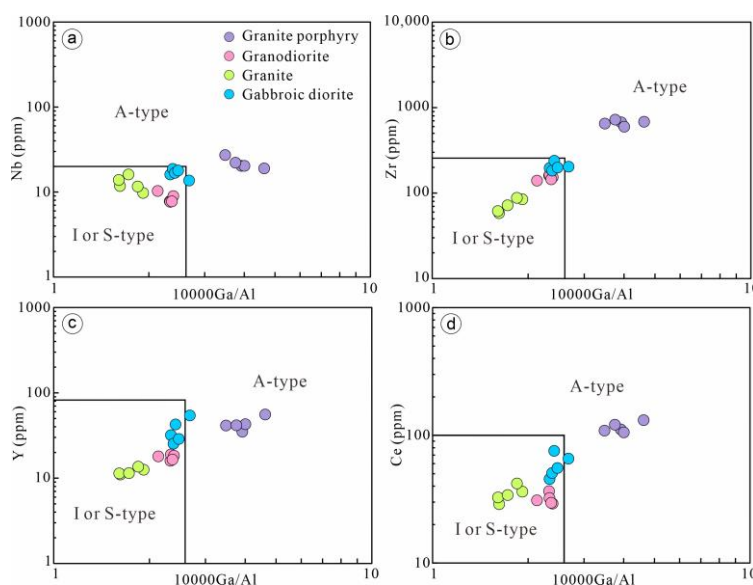
Figure 7. The discrimination diagrams of intrusive rocks from the Niukutoudong deposit. (a–d) Nb, Zr, Y and Ce vs. 10,000 \times Ga/Al , respectively [78].
