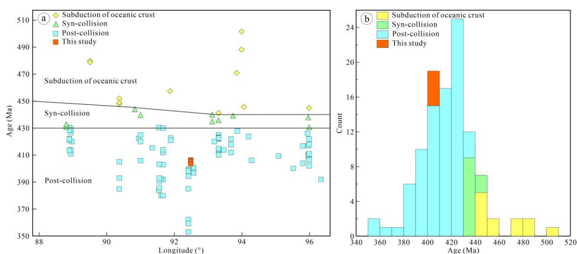
Figure 10. Schematic diagram of the Early Paleozoic tectono-magmatic event sequence in the western segment of the East Kunlun Orogenic Belt. Age data are from [1,11–53] and references therein. (a) Plot of age vs. longitude and (b) histogram of age distribution for magmatic rocks of different tectonic stages.
