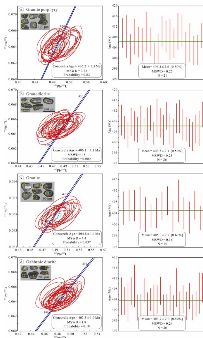
Figure 4. Representative CL images, zircon U-Pb concordia diagrams and weighted average ages diagrams. (a) The results of the granite porphyry sample; (b) the results of the granodiorite sample; (c) the results of the granite sample; (d) the results of the gabbroic diorite sample.
