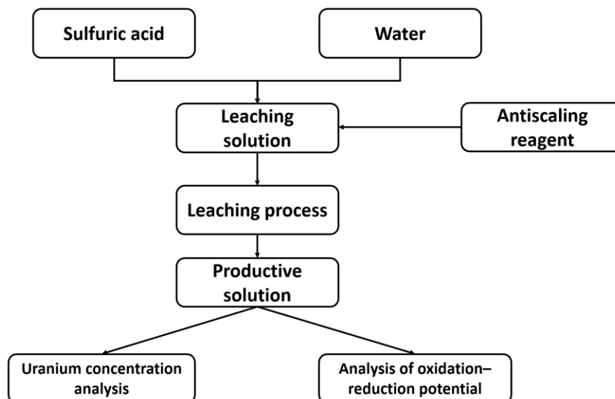
Figure 4. Flowchart of the laboratory experimental procedure.
