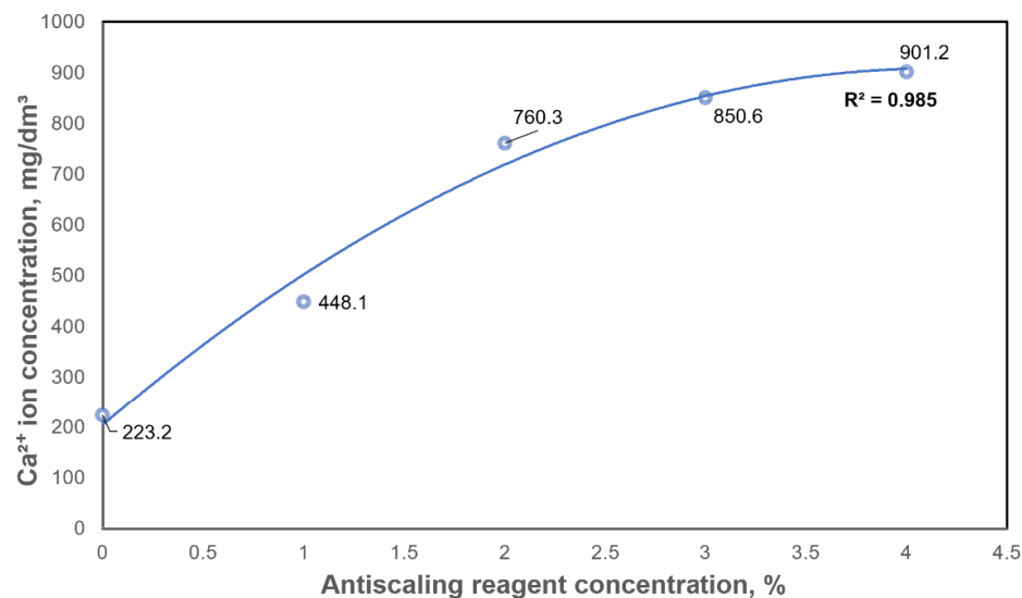
Figure 5. Changes in the degree of Ca 2+ ion dissolution in the solutions.
