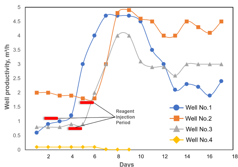
Figure 8. Changes in injection well performance before and after reagent injection.
