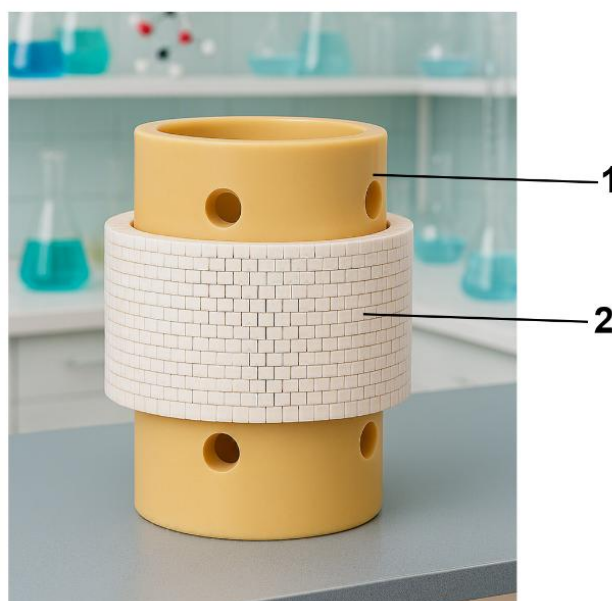
Figure 1. Structure of the frame-disc filter (1—inner perforated pipe; 2—filter discs).
