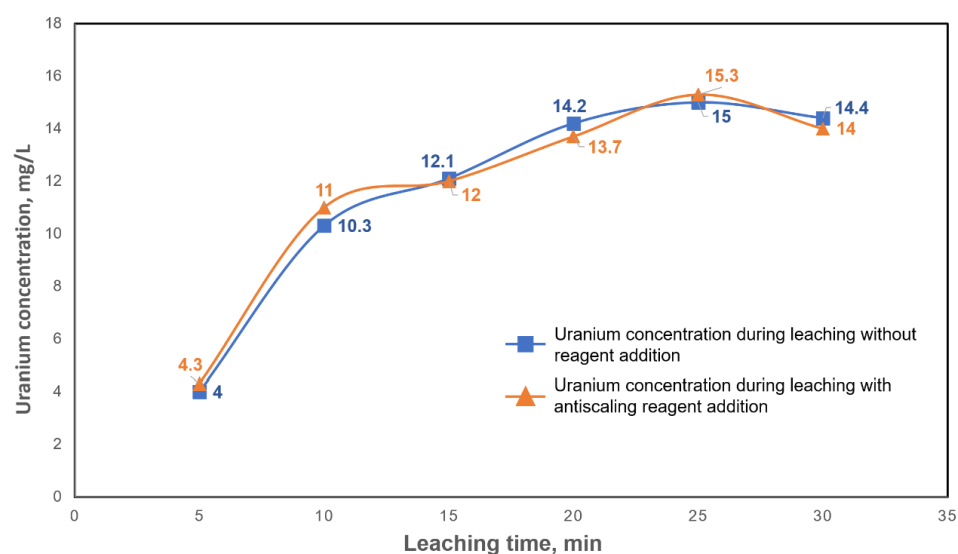
Figure 6. Dependences of uranium concentration in the pregnant leach solution on leaching time.
