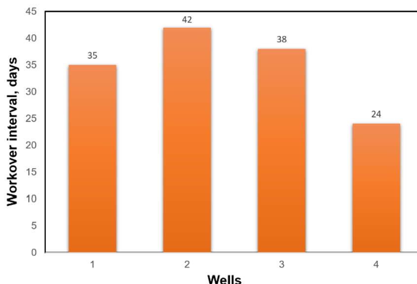
Figure 9. Workover intervals of the wells. Wells No. 1, 2, and 3 were treated using the proposed reagent, whereas well No. 4 was operated without the addition of the proposed reagent.
