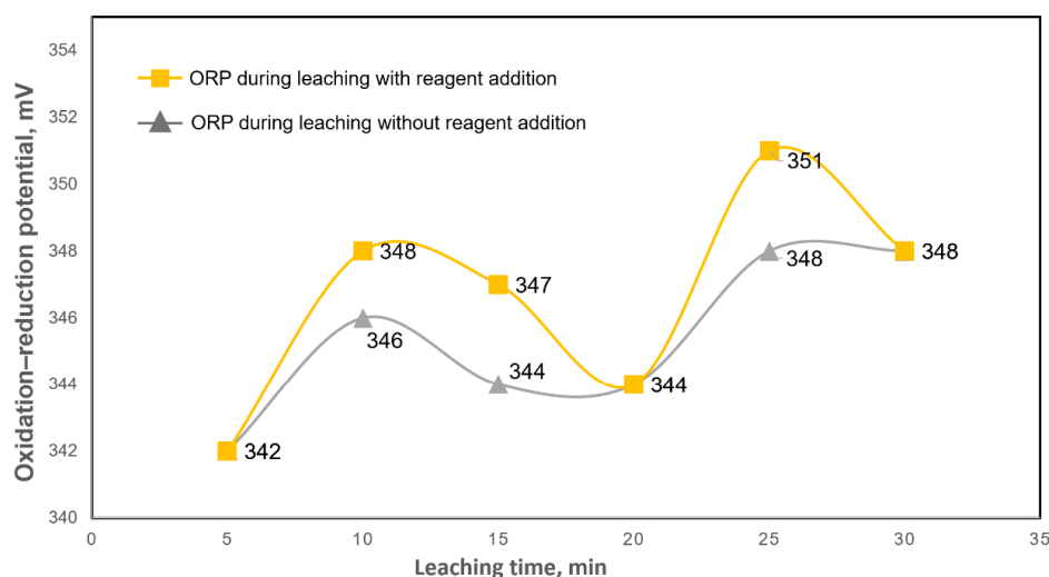
Figure 7. Dependences of oxidation–reduction potential (ORP) on leaching time.
