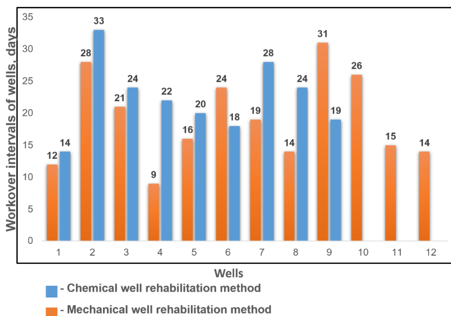
Figure 2. Workover intervals of 12 wells after mechanical and chemical well rehabilitation methods.
