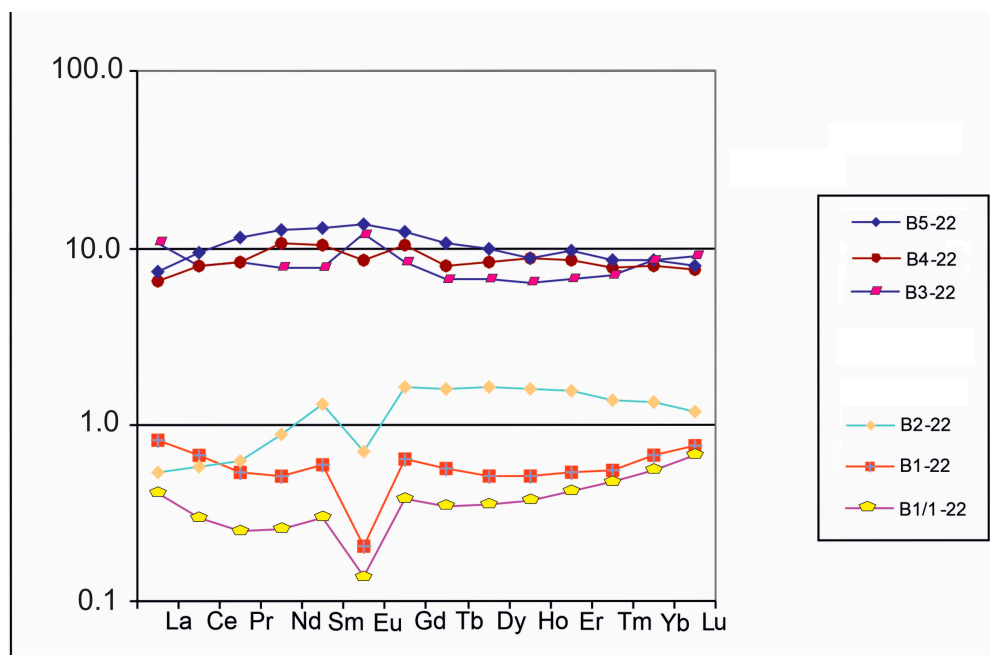
Figure 8. Normalized spectra of rare earth element contents of nephrite B1, B1/1, and B2 and metagabbro B3, B4, and B5.
