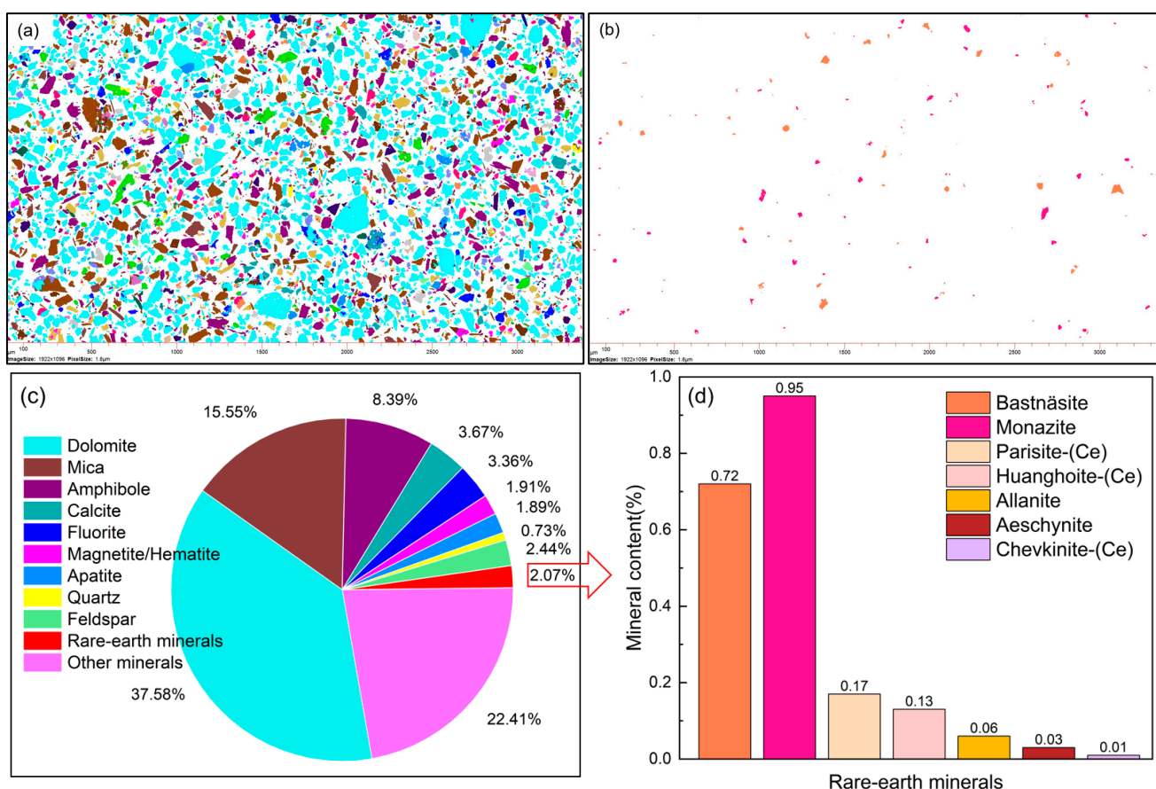
Figure 2. Mineralogical characterization of the West Mine iron beneficiation tailings: (a) AMICS mineral map of all phases; (b) AMICS rare-earth mineral map; (c) major mineral composition; and (d) rare-earth mineral composition.
