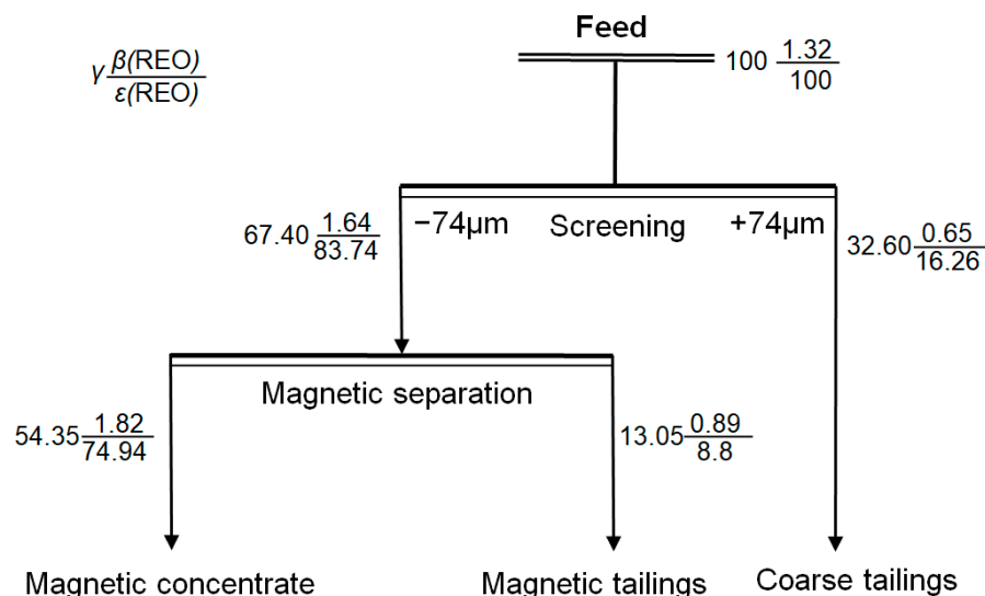
Figure 7. Mass and metallurgical balance for the combined screening and magnetic separation tests.
