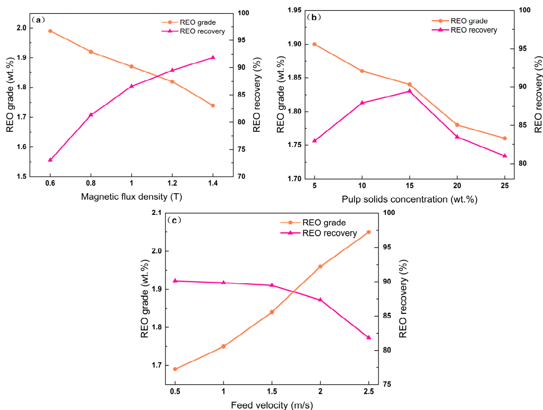
Figure 6. Effects of magnetic separation conditions on the REO grade and recovery of the concentrate: (a) magnetic flux density; (b) pulp solids concentration; and (c) feed velocity.
