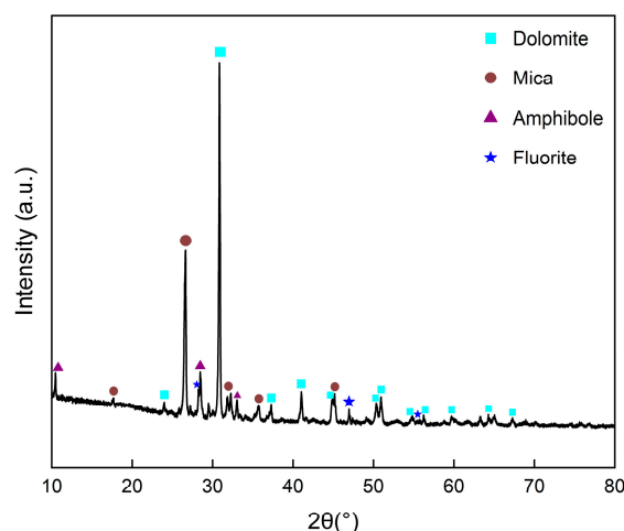
Figure 1. XRD pattern of the Bayan Obo West Mine iron beneficiation tailings.
