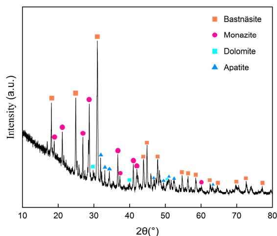
Figure 11. XRD pattern of the rare-earth concentrate.
