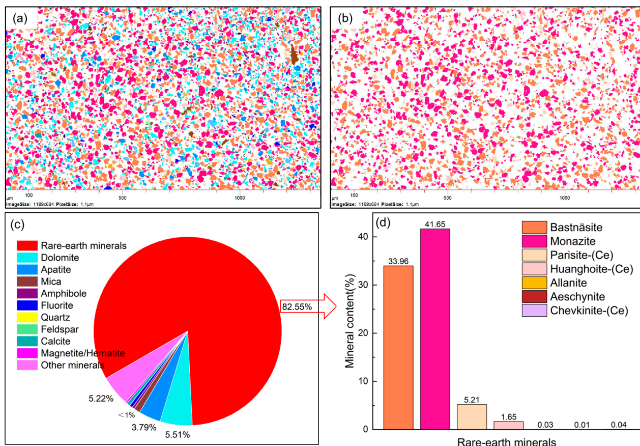
Figure 12. Mineralogical characterization of the closed-circuit rare-earth flotation concentrate: (a) AMICS mineral map of all phases; (b) AMICS rare-earth mineral map; (c) major mineral composition; and (d) rare-earth mineral composition.
