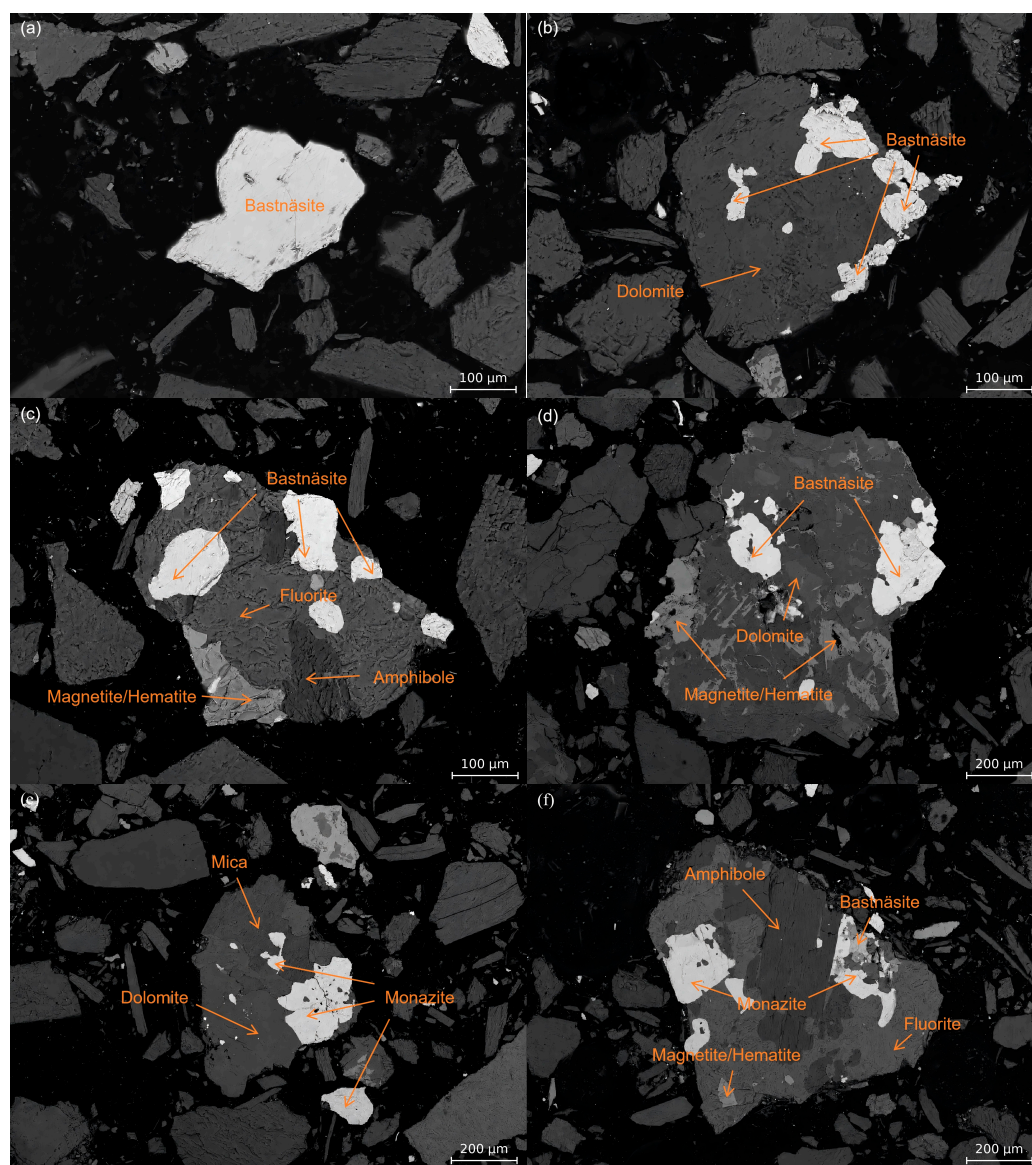
Figure 4. Representative dissemination and intergrowth characteristics of bastnäsite and monazite: (a) liberated bastnäsite; (b) bastnäsite disseminated along the margins of dolomite; (c) bastnäsite intergrown with dolomite and amphibole; (d) bastnäsite intergrown with dolomite and magnetite/hematite; (e) monazite intergrown with dolomite and mica; and (f) monazite and bastnäsite intergrown with amphibole, fluorite, and magnetite/hematite.
