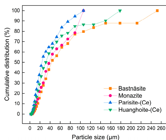
Figure 3. Cumulative particle size distributions of the principal rare-earth minerals.
