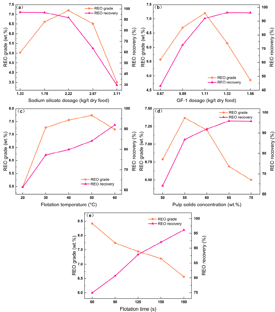
Figure 8. Effects of rougher flotation conditions on the REO grade and recovery of the concentrate: (a) sodium silicate dosage; (b) GF-1 dosage; (c) flotation temperature; (d) pulp solids concentration; and (e) flotation time.
