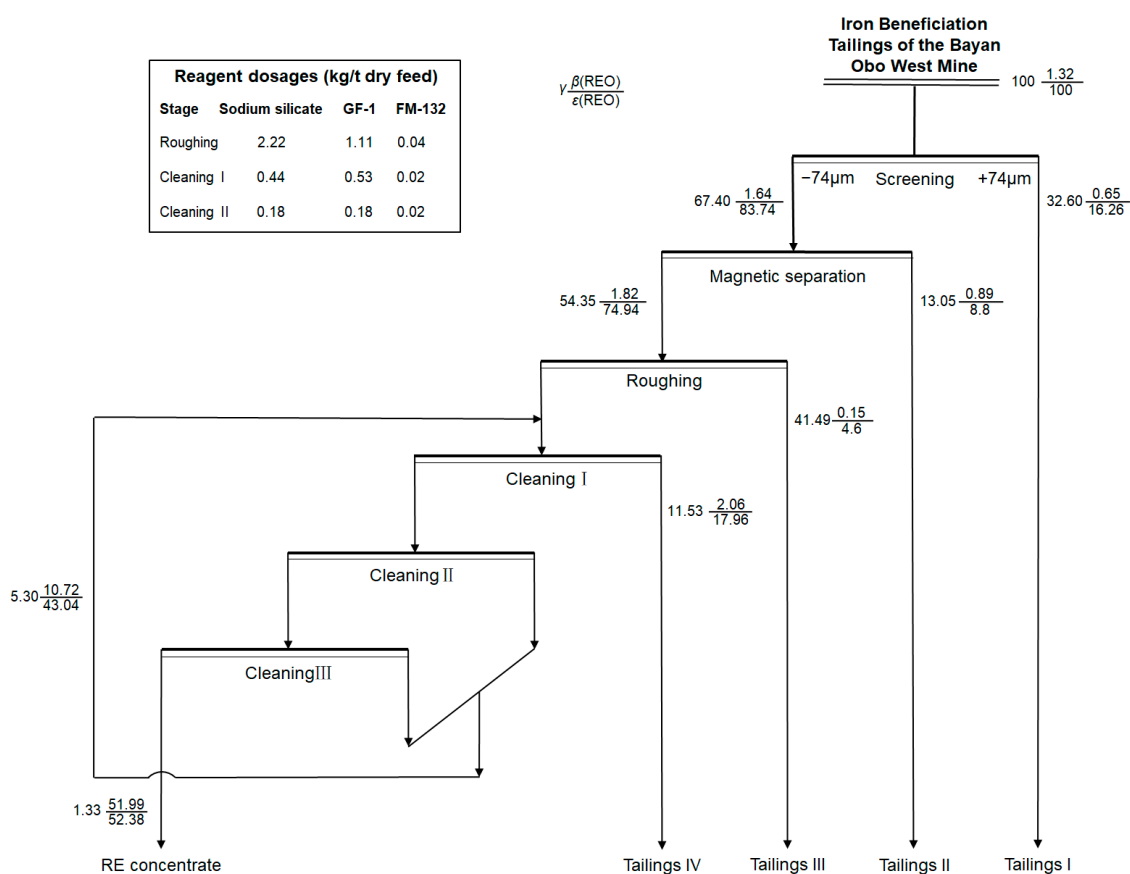
Figure 10. Mass and metallurgical balance for the overall flowsheet comprising screening, magnetic separation, and closed-circuit flotation with one rougher and three cleaner stages for the West Mine iron beneficiation tailings.
