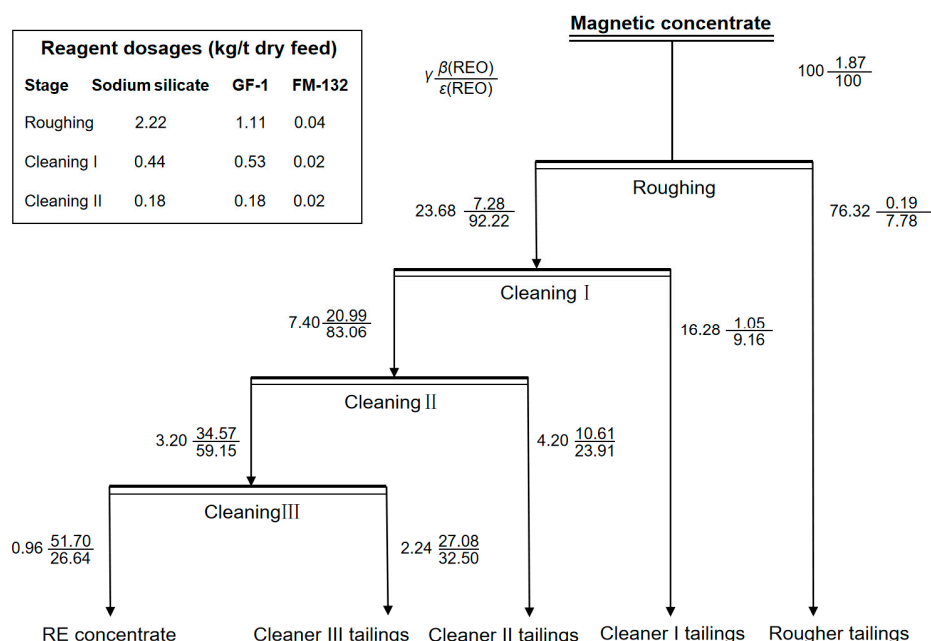
Figure 9. Mass and metallurgical balance for the open-circuit rare-earth flotation test.
