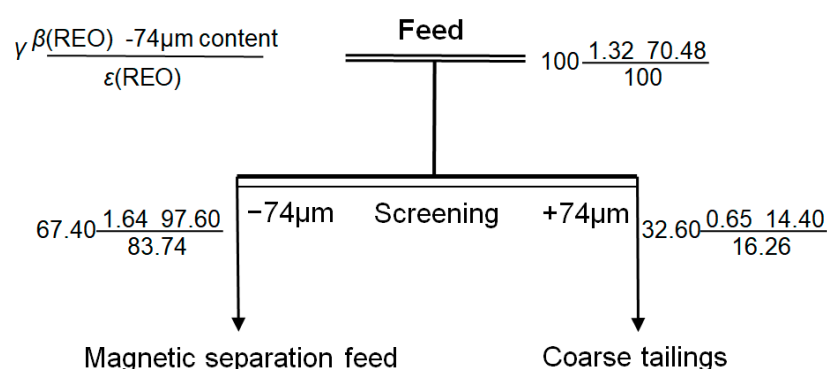
Figure 5. Mass and metallurgical balance for the 74 \mu\text{m} screening test. Here, \gamma denotes mass yield (%), \beta(\text{REO}) denotes REO grade (wt.%), \epsilon(\text{REO}) denotes REO recovery (%), and the final value shown for each stream denotes the -74 \mu\text{m} content (%).
