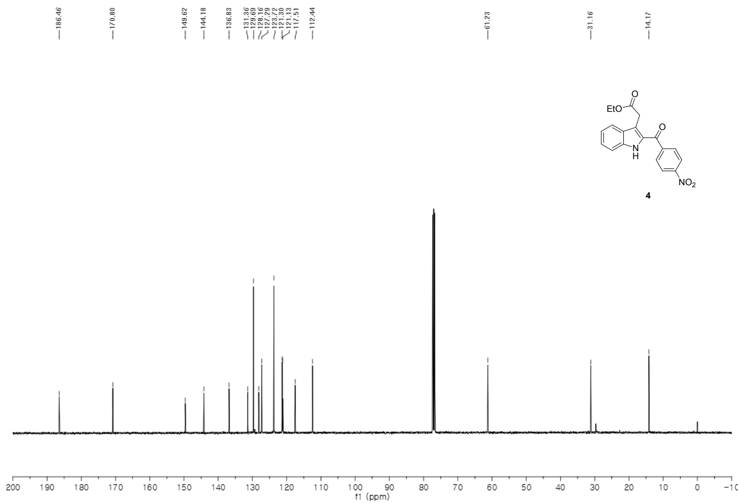
Figure S2. ^{13}\text{C} NMR spectrum of 4 ( \text{CDCl}_3 , 100 MHz)
