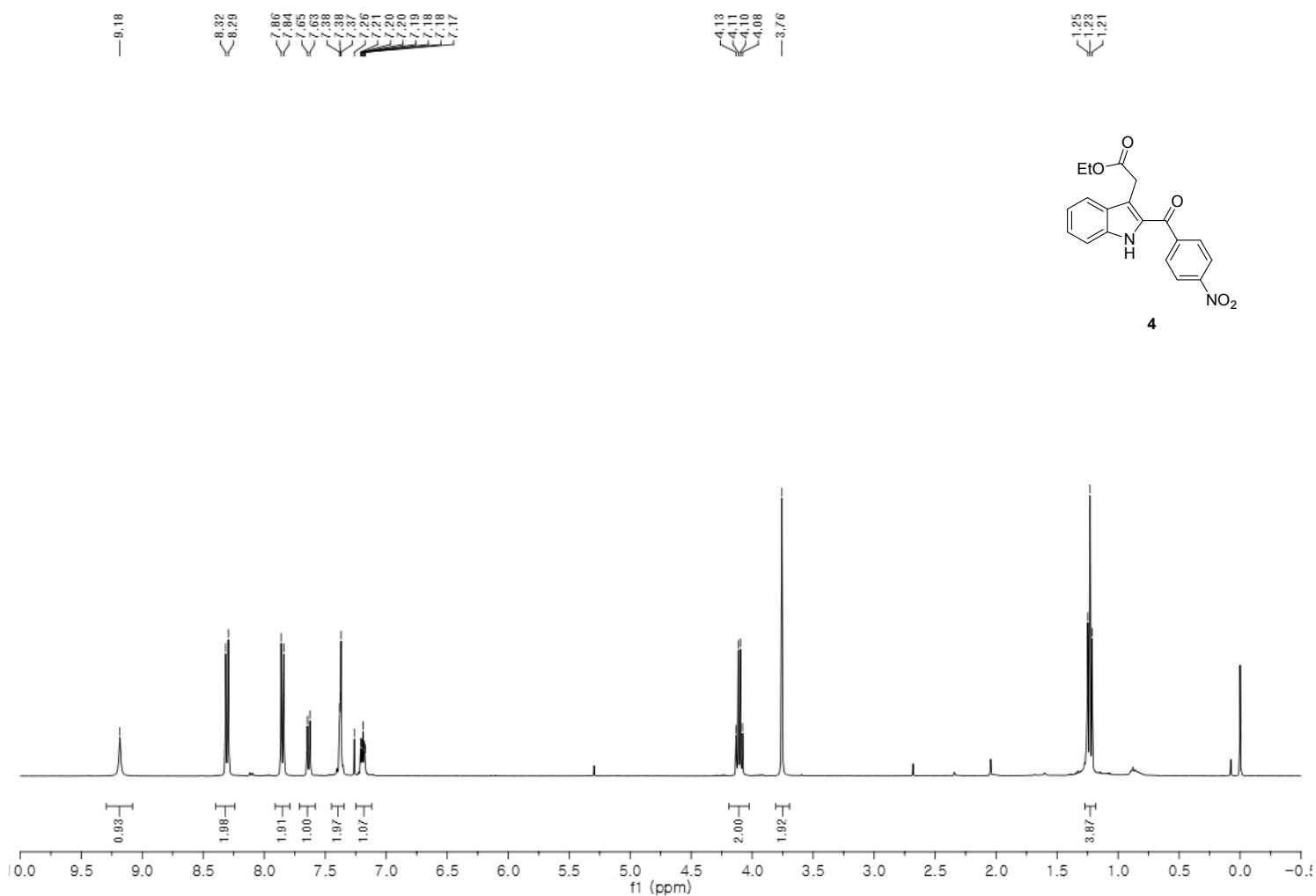
Figure S1. 1 H NMR spectrum of 4 (CDCl 3 , 400 MHz)
