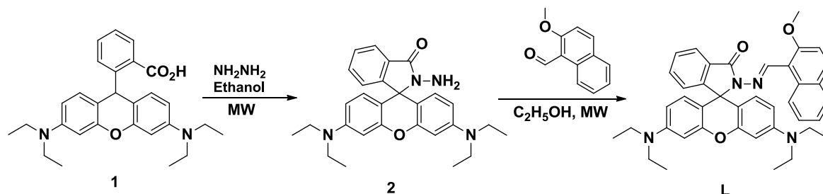
Scheme 1. Synthesis of ( E )-3',6'-bis(diethylamine)-2-[(2-methoxynaphthalen-1-yl)methyleneamino]spiro[isindoline-1,9'-xanthen]-3-one ( L ).
