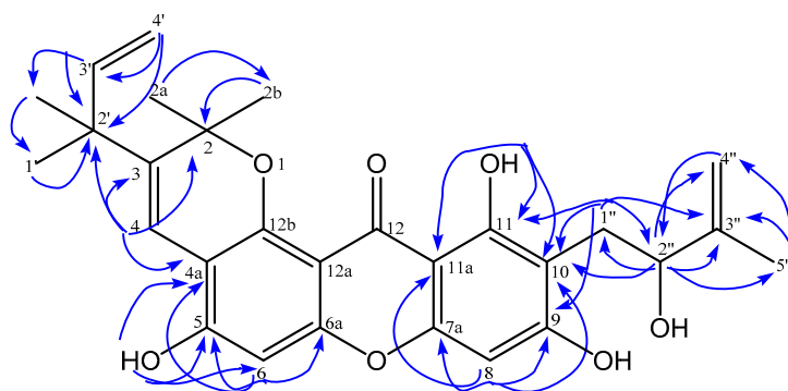
Figure 2. Selected HMBC correlation for 5,9,11-trihydroxy-10-(2''-hydroxy-3''-methylbut-3''-en-1-yl)-2,2-dimethyl-3-(2'-methylbut-3'-en-2'-yl)-2H,12H-pyrano[2,3-a]xanthen-12-one.
