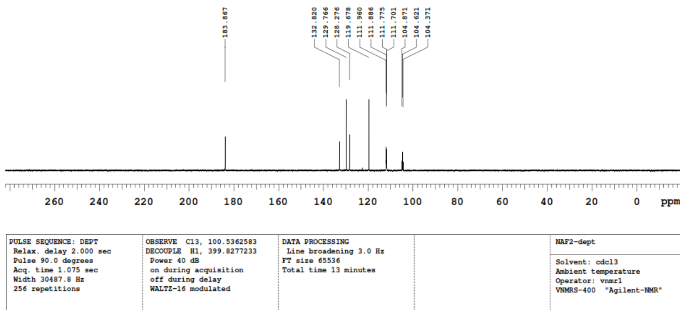
Figure S8. ^{13}\text{C} NMR DEPT Spectra of 3-(3,5-difluorophenyl)-1-phenyl-1 H -pyrazole-4-carboxaldehyde (2)
