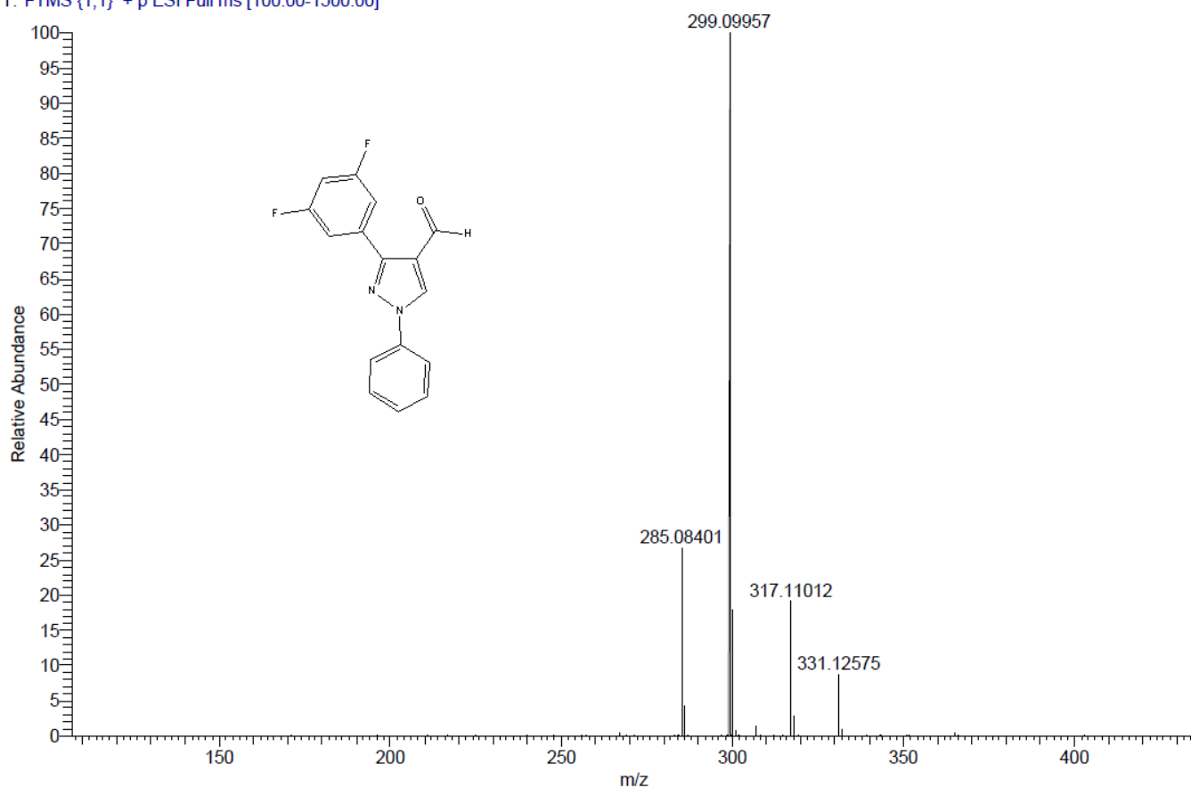
Figure S1. High Resolution Mass Spectra (HRMS) of 3-(3,5-difluorophenyl)-1-phenyl-1H-pyrazole-4-carboxalehyde ( 2 )
