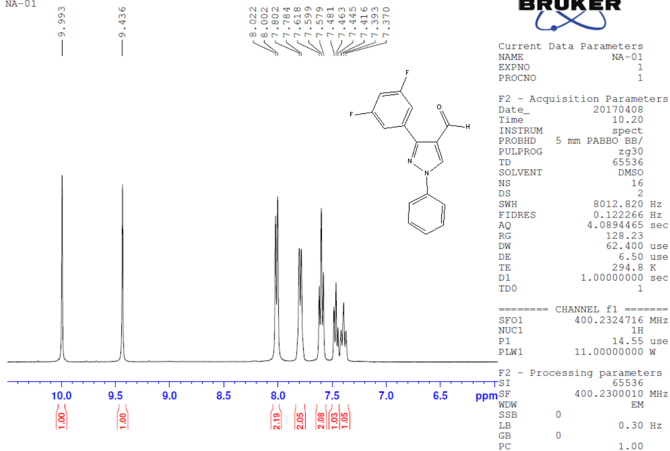
Figure S4. Expanded ^1\text{H} NMR spectra of 3-(3,5-difluorophenyl)-1-phenyl-1 H -pyrazole-4-carboxaldehyde (2)
