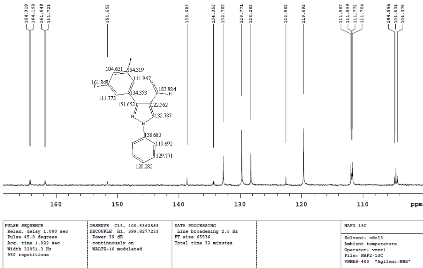
Figure S7. Expanded ^{13}\text{C} NMR spectra of 3-(3,5-difluorophenyl)-1-phenyl-1 H -pyrazole-4-carboxaldehyde (2)
