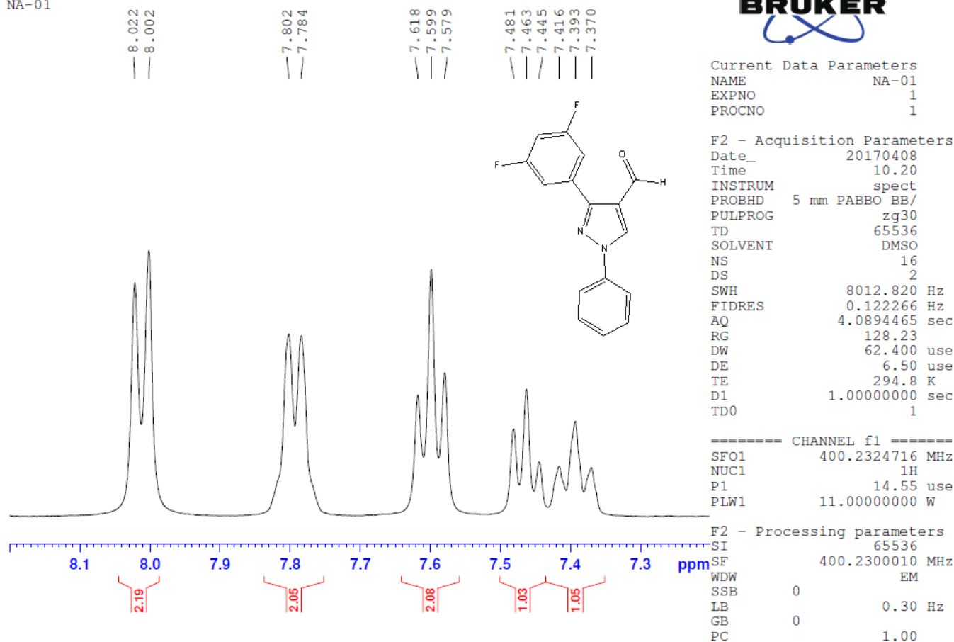
Figure S5. Expanded ^1\text{H} NMR spectra of 3-(3,5-difluorophenyl)-1-phenyl-1 H -pyrazole-4-carboxaldehyde (2)
