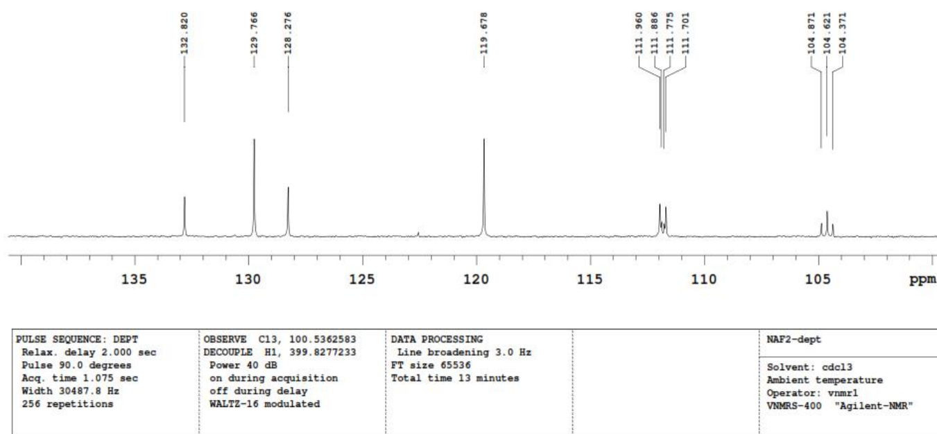
Figure S9. Expanded ^{13}\text{C} NMR DEPT Spectra of 3-(3,5-difluorophenyl)-1-phenyl-1 H -pyrazole-4-carboxaldehyde ( 2 )
