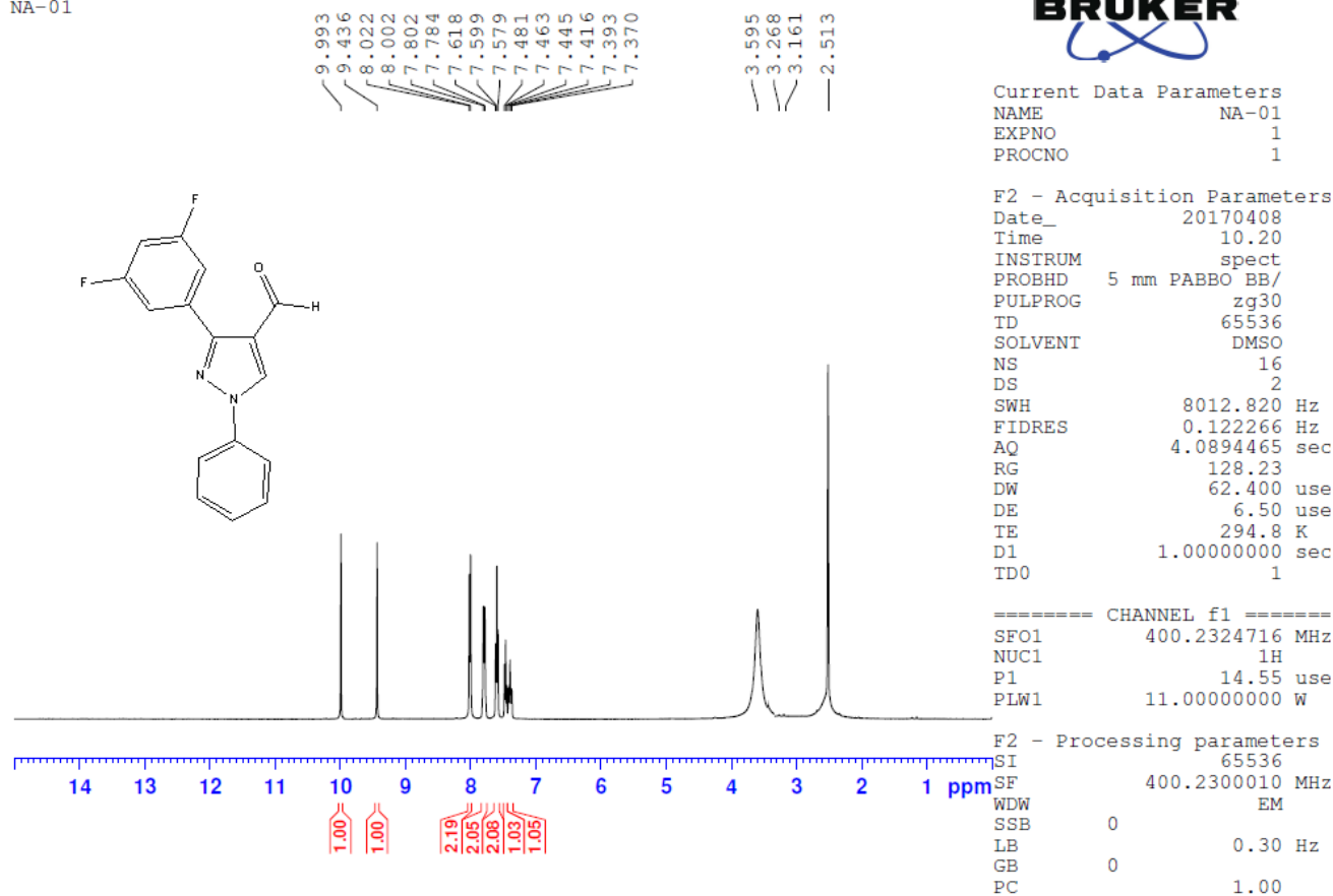
Figure S3. ^1\text{H} NMR of 3-(3,5-difluorophenyl)-1-phenyl-1 H -pyrazole-4-carboxaldehyde (2)
