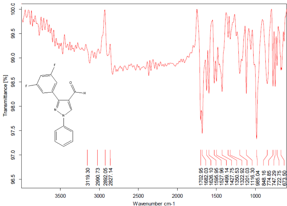
Figure S2. FT-IR Spectra of 3-(3,5-difluorophenyl)-1-phenyl-1H-pyrazole-4-carboxalehyde ( 2 )
