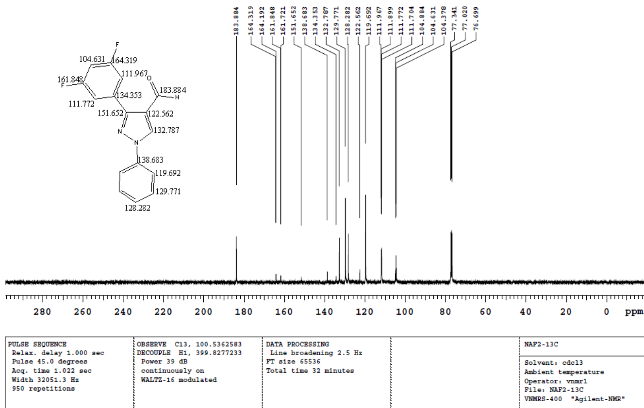
Figure S6. ^{13}\text{C} NMR spectra of 3-(3,5-difluorophenyl)-1-phenyl-1 H -pyrazole-4-carboxaldehyde (2)
