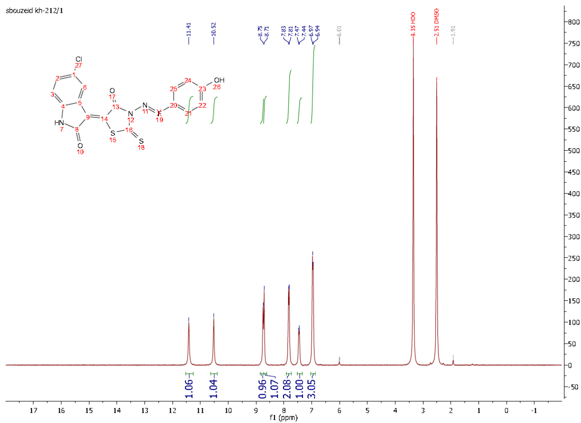
Figure S1. 1 H-NMR of compound 4.
