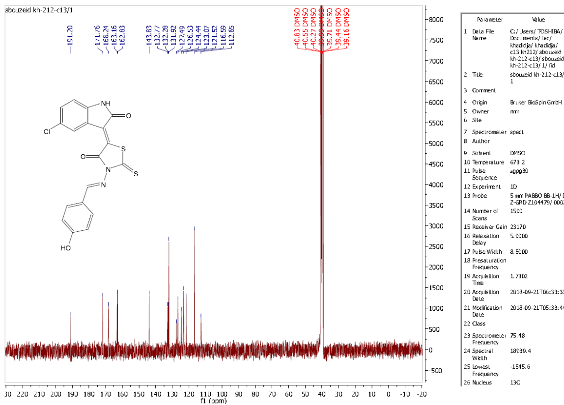
Figure S2. 13 C-NMR of compound 4.
