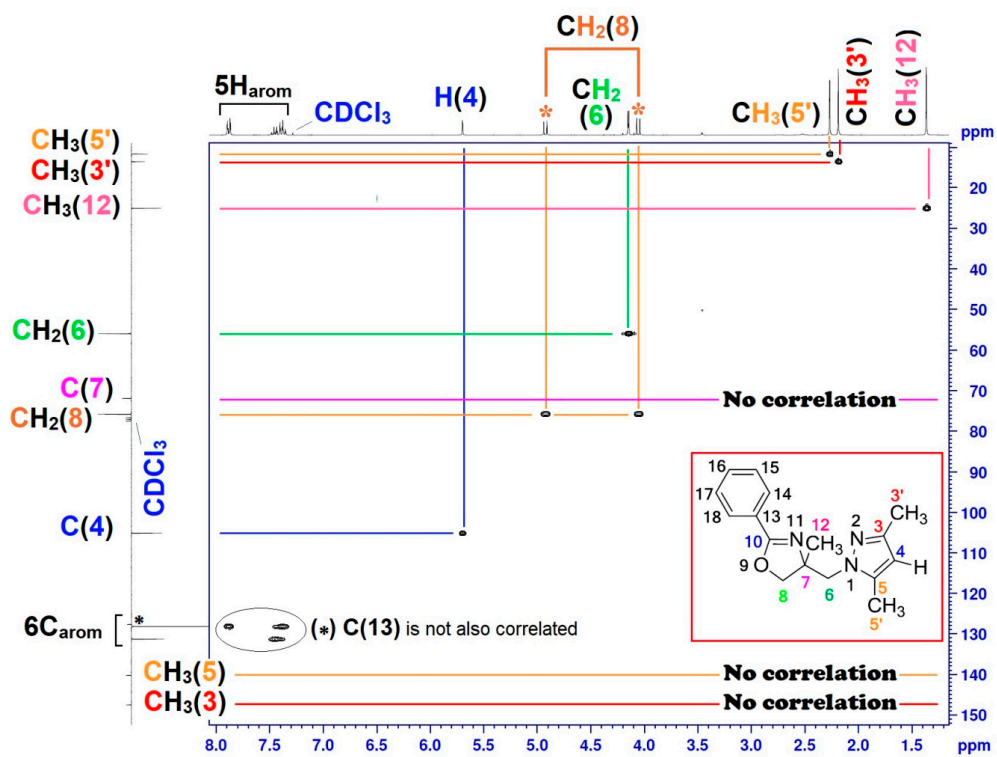
Figure 2. ^1\text{H} - ^{13}\text{C} 2D correlation spectroscopy identifies coupling between protons and carbons in compound 2.
