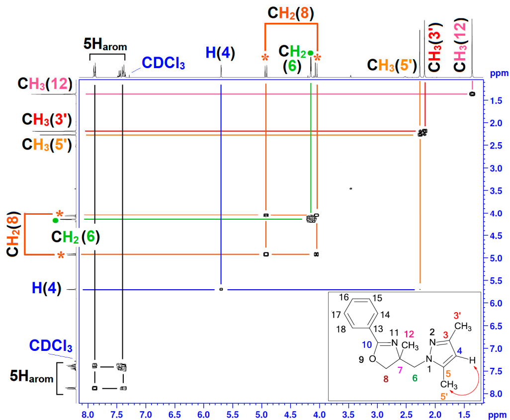
Figure 1. ^1\text{H} - ^1\text{H} correlation spectroscopy identifies coupling between protons in compound 2.
