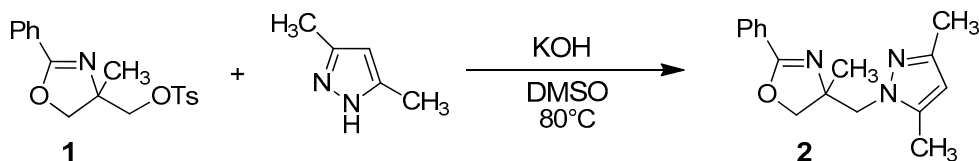
Scheme 1. Synthesis strategy for compound 2 .
