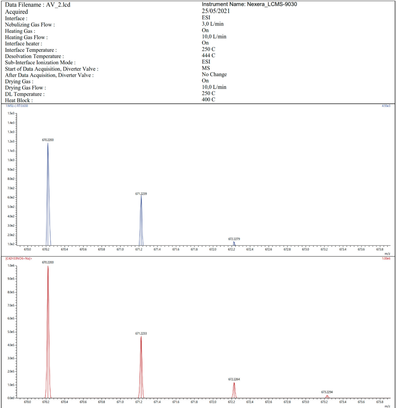
Figure 3. ESI-HRMS spectrum of 1.
