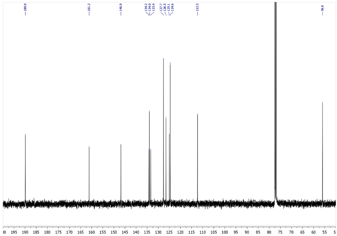
Figure 2. 13 C NMR spectrum of 1, CDCl 3 , 100 MHz.
