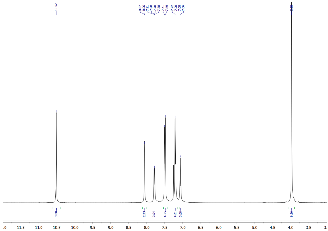
Figure 1. 1 H NMR spectrum of 1, CDCl 3 , 400 MHz.
