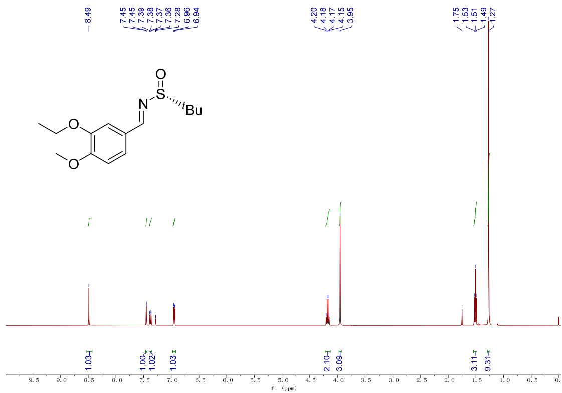
Figure S1: 1 H-NMR of (R,E) - N -(3-ethoxy-4-methoxybenzylidene)-2-methylpropane-2-sulfonamide ( 8 )
