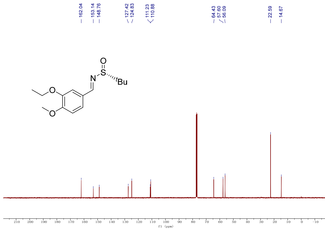
Figure S2: 13 C-NMR of (R,E) - N -(3-ethoxy-4-methoxybenzylidene)-2-methylpropane-2-sulfonamide ( 8 )
