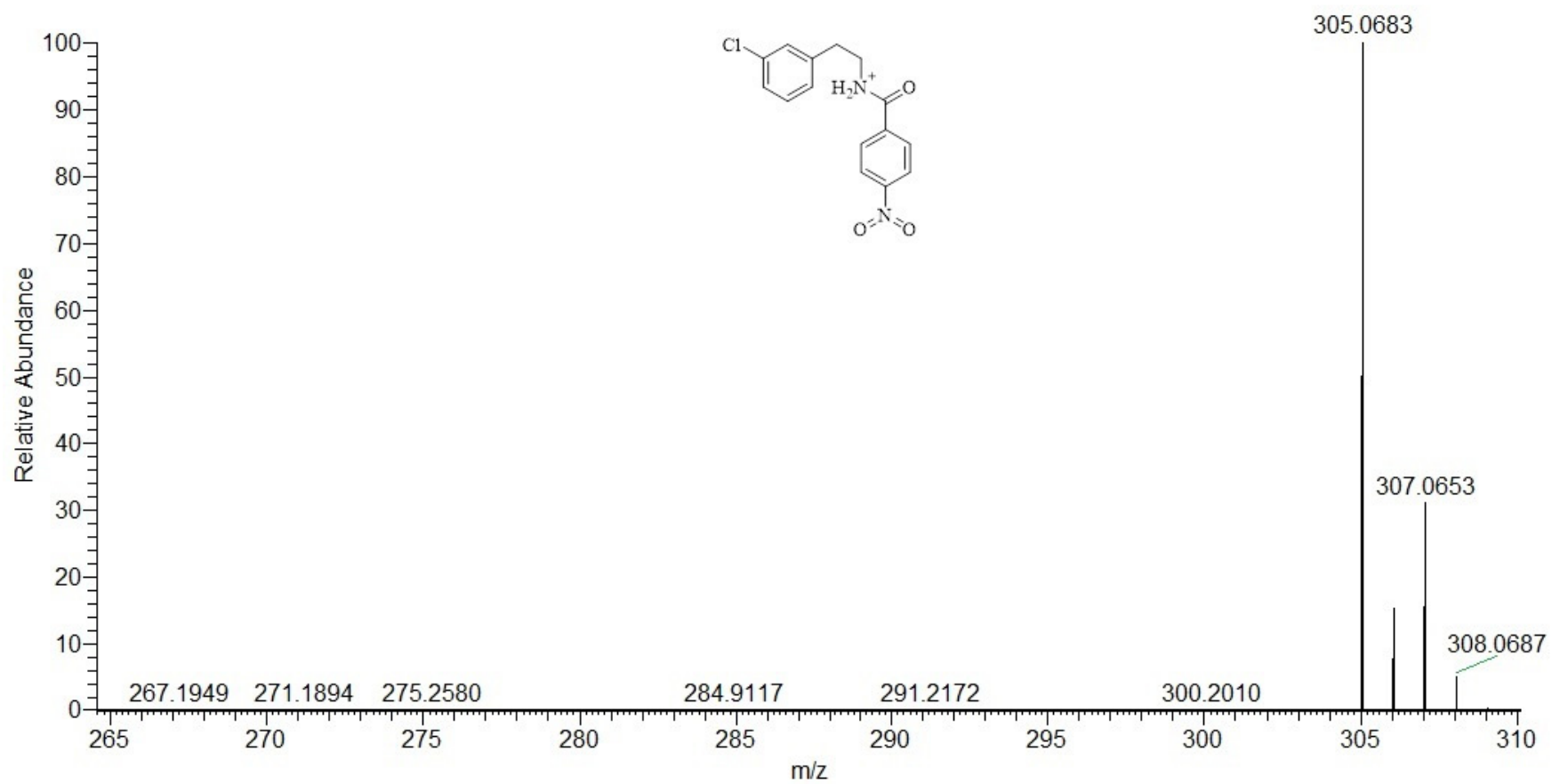
Figure S4. ESI-HRMS of compound 3.
