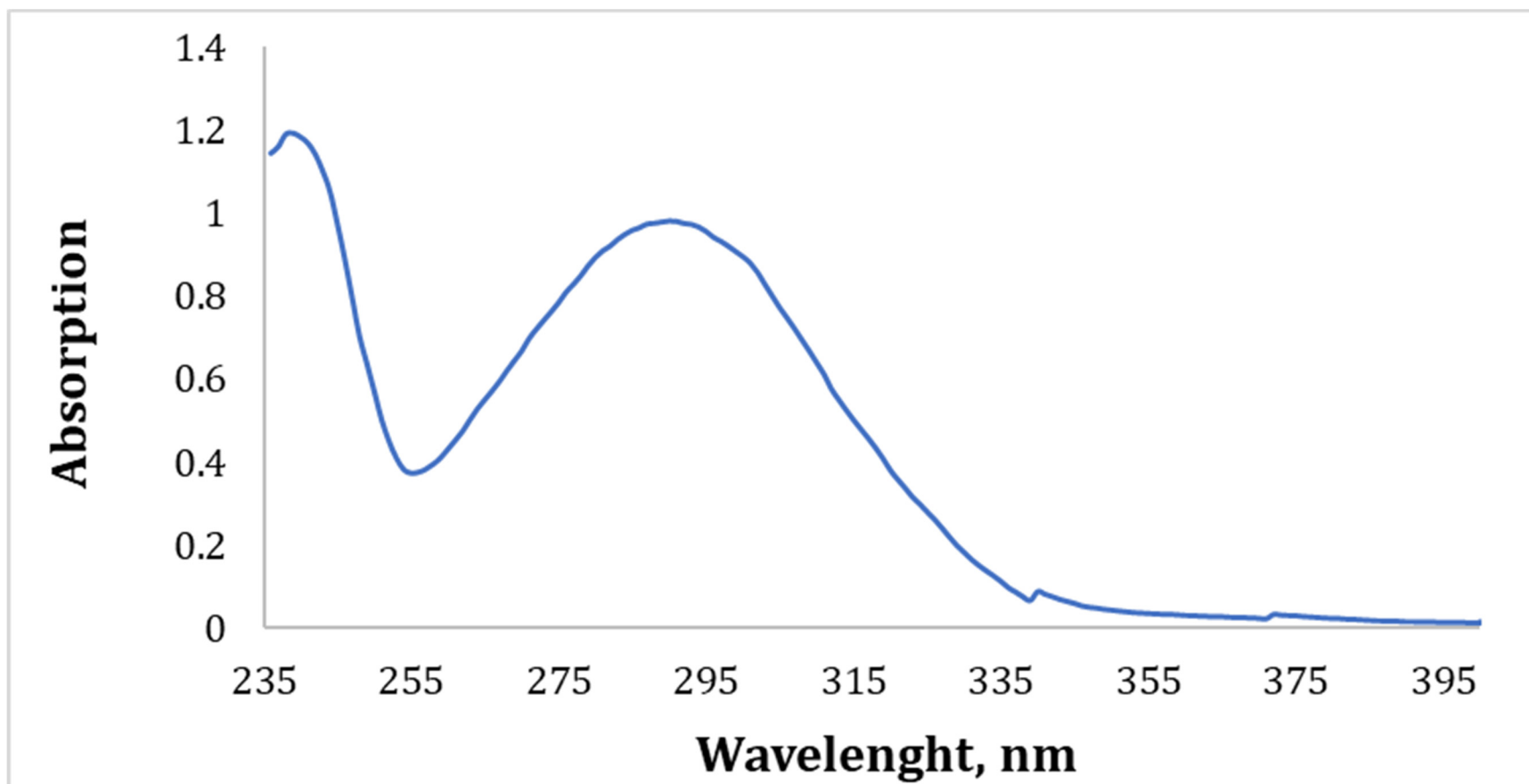
Figure S3. UV spectrum of compound 3.
