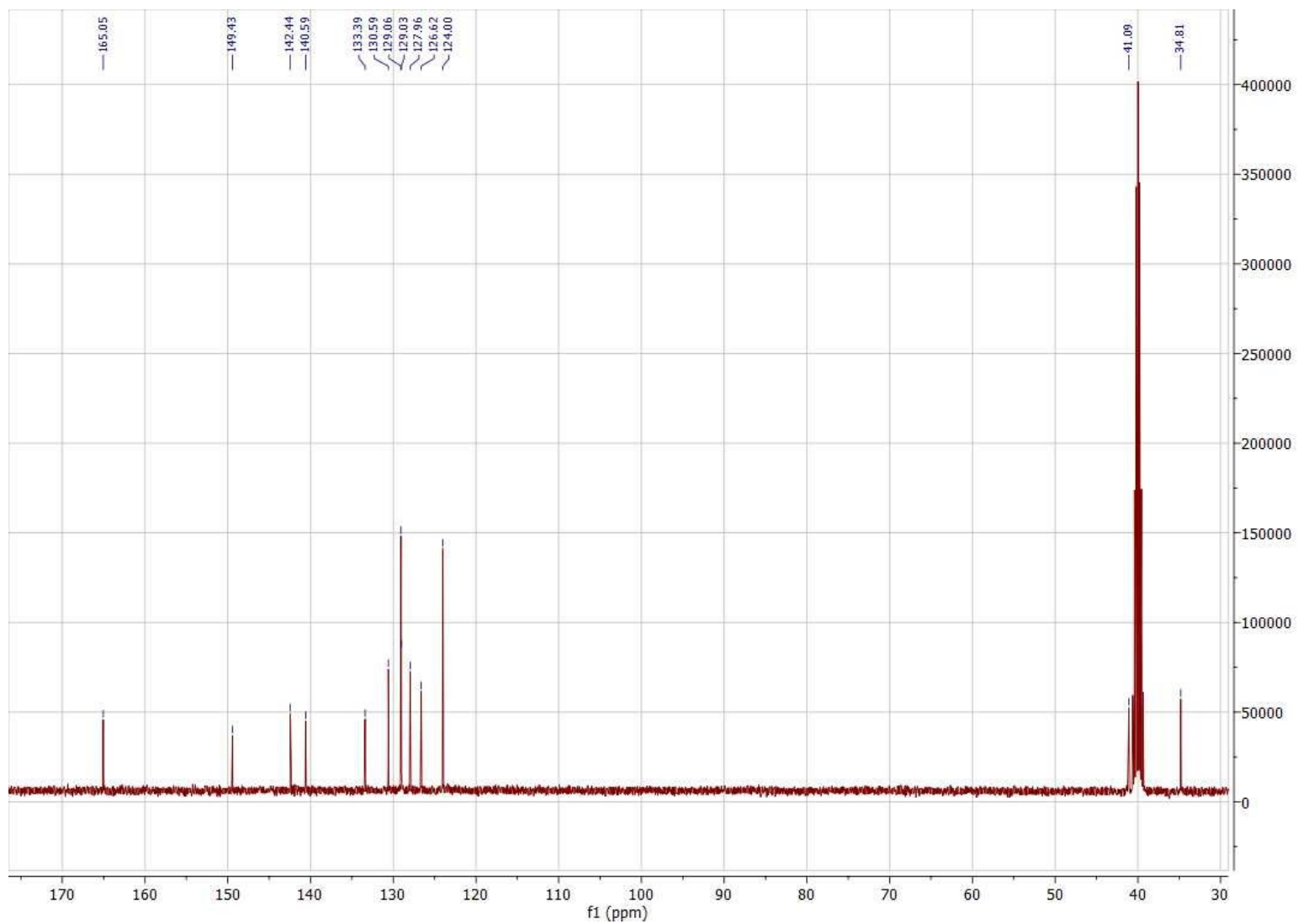
Figure S2. ^{13}\text{C} -NMR spectrum of compound 3.
