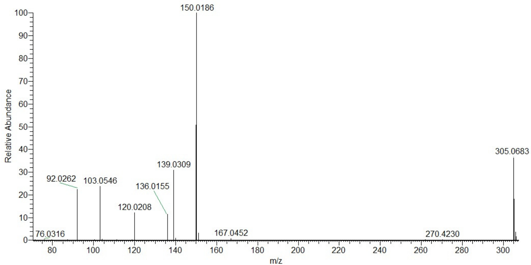
Figure S5. Mass spectrum of compound 3 obtained by positive ion ESI-MS/MS.
