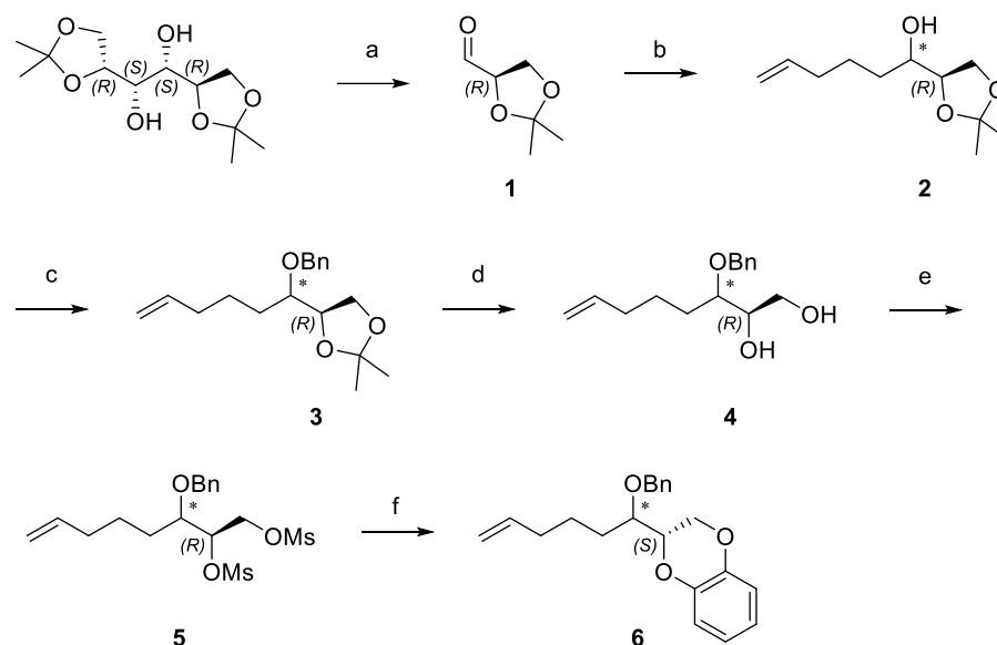
Scheme 1. Synthesis of 2-(1-benzyloxy-hex-5-enyl)-2,3-dihydro-1,4-benzodioxine ( 6 ). Reagents and conditions: (a) NaHCO 3 sat., NaIO 4 , DCM, RT; (b) Mg, I 2 , 5-bromopentene, THF, reflux; (c) NaH, BnBr, THF, RT; (d) HCl 10%, MeOH, RT; (e) TEA, MsCl, DCM, RT; (f) K 2 CO 3 , catechol, DMF, RT.
