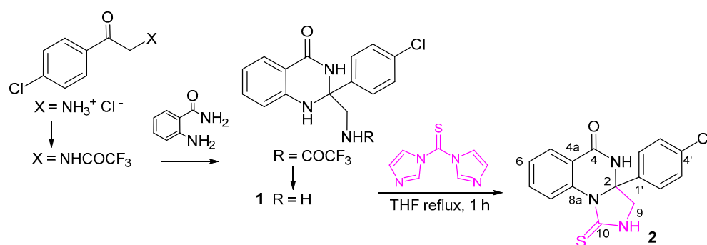
Scheme 1. Synthesis of the target compound 2 from 1 ; arbitrary numbering is for convenience, used for NMR assignments.
