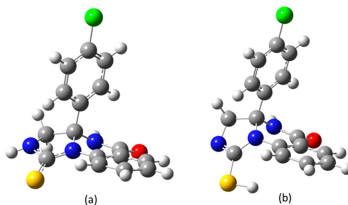
Figure 1. Energy minimized structures of (a) thioamide and (b) iminethiol forms of compound 2.
