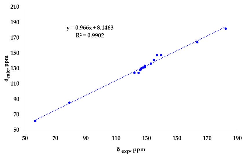
Figure 2. Correlation plot of calculated vs. experimental ^{13}\text{C} NMR chemical shifts for the thioamide form of compound 2.
