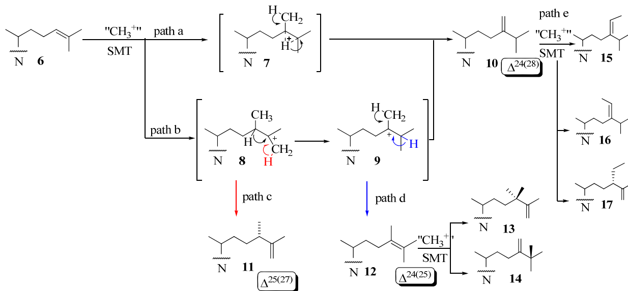
Figure 3. Various C-24-alkylation pathways.
