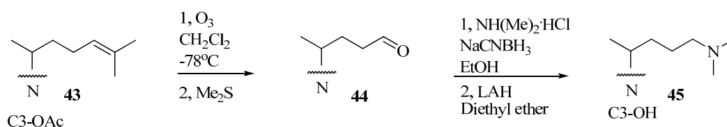
Figure 5. Preparative route to 25-azalanosterol A45 .
