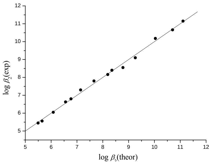
Figure 6. Experimental vs. theoretical (fit) \log \beta_2 for \text{Mn}^{2+} , \text{Fe}^{2+} , \text{Co}^{2+} , and \text{Ni}^{2+} complexes with glycine, alanine, valine and leucine; r = 0.998 , \text{S.E.}_{\text{cv}} = 0.15 .
