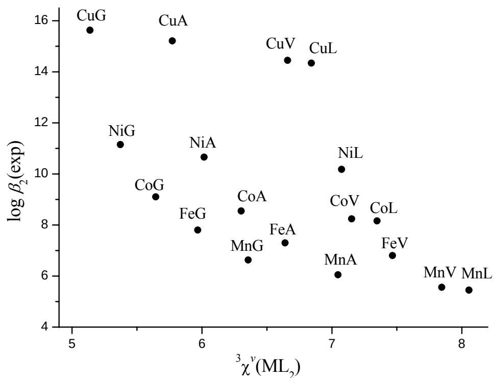
Figure 3. Experimental values of \log \beta_2 vs. connectivity {}^3\chi^v index for \text{Mn}^{2+} , \text{Fe}^{2+} , \text{Co}^{2+} , \text{Ni}^{2+} , and \text{Cu}^{2+} complexes with glycine (G), alanine (A), valine (V) and leucine (L).
