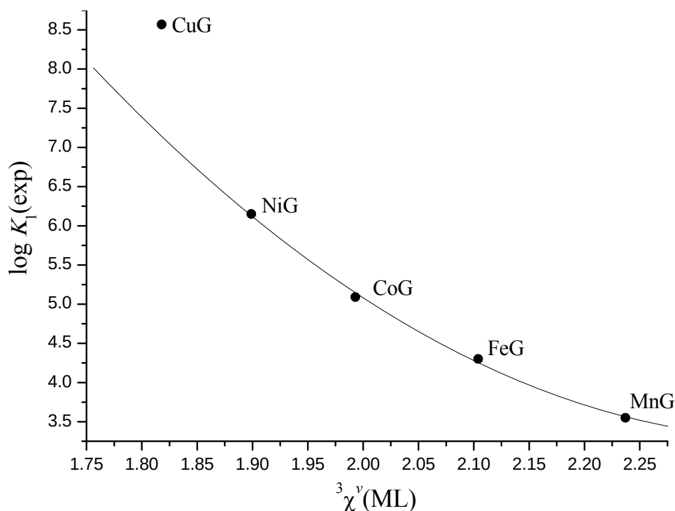
Figure 4. Quadratic dependence of \log K_1 of \text{Mn}^{2+} , \text{Fe}^{2+} , \text{Co}^{2+} , and \text{Ni}^{2+} complexes with glycine (G) on connectivity index {}^3\chi^v .
