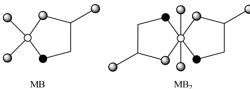
Figure 1. The graph representations for metal(II) mono - (MB) and bis -complex (MB 2 ) with glycine. Heteroatoms are marked with ○ (M), ● (N), and ◐ (O).
