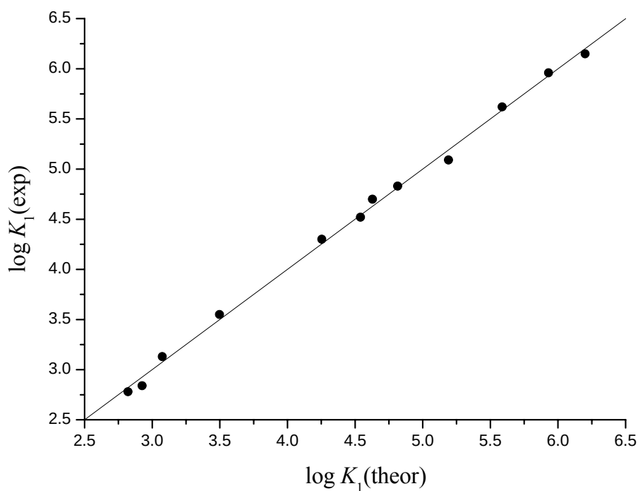
Figure 5. Experimental vs. theoretical (fit) \log K_1 for \text{Mn}^{2+} , \text{Fe}^{2+} , \text{Co}^{2+} , and \text{Ni}^{2+} complexes with glycine, alanine, valine and leucine; r = 0.999 , \text{S.E.}_{\text{cv}} = 0.08 .
