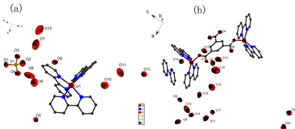
Figure 1. (a) The coordination environments of Co atoms with 50% thermal ellipsoids of complex 1 . (b) The coordination environments of Cu atoms with 50% thermal ellipsoids of complex 2 .
