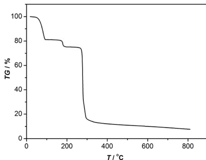
Figure 7. The TG-DTG curve of complex 2.
