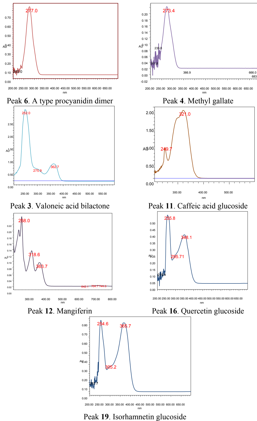
Figure 5. PDA spectra of compounds 3 , 4 , 6 , 11 , 12 , 16 and 19 .
